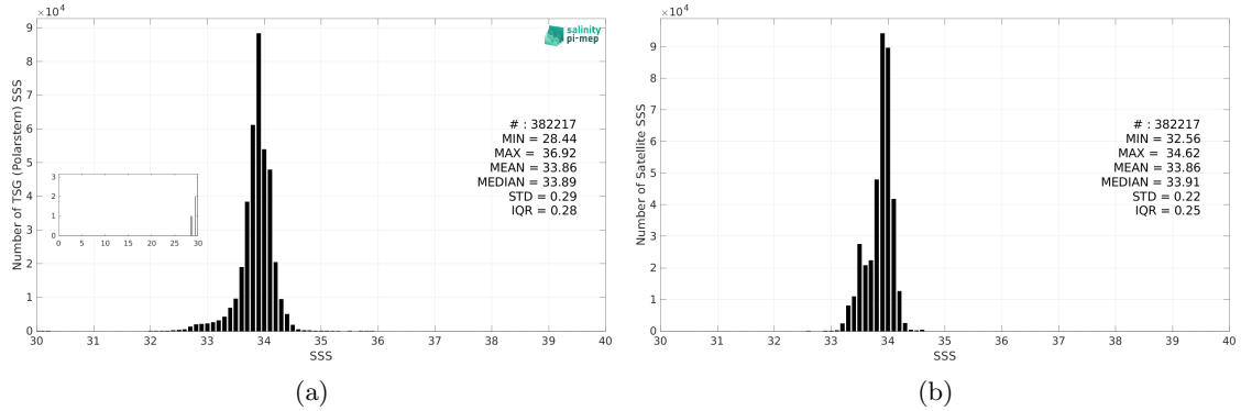
Figure 3: Histograms of SSS from TSG (Polarstern) (a) and SMOS SSS L4 v1 - Monthly (CMEMS-CNR) (b) considering all match-up pairs per bins of 0.1 over the Southern Ocean Pi-MEP region and for the full satellite product period.
