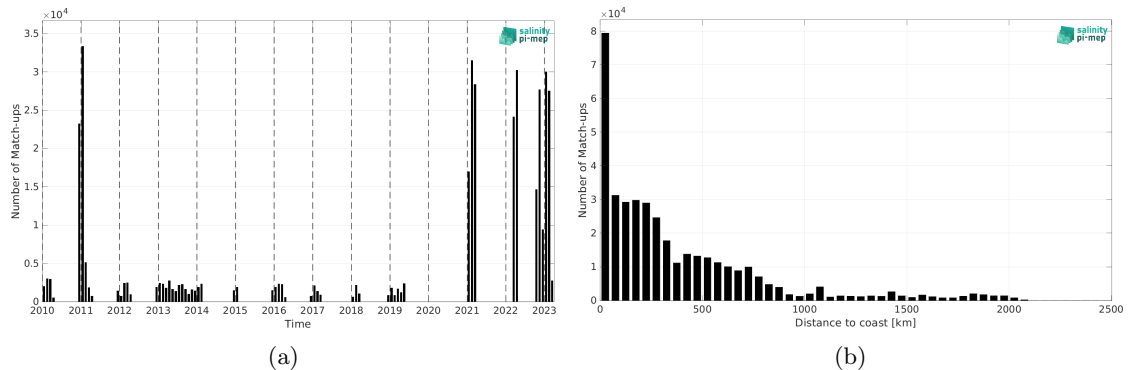
Figure 2: Number of match-ups between TSG (Polarstern) and SMOS SSS L4 v1 - Monthly (CMEMS-CNR) SSS as a function of time (a) and as function of the distance to coast (b) over the Southern Ocean Pi-MEP region and for the full satellite product period.
