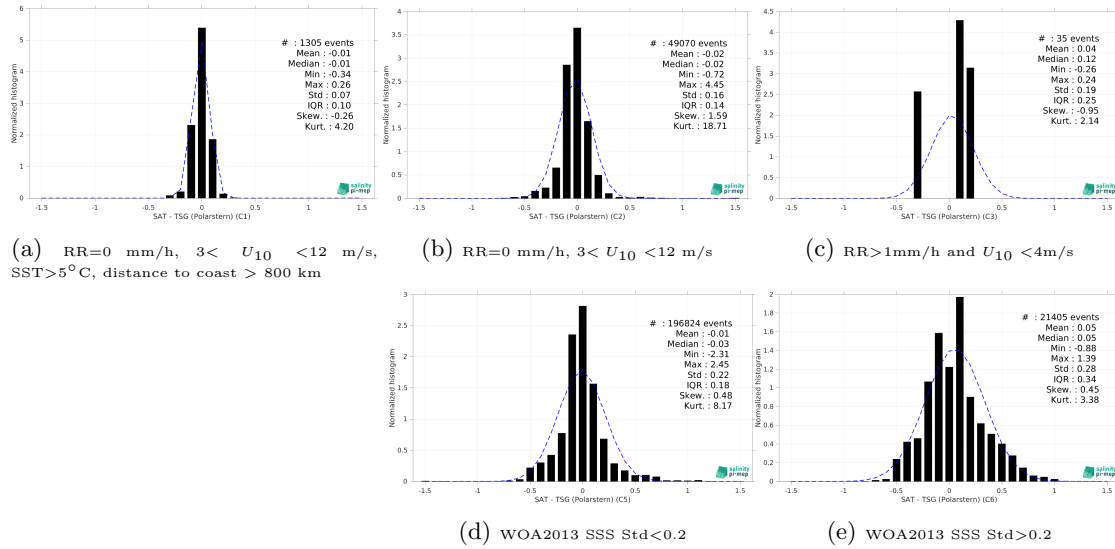
Figure 13: Normalized histogram of \Delta\text{SSS} (SMOS SSS L4 v1 - Monthly (CMEMS-CNR) - TSG (Polarstern)) for 5 different subdatasets corresponding to: RR=0 mm/h, 3 < U_{10} < 12 m/s, SST>5°C, distance to coast > 800 km (a), RR=0 mm/h, 3 < U_{10} < 12 m/s (b), RR>1mm/h and U_{10} < 4 m/s (c), WOA2013 SSS Std<0.2 (d), WOA2013 SSS Std>0.2 (e).
