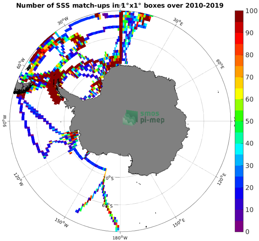
Figure 4: Number of SSS match-ups between TSG (Polarstern) SSS and the SMOS SSS L4 v1 - Monthly (CMEMS-CNR) SSS product for the Southern Ocean Pi-MEP region over 1^\circ \times 1^\circ boxes and for the full satellite product period.
