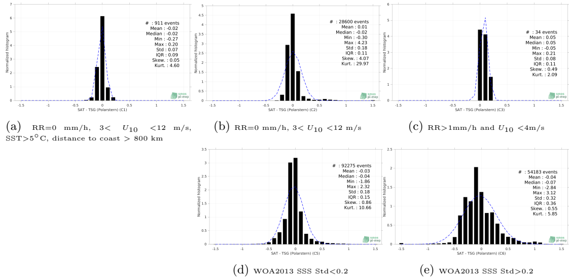
Figure 13: Normalized histogram of \Delta SSS (SMOS SSS L4 v1 - Monthly (CMEMS-CNR) - TSG (Polarstern)) for 5 different subdatasets corresponding to: RR=0 mm/h, 3 < U_{10} < 12 m/s, SST > 5°C, distance to coast > 800 km (a), RR=0 mm/h, 3 < U_{10} < 12 m/s (b), RR > 1mm/h and U_{10} < 4 m/s (c), WOA2013 SSS Std < 0.2 (d), WOA2013 SSS Std > 0.2 (e).
