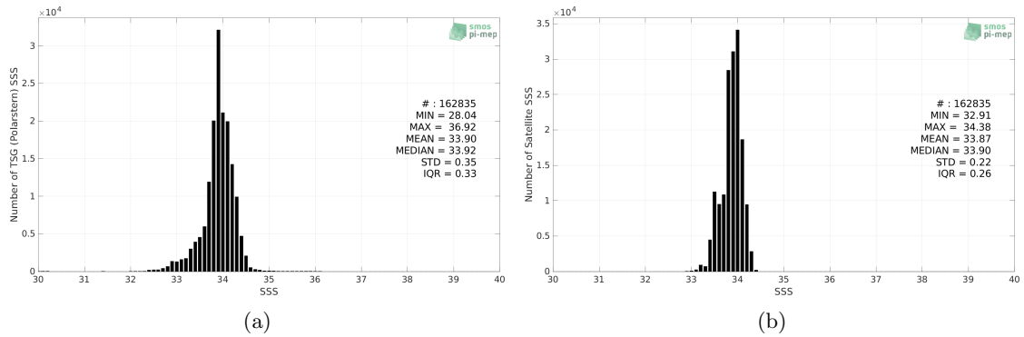
Figure 2: Histograms of SSS from TSG (Polarstern) (a) and SMOS SSS L4 v1 - Monthly (CMEMS-CNR) (b) considering all match-up pairs per bins of 0.1 over the Southern Ocean Pi-MEP region and for the full satellite product period.
