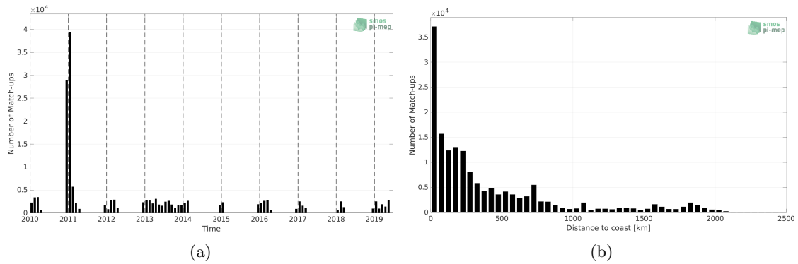
Figure 1: Number of match-ups between TSG (Polarstern) and SMOS SSS L4 v1 - Monthly (CMEMS-CNR) SSS as a function of time (a) and as function of the distance to coast (b) over the Southern Ocean Pi-MEP region and for the full satellite product period.
