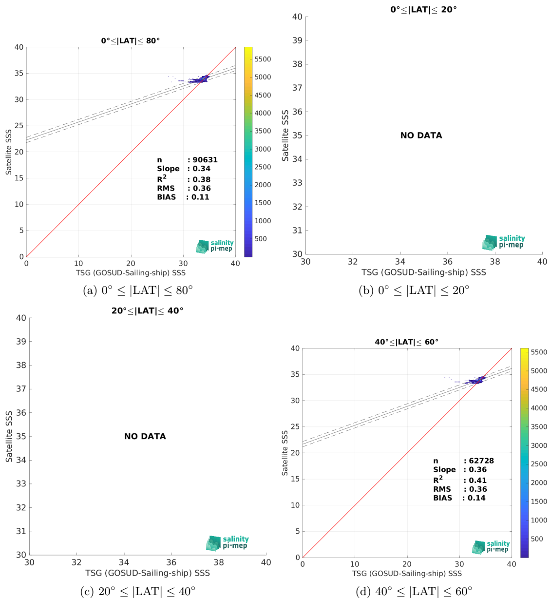
Figure 10: Contour maps of the concentration of SMOS SSS L4 v1 - Monthly (CMEMS-CNR) SSS (y-axis) versus TSG (GOSUD-Sailing-ship) SSS (x-axis) at match-up pairs for different latitude bands. For each plot, the red line shows x=y . The black thin and dashed lines indicate a linear fit through the data cloud and the \pm 95\% confidence levels, respectively. The number match-up pairs n , the slope and R^2 coefficient of the linear fit, the root mean square (RMS) and the mean bias between satellite and in situ data are indicated for each latitude band in each plots.
