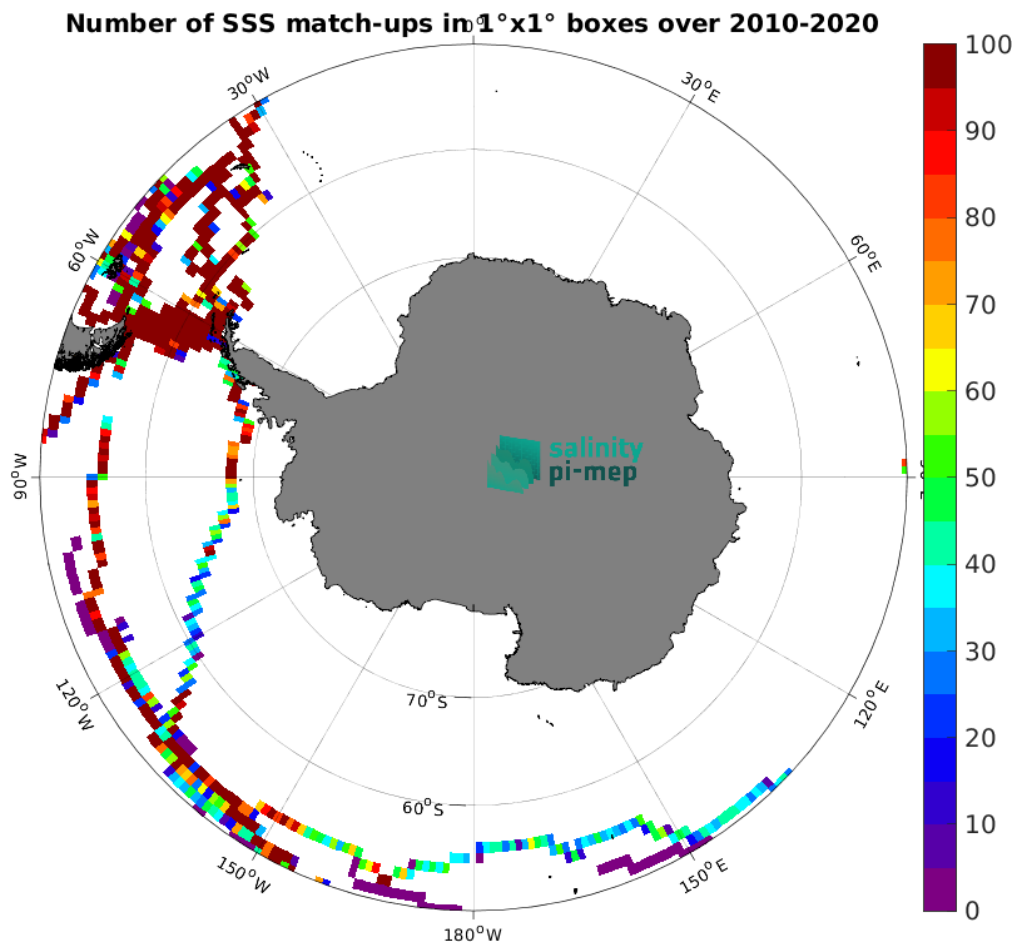
Figure 5: Number of SSS match-ups between TSG (GOSUD-Sailing-ship) SSS and the SMOS SSS L4 v1 - Monthly (CMEMS-CNR) SSS product for the Southern Ocean Pi-MEP region over 1^\circ \times 1^\circ boxes and for the full satellite product period.
