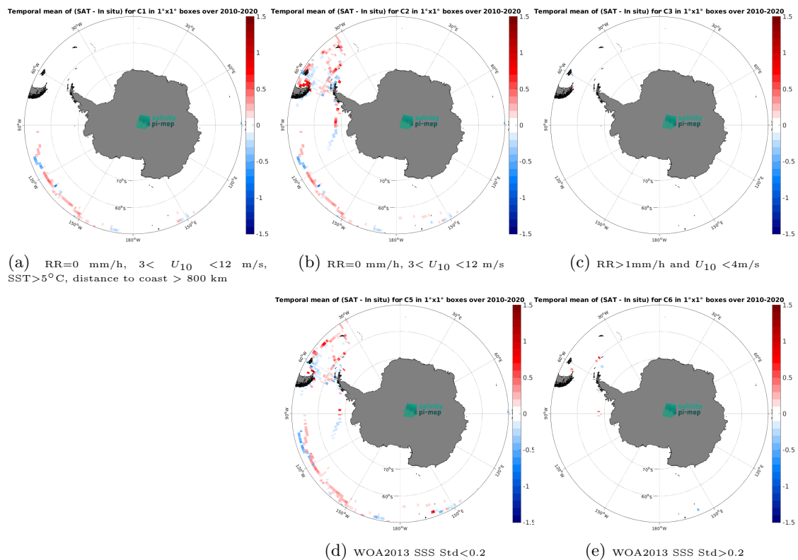
Figure 14: Temporal mean gridded over spatial boxes of size 1^\circ \times 1^\circ of \Delta SSS (SMOS SSS L4 v1 - Monthly (CMEMS-CNR) - TSG (GOSUD-Sailing-ship)) for 5 different subdatasets corresponding to:RR=0 mm/h, 3 < U_{10} < 12 m/s, SST > 5^\circ\text{C} , distance to coast > 800 km (a), RR=0 mm/h, 3 < U_{10} < 12 m/s (b), RR > 1 mm/h and U_{10} < 4 m/s (c), WOA2013 SSS Std < 0.2 (d), WOA2013 SSS Std > 0.2 (e).
