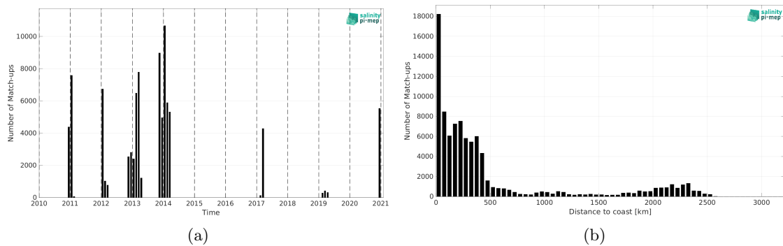
Figure 2: Number of match-ups between TSG (GOSUD-Sailing-ship) and SMOS SSS L4 v1 - Monthly (CMEMS-CNR) SSS as a function of time (a) and as function of the distance to coast (b) over the Southern Ocean Pi-MEP region and for the full satellite product period.
