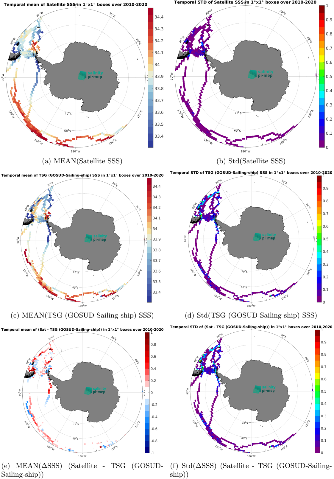
Figure 7: Temporal mean (left) and Std (right) of SSS from SMOS SSS L4 v1 - Monthly (CMEMS-CNR) (top), TSG (GOSUD-Sailing-ship) (middle), and of \Delta SSS (Satellite - TSG (GOSUD-Sailing-ship)). Only match-up pairs are used to generate these maps.
