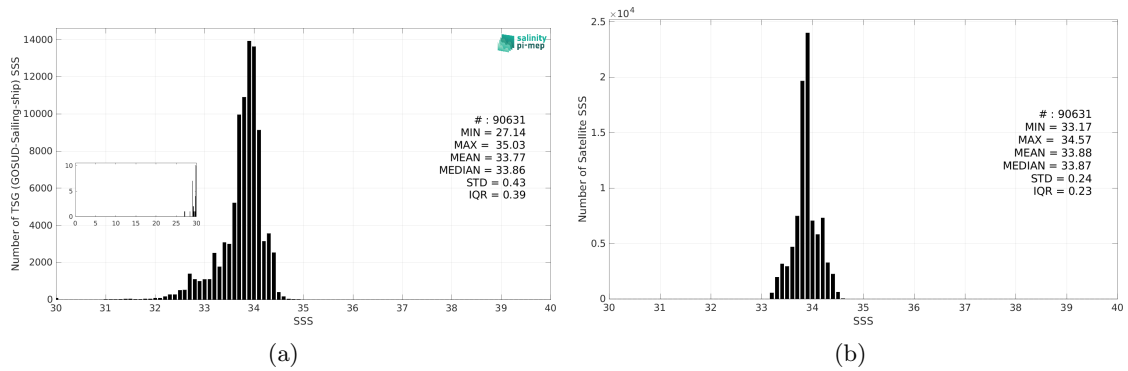
Figure 3: Histograms of SSS from TSG (GOSUD-Sailing-ship) (a) and SMOS SSS L4 v1 - Monthly (CMEMS-CNR) (b) considering all match-up pairs per bins of 0.1 over the Southern Ocean Pi-MEP region and for the full satellite product period.
