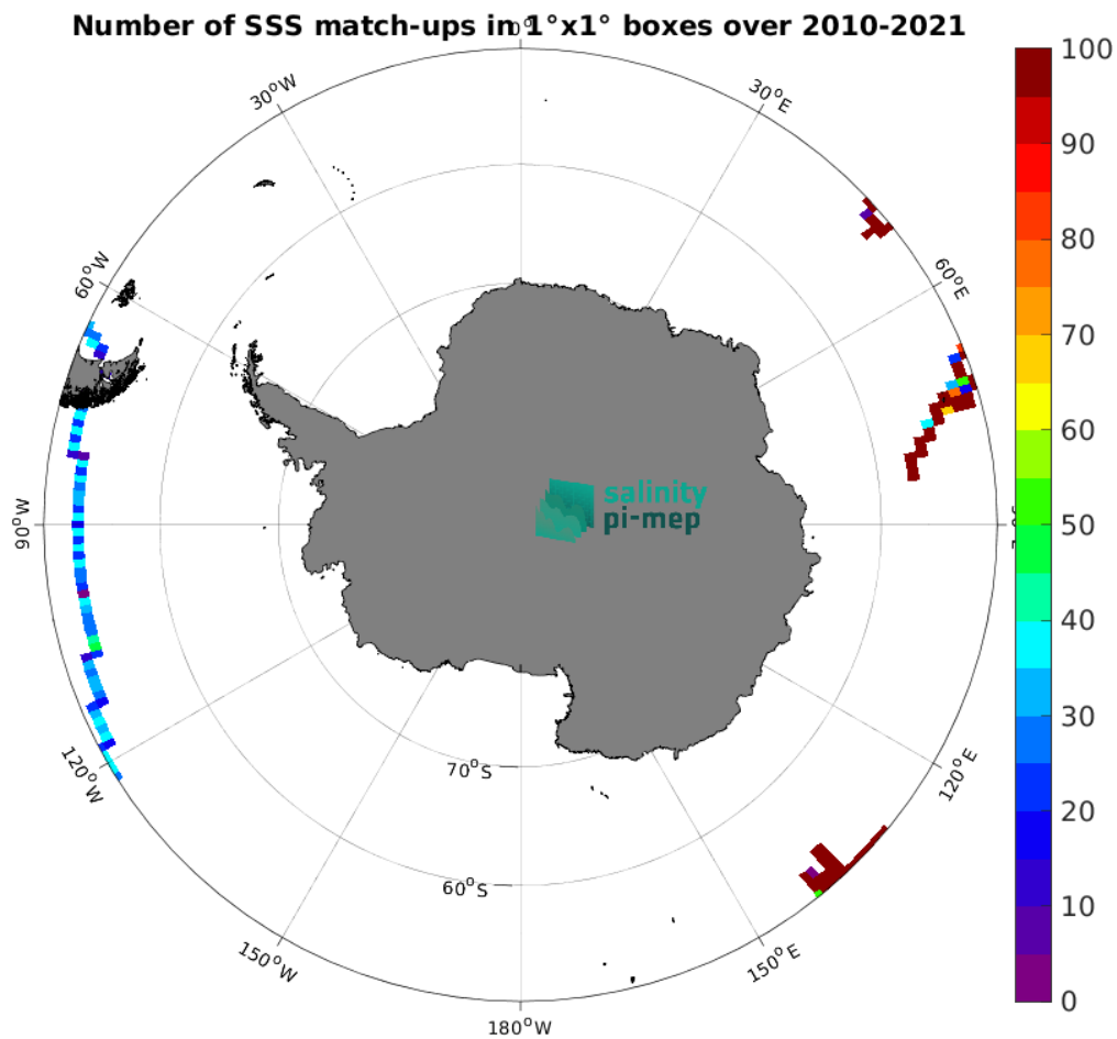
Figure 5: Number of SSS match-ups between TSG (GOSUD-Research-vessel) SSS and the SMOS SSS L4 v1 - Monthly (CMEMS-CNR) SSS product for the Southern Ocean Pi-MEP region over 1^\circ \times 1^\circ boxes and for the full satellite product period.
