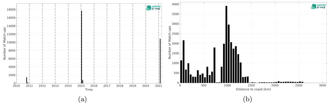
Figure 2: Number of match-ups between TSG (GOSUD-Research-vessel) and SMOS SSS L4 v1 - Monthly (CMEMS-CNR) SSS as a function of time (a) and as function of the distance to coast (b) over the Southern Ocean Pi-MEP region and for the full satellite product period.
