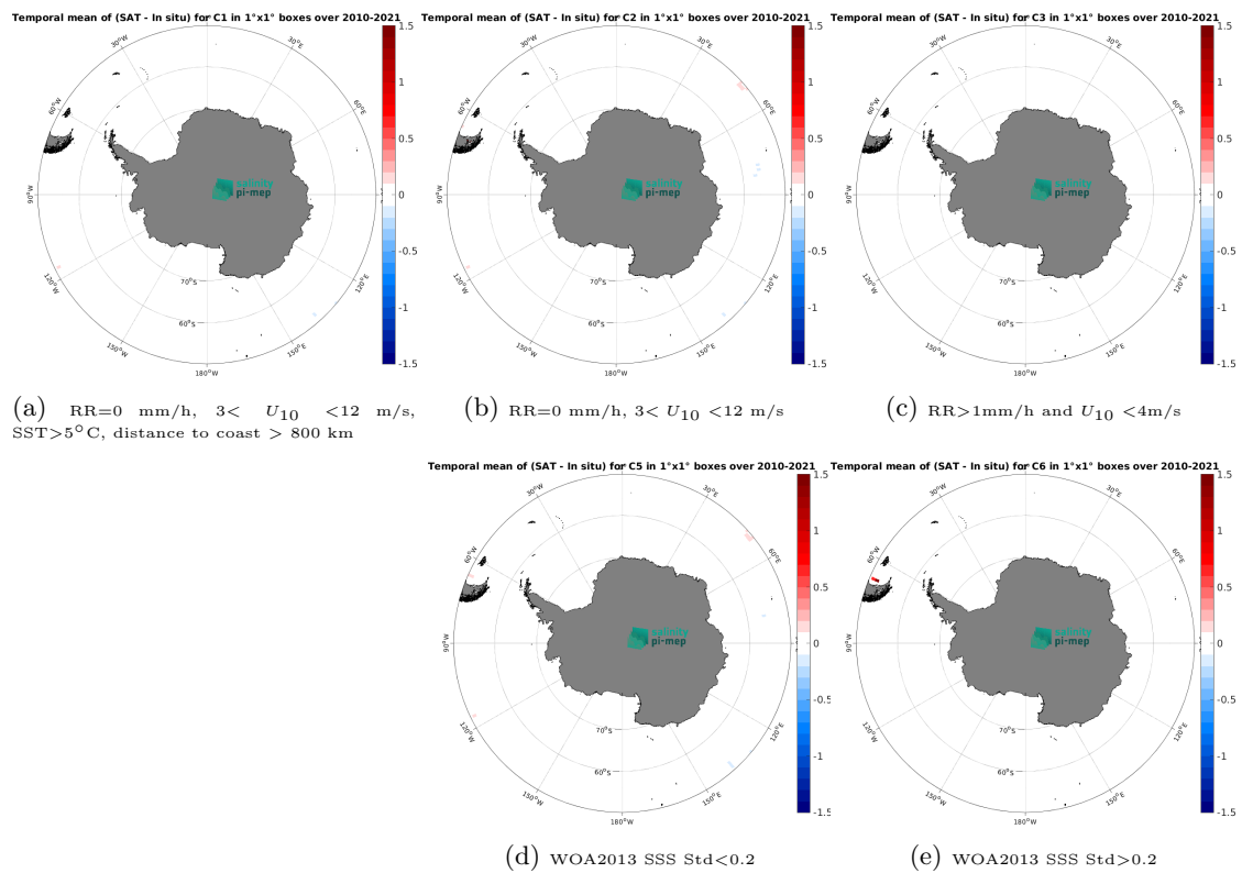
Figure 14: Temporal mean gridded over spatial boxes of size 1^\circ \times 1^\circ of \Delta\text{SSS} (SMOS SSS L4 v1 - Monthly (CMEMS-CNR) - TSG (GOSUD-Research-vessel)) for 5 different subdatasets corresponding to:RR=0 mm/h, 3 < U_{10} < 12 m/s, SST>5°C, distance to coast > 800 km (a), RR=0 mm/h, 3 < U_{10} < 12 m/s (b), RR>1mm/h and U_{10} < 4 m/s (c), WOA2013 SSS Std<0.2 (d), WOA2013 SSS Std>0.2 (e).
