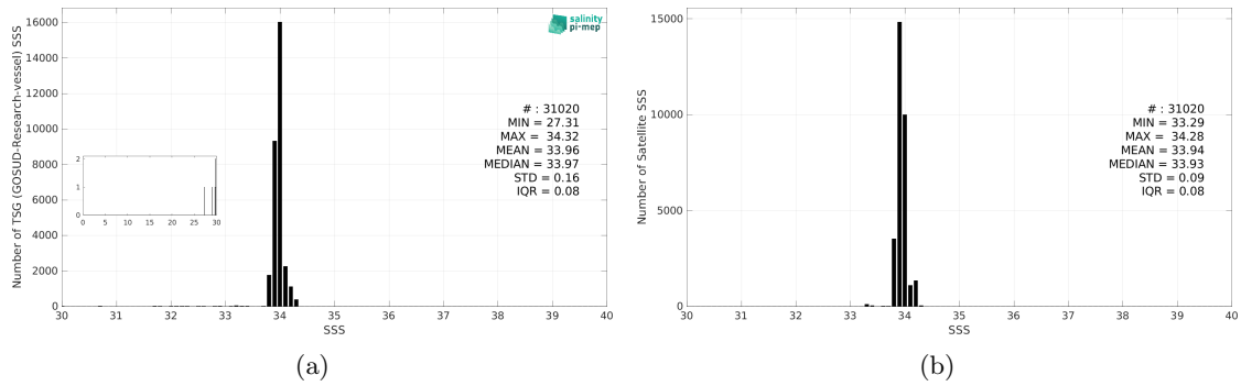
Figure 3: Histograms of SSS from TSG (GOSUD-Research-vessel) (a) and SMOS SSS L4 v1 - Monthly (CMEMS-CNR) (b) considering all match-up pairs per bins of 0.1 over the Southern Ocean Pi-MEP region and for the full satellite product period.
