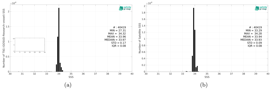
Figure 2: Histograms of SSS from TSG (GOSUD-Research-vessel) (a) and SMOS SSS L4 v1 - Monthly (CMEMS-CNR) (b) considering all match-up pairs per bins of 0.1 over the Southern Ocean Pi-MEP region and for the full satellite product period.
