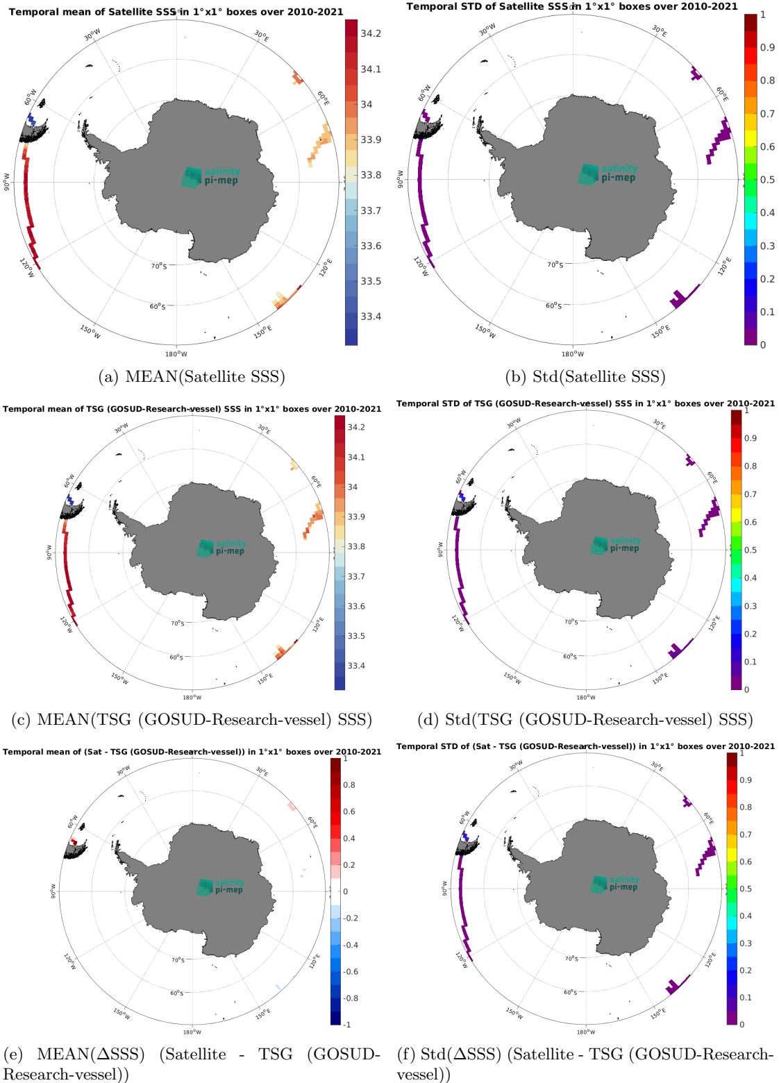
Figure 6: Temporal mean (left) and Std (right) of SSS from SMOS SSS L4 v1 - Monthly (CMEMS-CNR) (top), TSG (GOSUD-Research-vessel) (middle), and of \Delta SSS (Satellite - TSG (GOSUD-Research-vessel)). Only match-up pairs are used to generate these maps.
