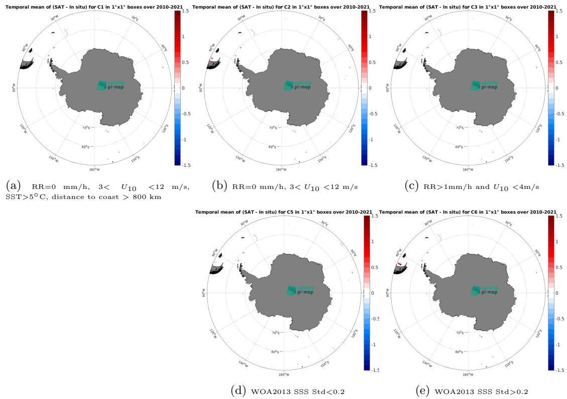
Figure 12: Temporal mean gridded over spatial boxes of size 1^\circ \times 1^\circ of \Delta\text{SSS} (SMOS SSS L4 v1 - Monthly (CMEMS-CNR) - TSG (GOSUD-Research-vessel)) for 5 different subdatasets corresponding to: RR=0 mm/h, 3 < U_{10} < 12 m/s, SST > 5^\circ\text{C} , distance to coast > 800 km (a), RR=0 mm/h, 3 < U_{10} < 12 m/s (b), RR > 1 mm/h and U_{10} < 4 m/s (c), WOA2013 SSS Std < 0.2 (d), WOA2013 SSS Std > 0.2 (e).
