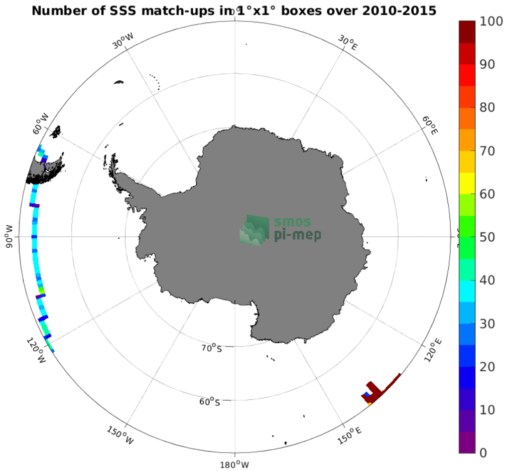
Figure 4: Number of SSS match-ups between TSG (GOSUD-Research-vessel) SSS and the SMOS SSS L4 v1 - Monthly (CMEMS-CNR) SSS product for the Southern Ocean Pi-MEP region over 1^\circ \times 1^\circ boxes and for the full satellite product period.
