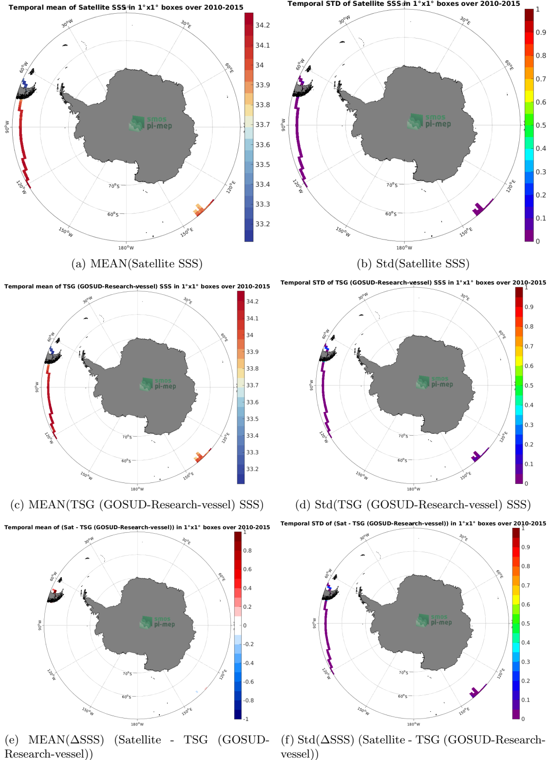
Figure 6: Temporal mean (left) and Std (right) of SSS from SMOS SSS L4 v1 - Monthly (CMEMS-CNR) (top), TSG (GOSUD-Research-vessel) (middle), and of \Delta SSS (Satellite - TSG (GOSUD-Research-vessel)). Only match-up pairs are used to generate these maps.
