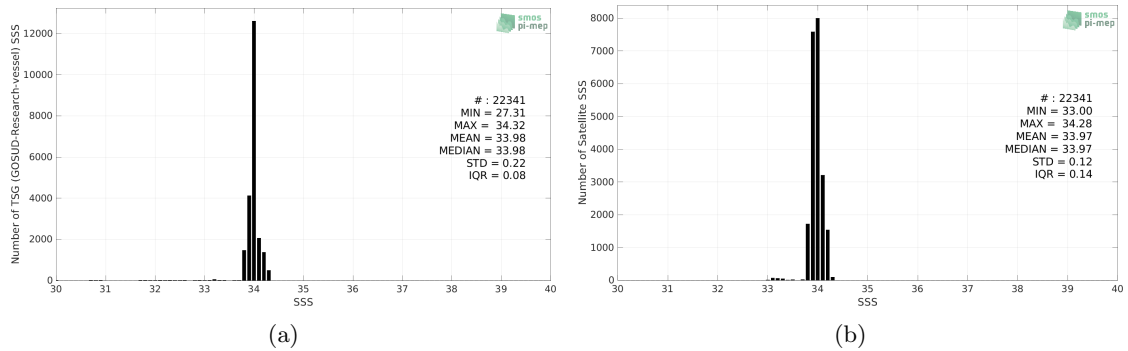
Figure 2: Histograms of SSS from TSG (GOSUD-Research-vessel) (a) and SMOS SSS L4 v1 - Monthly (CMEMS-CNR) (b) considering all match-up pairs per bins of 0.1 over the Southern Ocean Pi-MEP region and for the full satellite product period.
