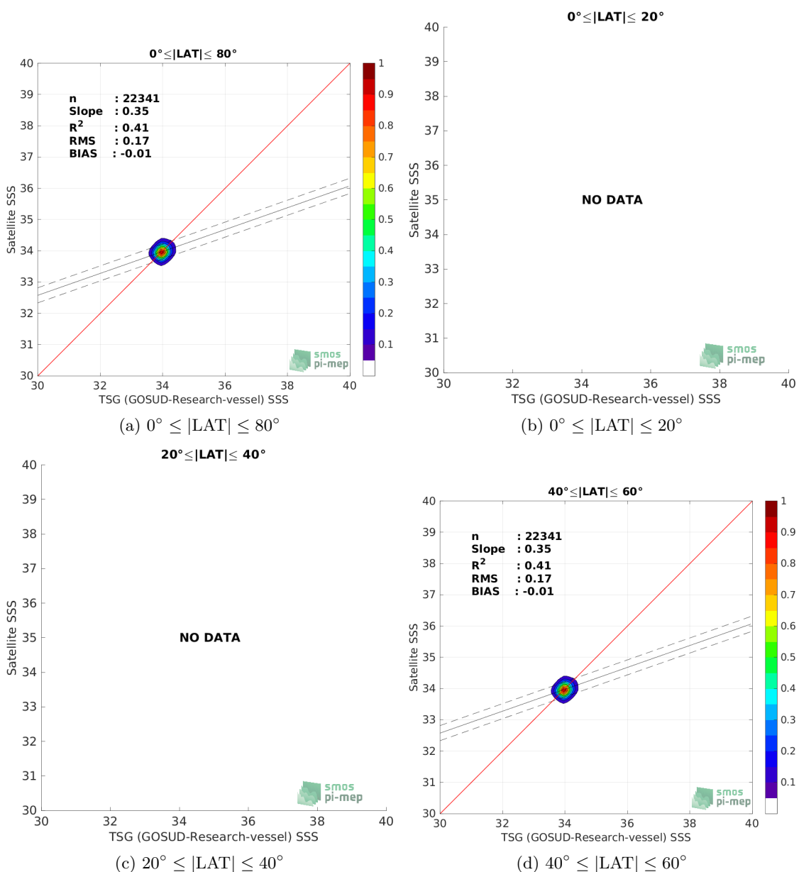
Figure 9: Contour maps of the concentration of SMOS SSS L4 v1 - Monthly (CMEMS-CNR) SSS (y-axis) versus TSG (GOSUD-Research-vessel) SSS (x-axis) at match-up pairs for different latitude bands. For each plot, the red line shows x=y . The black thin and dashed lines indicate a linear fit through the data cloud and the \pm 95\% confidence levels, respectively. The number match-up pairs n , the slope and R^2 coefficient of the linear fit, the root mean square (RMS) and the mean bias between satellite and in situ data are indicated for each latitude band in each plots.
