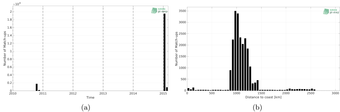
Figure 1: Number of match-ups between TSG (GOSUD-Research-vessel) and SMOS SSS L4 v1 - Monthly (CMEMS-CNR) SSS as a function of time (a) and as function of the distance to coast (b) over the Southern Ocean Pi-MEP region and for the full satellite product period.
