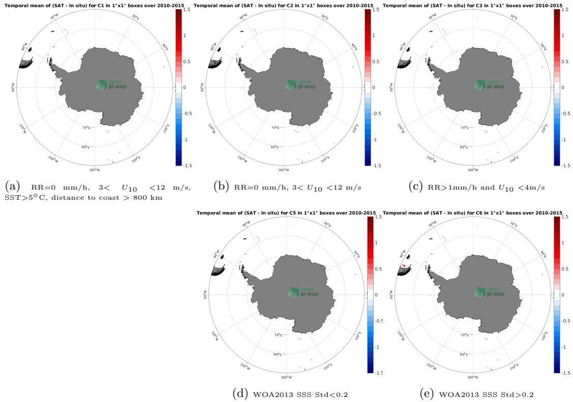
Figure 12: Temporal mean gridded over spatial boxes of size 1^\circ \times 1^\circ of \Delta SSS (SMOS SSS L4 v1 - Monthly (CMEMS-CNR) - TSG (GOSUD-Research-vessel)) for 5 different subdatasets corresponding to:RR=0 mm/h, 3 < U_{10} < 12 m/s, SST >5^\circ C, distance to coast > 800 km (a), RR=0 mm/h, 3 < U_{10} < 12 m/s (b), RR >1 mm/h and U_{10} < 4 m/s (c), WOA2013 SSS Std <0.2 (d), WOA2013 SSS Std >0.2 (e).
