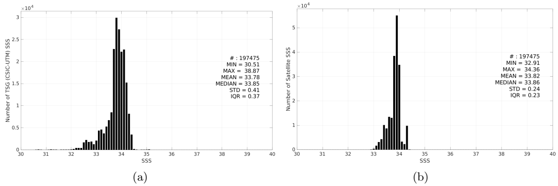
Figure 3: Histograms of SSS from TSG (CSIC-UTM) (a) and SMOS SSS L4 v1 - Monthly (CMEMS-CNR) (b) considering all match-up pairs per bins of 0.1 over the Southern Ocean Pi-MEP region and for the full satellite product period.
