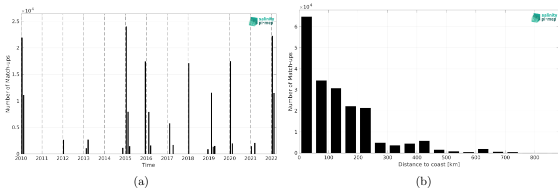
Figure 2: Number of match-ups between TSG (CSIC-UTM) and SMOS SSS L4 v1 - Monthly (CMEMS-CNR) SSS as a function of time (a) and as function of the distance to coast (b) over the Southern Ocean Pi-MEP region and for the full satellite product period.
