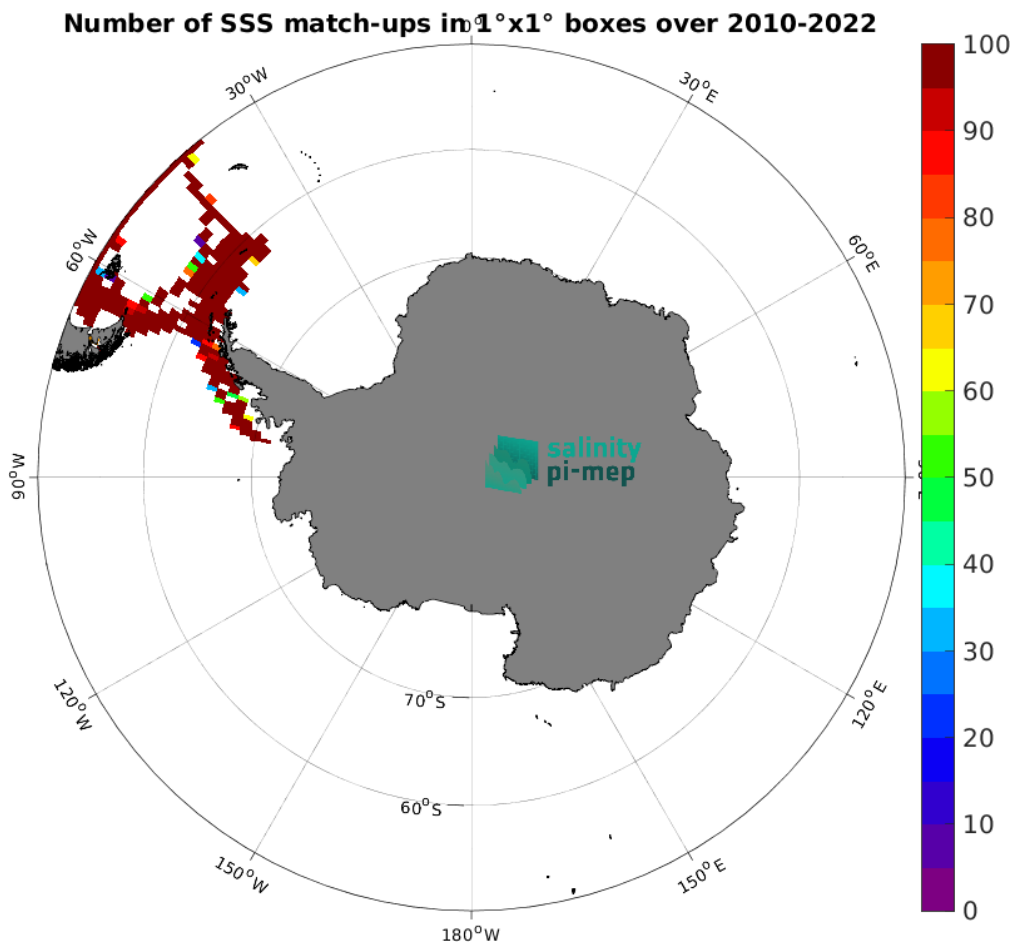
Figure 5: Number of SSS match-ups between TSG (CSIC-UTM) SSS and the SMOS SSS L4 v1 - Monthly (CMEMS-CNR) SSS product for the Southern Ocean Pi-MEP region over 1^\circ \times 1^\circ boxes and for the full satellite product period.
