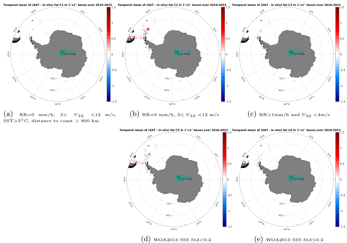
Figure 14: Temporal mean gridded over spatial boxes of size 1^\circ \times 1^\circ of \Delta SSS (SMOS SSS L4 v1 - Monthly (CMEMS-CNR) - TSG (CSIC-UTM)) for 5 different subdatasets corresponding to:RR=0 mm/h, 3 < U_{10} < 12 m/s, SST >5^\circ C, distance to coast > 800 km (a), RR=0 mm/h, 3 < U_{10} < 12 m/s (b), RR >1 mm/h and U_{10} < 4 m/s (c), WOA2013 SSS Std <0.2 (d), WOA2013 SSS Std >0.2 (e).
