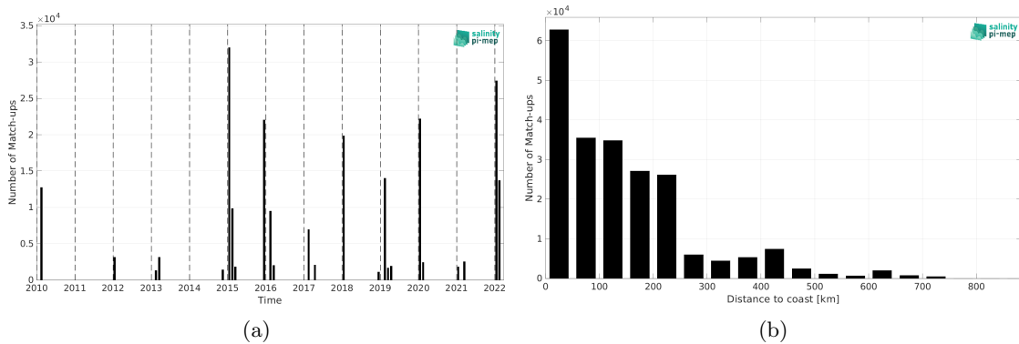
Figure 1: Number of match-ups between TSG (CSIC-UTM) and SMOS SSS L4 v1 - Monthly (CMEMS-CNR) SSS as a function of time (a) and as function of the distance to coast (b) over the Southern Ocean Pi-MEP region and for the full satellite product period.
