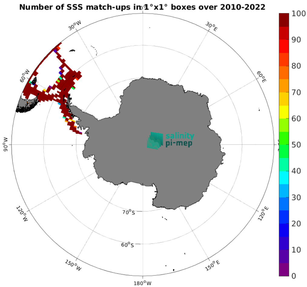
Figure 4: Number of SSS match-ups between TSG (CSIC-UTM) SSS and the SMOS SSS L4 v1 - Monthly (CMEMS-CNR) SSS product for the Southern Ocean Pi-MEP region over 1^\circ \times 1^\circ boxes and for the full satellite product period.
