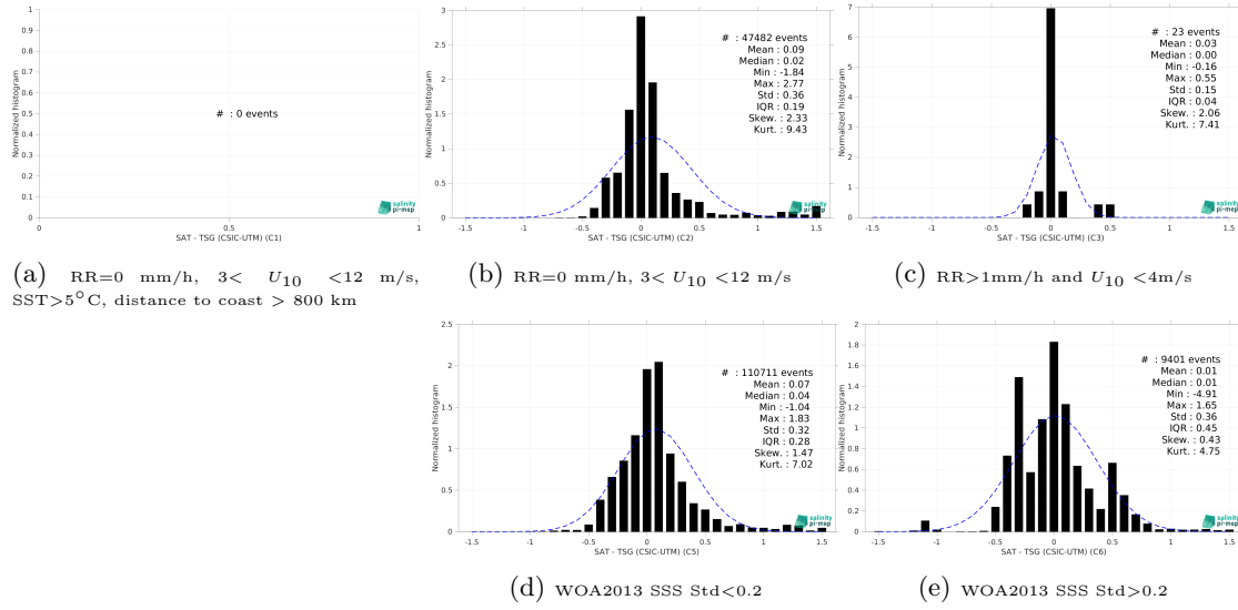
Figure 13: Normalized histogram of \Delta\text{SSS} (SMOS SSS L4 v1 - Monthly (CMEMS-CNR) - TSG (CSIC-UTM)) for 5 different subdatasets corresponding to: RR=0 mm/h, 3 < U_{10} < 12 m/s, SST >5^{\circ}\text{C} , distance to coast > 800 km (a), RR=0 mm/h, 3 < U_{10} < 12 m/s (b), RR>1\text{mm/h} and U_{10} < 4\text{m/s} (c), WOA2013 SSS Std <0.2 (d), WOA2013 SSS Std >0.2 (e).
