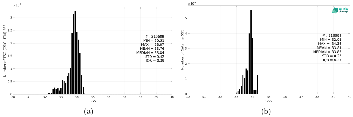
Figure 2: Histograms of SSS from TSG (CSIC-UTM) (a) and SMOS SSS L4 v1 - Monthly (CMEMS-CNR) (b) considering all match-up pairs per bins of 0.1 over the Southern Ocean Pi-MEP region and for the full satellite product period.
