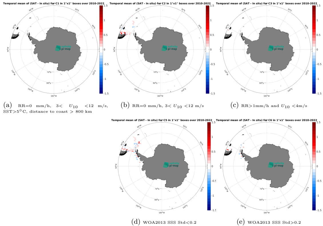
Figure 12: Temporal mean gridded over spatial boxes of size 1^{\circ}\times 1^{\circ} of \Delta\text{SSS} (SMOS SSS L4 v1 - Monthly (CMEMS-CNR) - TSG (CSIC-UTM)) for 5 different subdatasets corresponding to:RR=0 mm/h, 3 < U_{10} < 12 m/s, SST >5^{\circ}\text{C} , distance to coast > 800 km (a), RR=0 mm/h, 3 < U_{10} < 12 m/s (b), RR >1 mm/h and U_{10} < 4 m/s (c), WOA2013 SSS Std <0.2 (d), WOA2013 SSS Std >0.2 (e).
