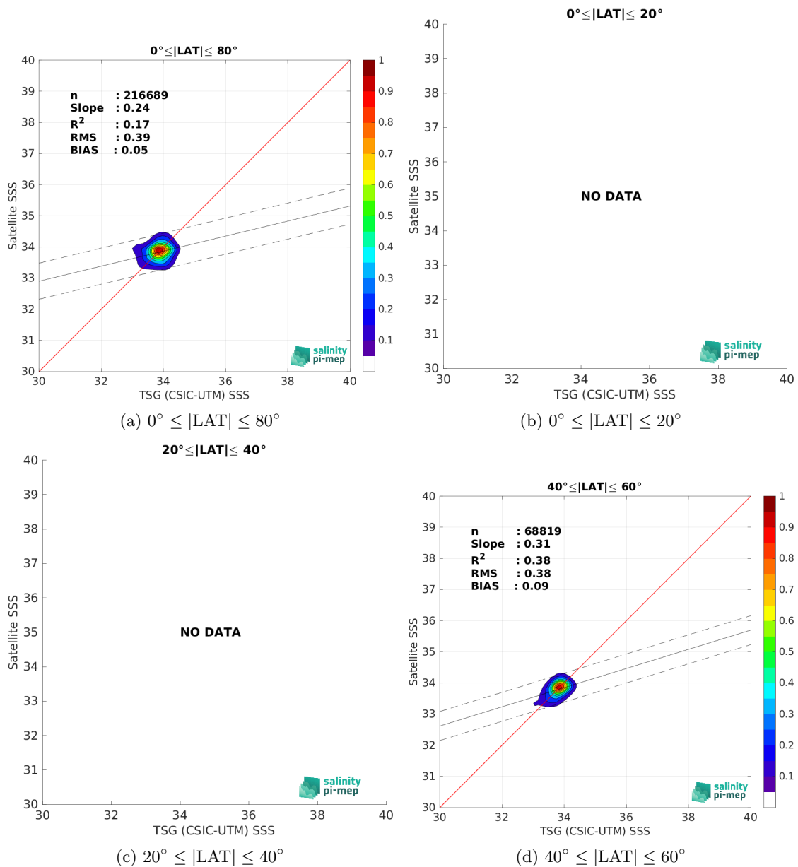
Figure 9: Contour maps of the concentration of SMOS SSS L4 v1 - Monthly (CMEMS-CNR) SSS (y-axis) versus TSG (CSIC-UTM) SSS (x-axis) at match-up pairs for different latitude bands. For each plot, the red line shows x=y . The black thin and dashed lines indicate a linear fit through the data cloud and the \pm 95\% confidence levels, respectively. The number match-up pairs n , the slope and R^2 coefficient of the linear fit, the root mean square (RMS) and the mean bias between satellite and in situ data are indicated for each latitude band in each plots.
