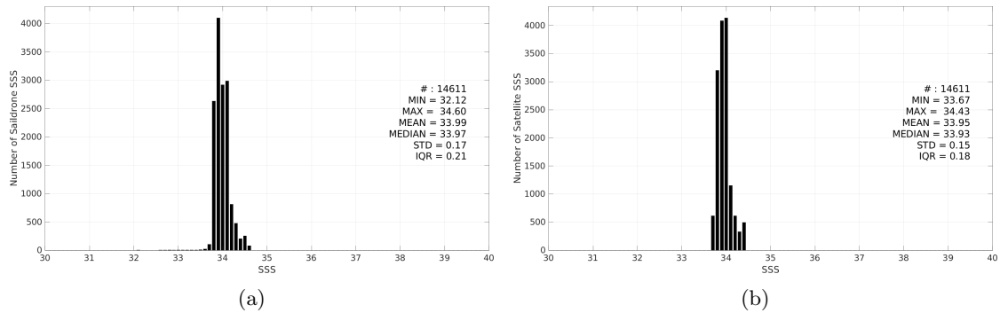
Figure 3: Histograms of SSS from Saildrone (a) and SMOS SSS L4 v1 - Monthly (CMEMS-CNR) (b) considering all match-up pairs per bins of 0.1 over the Southern Ocean Pi-MEP region and for the full satellite product period.
