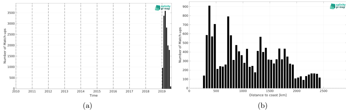
Figure 2: Number of match-ups between Saildrone and SMOS SSS L4 v1 - Monthly (CMEMS-CNR) SSS as a function of time (a) and as function of the distance to coast (b) over the Southern Ocean Pi-MEP region and for the full satellite product period.
