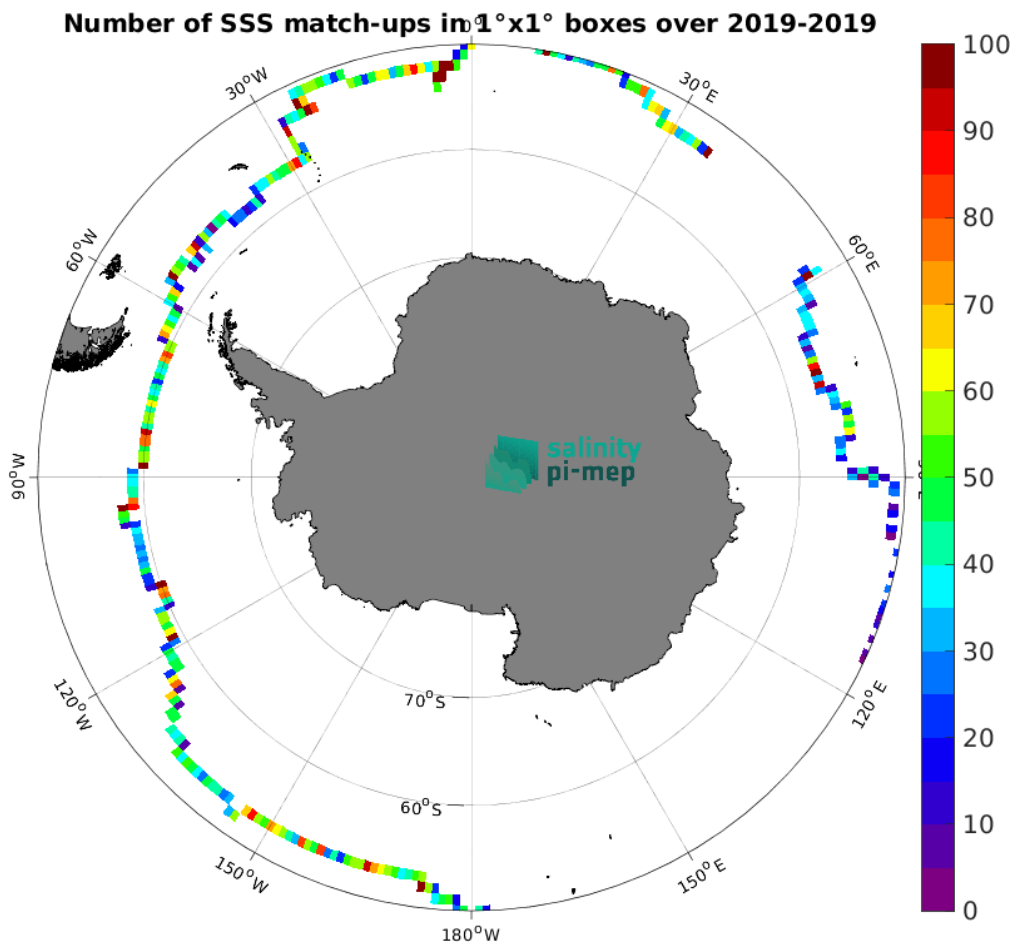
Figure 5: Number of SSS match-ups between Saildrone SSS and the SMOS SSS L4 v1 - Monthly (CMEMS-CNR) SSS product for the Southern Ocean Pi-MEP region over 1^\circ \times 1^\circ boxes and for the full satellite product period.
