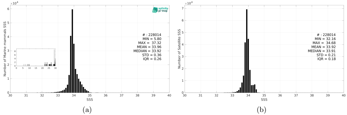
Figure 3: Histograms of SSS from Marine mammals (a) and SMOS SSS L4 v1 - Monthly (CMEMS-CNR) (b) considering all match-up pairs per bins of 0.1 over the Southern Ocean Pi-MEP region and for the full satellite product period.
