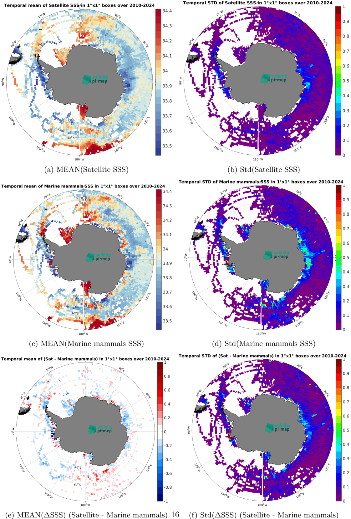
Figure 7: Temporal mean (left) and Std (right) of SSS from SMOS SSS L4 v1 - Monthly (CMEMS-CNR) (top), Marine mammals (middle), and of \Delta SSS (Satellite - Marine mammals). Only match-up pairs are used to generate these maps.
