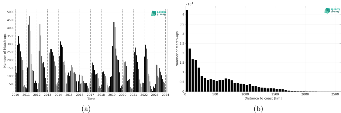
Figure 2: Number of match-ups between Marine mammals and SMOS SSS L4 v1 - Monthly (CMEMS-CNR) SSS as a function of time (a) and as function of the distance to coast (b) over the Southern Ocean Pi-MEP region and for the full satellite product period.
