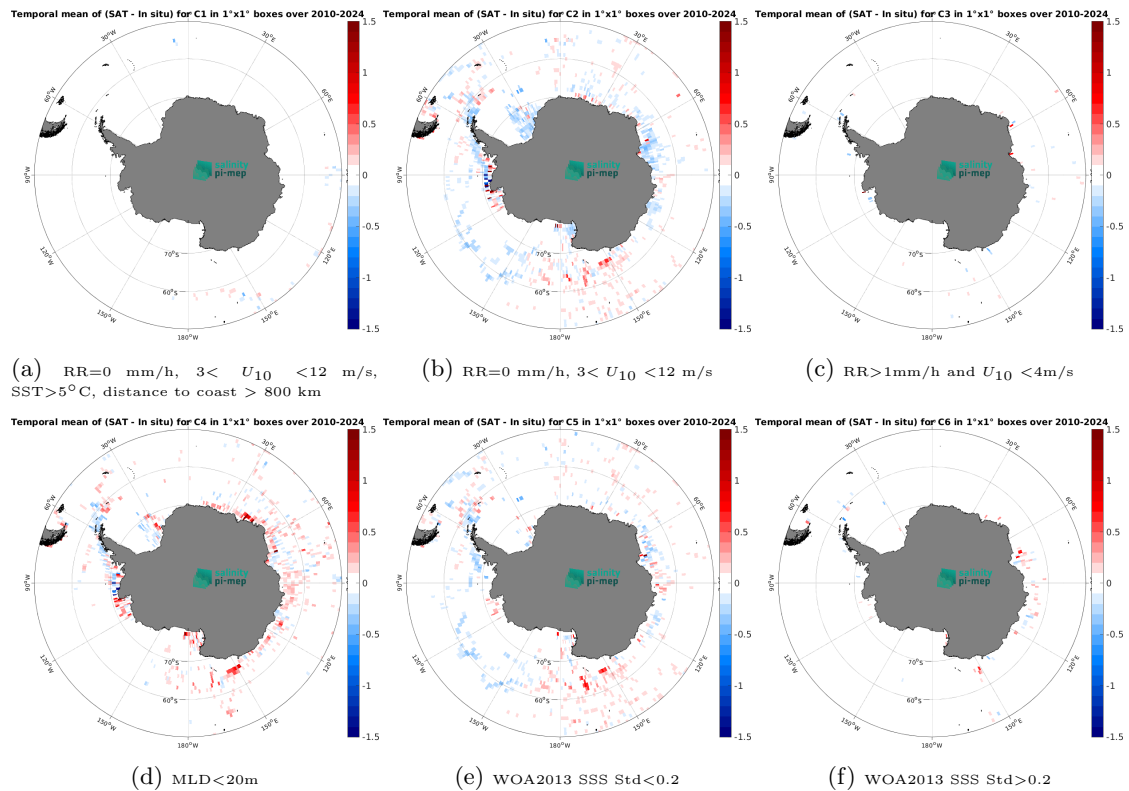
Figure 14: Temporal mean gridded over spatial boxes of size 1^\circ \times 1^\circ of \Delta SSS (SMOS SSS L4 v1 - Monthly (CMEMS-CNR) - Marine mammals) for 6 different subdatasets corresponding to:RR=0 mm/h, 3 < U_{10} < 12 m/s, SST>5°C, distance to coast > 800 km (a), RR=0 mm/h, 3 < U_{10} < 12 m/s (b), RR>1mm/h and U_{10} < 4 m/s (c),MLD<20m (d),WOA2013 SSS Std<0.2 (e),WOA2013 SSS Std>0.2 (f).
