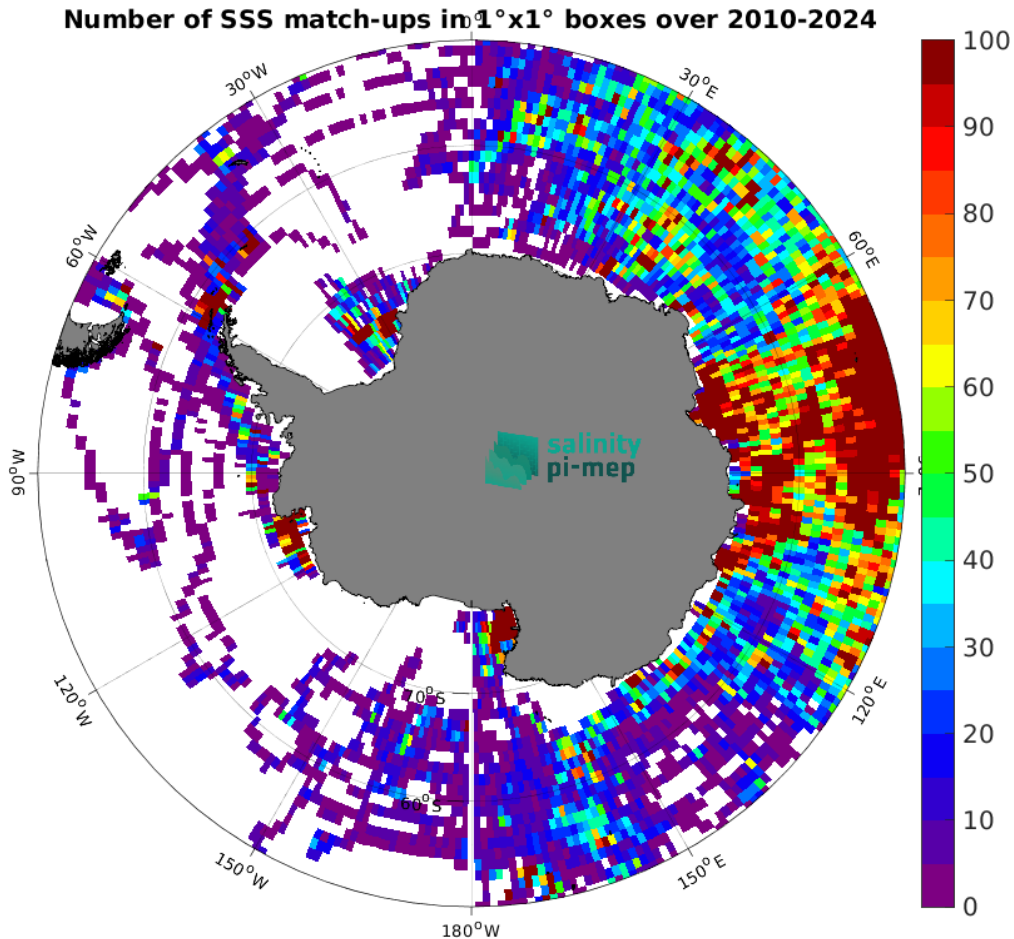
Figure 5: Number of SSS match-ups between Marine mammals SSS and the SMOS SSS L4 v1 - Monthly (CMEMS-CNR) SSS product for the Southern Ocean Pi-MEP region over 1^\circ \times 1^\circ boxes and for the full satellite product period.
