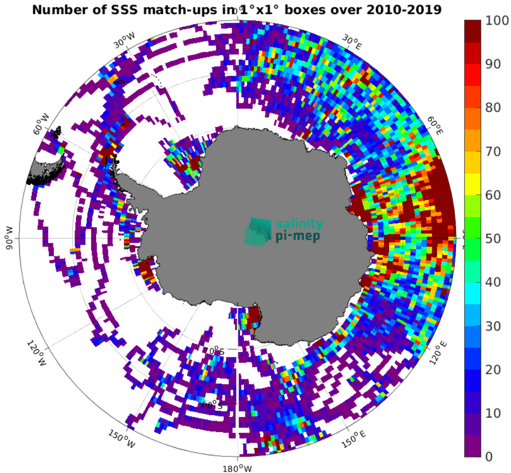
Figure 4: Number of SSS match-ups between Marine mammals SSS and the SMOS SSS L4 v1 - Monthly (CMEMS-CNR) SSS product for the Southern Ocean Pi-MEP region over 1^\circ \times 1^\circ boxes and for the full satellite product period.
