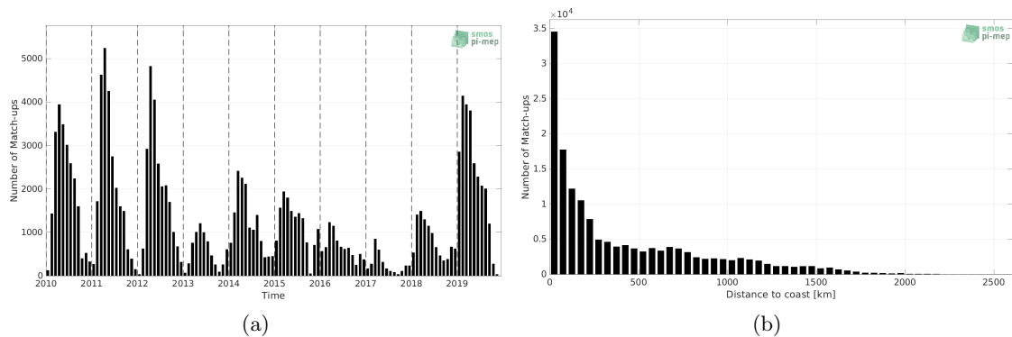
Figure 1: Number of match-ups between Marine mammals and SMOS SSS L4 v1 - Monthly (CMEMS-CNR) SSS as a function of time (a) and as function of the distance to coast (b) over the Southern Ocean Pi-MEP region and for the full satellite product period.
