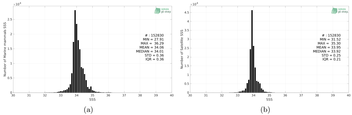
Figure 2: Histograms of SSS from Marine mammals (a) and SMOS SSS L4 v1 - Monthly (CMEMS-CNR) (b) considering all match-up pairs per bins of 0.1 over the Southern Ocean Pi-MEP region and for the full satellite product period.
