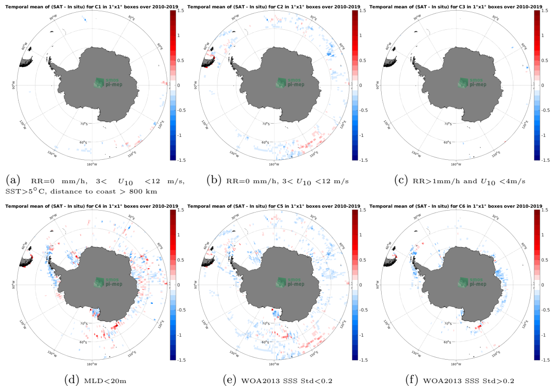
Figure 12: Temporal mean gridded over spatial boxes of size 1^{\circ}\times 1^{\circ} of \Delta\text{SSS} (SMOS SSS L4 v1 - Monthly (CMEMS-CNR) - Marine mammals) for 6 different subdatasets corresponding to: RR=0 mm/h, 3 < U_{10} < 12 m/s, SST > 5^{\circ}\text{C} , distance to coast > 800 km (a), RR=0 mm/h, 3 < U_{10} < 12 m/s (b), RR > 1\text{mm/h} and U_{10} < 4\text{m/s} (c), MLD < 20\text{m} (d), WOA2013 SSS Std < 0.2 (e), WOA2013 SSS Std > 0.2 (f).
