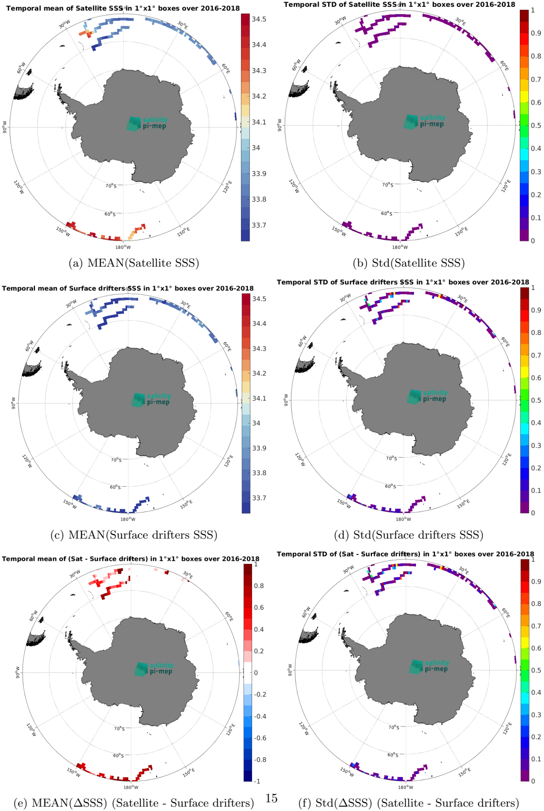
Figure 5: Temporal mean (left) and Std (right) of SSS from SMOS SSS L4 v1 - Monthly (CMEMS-CNR) (top), Surface drifters (middle), and of \Delta SSS (Satellite - Surface drifters). Only match-up pairs are used to generate these maps.
