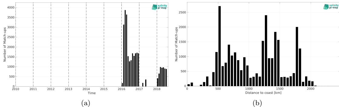
Figure 1: Number of match-ups between Surface drifters and SMOS SSS L4 v1 - Monthly (CMEMS-CNR) SSS as a function of time (a) and as function of the distance to coast (b) over the Southern Ocean Pi-MEP region and for the full satellite product period.
