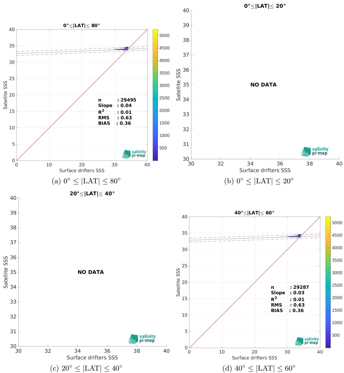
Figure 8: Contour maps of the concentration of SMOS SSS L4 v1 - Monthly (CMEMS-CNR) SSS (y-axis) versus Surface drifters SSS (x-axis) at match-up pairs for different latitude bands. For each plot, the red line shows x=y . The black thin and dashed lines indicate a linear fit through the data cloud and the \pm 95\% confidence levels, respectively. The number match-up pairs n , the slope and R^2 coefficient of the linear fit, the root mean square (RMS) and the mean bias between satellite and in situ data are indicated for each latitude band in each plots.
