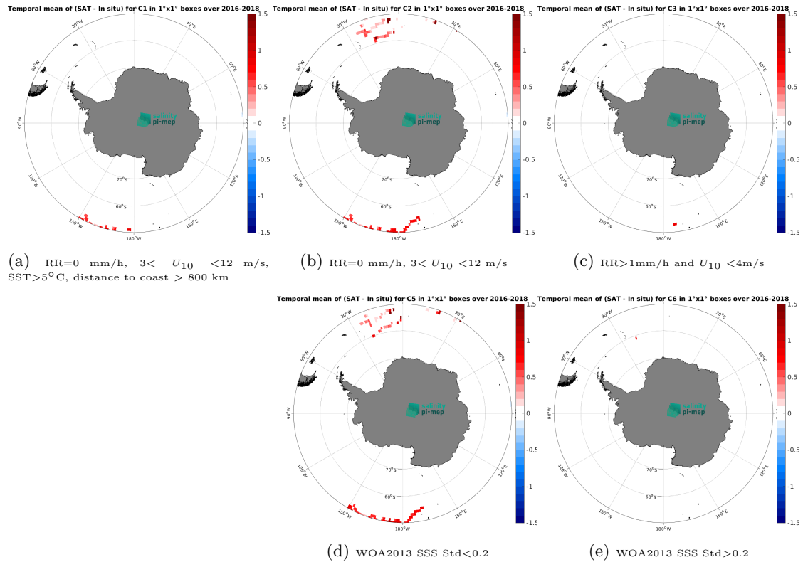
Figure 11: Temporal mean gridded over spatial boxes of size 1^{\circ}\times 1^{\circ} of \Delta\text{SSS} (SMOS SSS L4 v1 - Monthly (CMEMS-CNR) - Surface drifters) for 5 different subdatasets corresponding to:RR=0 mm/h, 3 < U_{10} < 12 m/s, SST >5^{\circ}\text{C} , distance to coast > 800 km (a), RR=0 mm/h, 3 < U_{10} < 12 m/s (b), RR >1 mm/h and U_{10} < 4 m/s (c), WOA2013 SSS Std <0.2 (d), WOA2013 SSS Std >0.2 (e).
