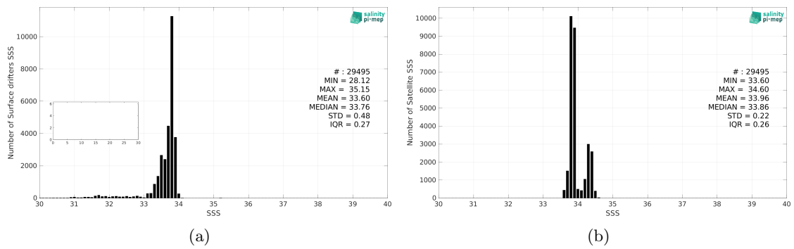
Figure 2: Histograms of SSS from Surface drifters (a) and SMOS SSS L4 v1 - Monthly (CMEMS-CNR) (b) considering all match-up pairs per bins of 0.1 over the Southern Ocean Pi-MEP region and for the full satellite product period.
