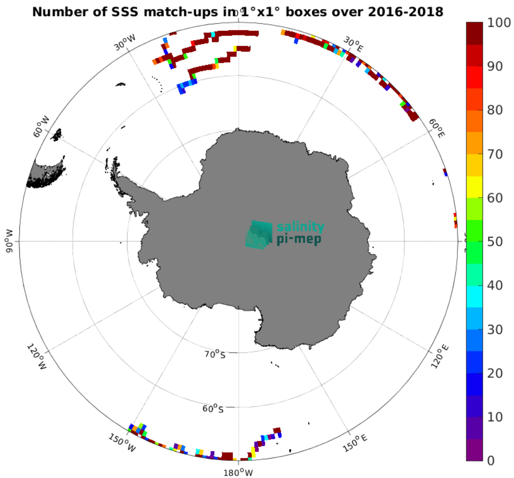
Figure 3: Number of SSS match-ups between Surface drifters SSS and the SMOS SSS L4 v1 - Monthly (CMEMS-CNR) SSS product for the Southern Ocean Pi-MEP region over 1^\circ \times 1^\circ boxes and for the full satellite product period.
