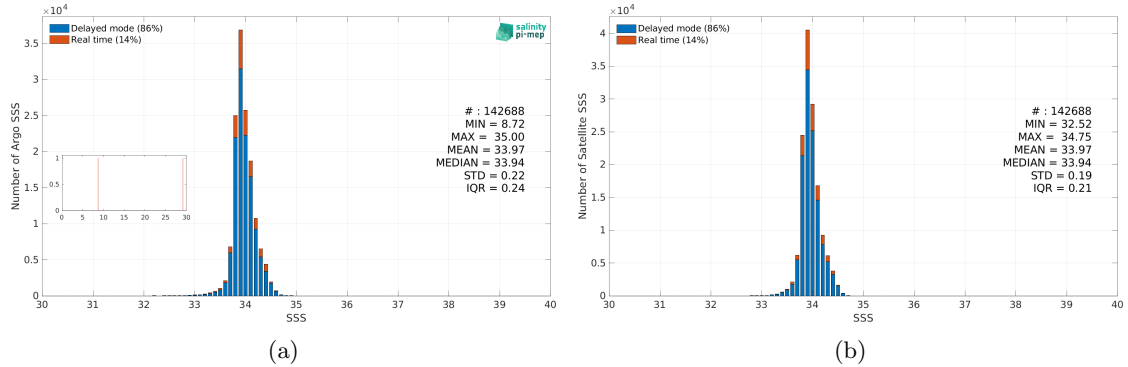
Figure 3: Histograms of SSS from Argo (a) and SMOS SSS L4 v1 - Monthly (CMEMS-CNR) (b) considering all match-up pairs per bins of 0.1 over the Southern Ocean Pi-MEP region and for the full satellite product period.
