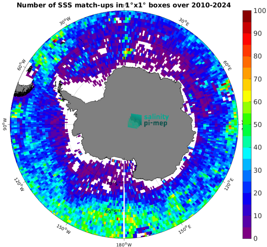
Figure 5: Number of SSS match-ups between Argo SSS and the SMOS SSS L4 v1 - Monthly (CMEMS-CNR) SSS product for the Southern Ocean Pi-MEP region over 1^\circ \times 1^\circ boxes and for the full satellite product period.
