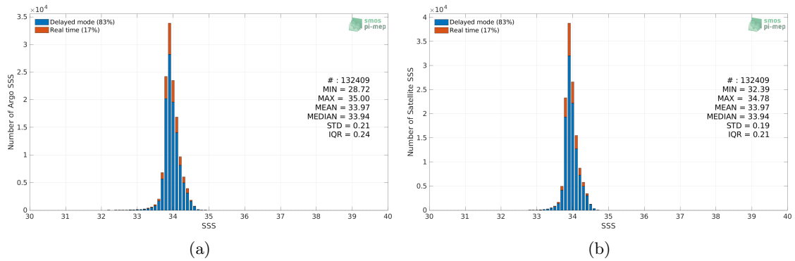
Figure 2: Histograms of SSS from Argo (a) and SMOS SSS L4 v1 - Monthly (CMEMS-CNR) (b) considering all match-up pairs per bins of 0.1 over the Southern Ocean Pi-MEP region and for the full satellite product period.
