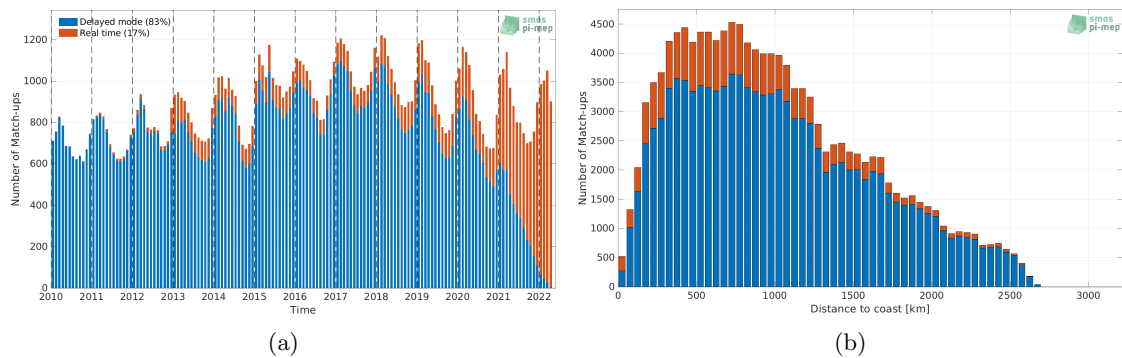
Figure 1: Number of match-ups between Argo and SMOS SSS L4 v1 - Monthly (CMEMS-CNR) SSS as a function of time (a) and as function of the distance to coast (b) over the Southern Ocean Pi-MEP region and for the full satellite product period.
