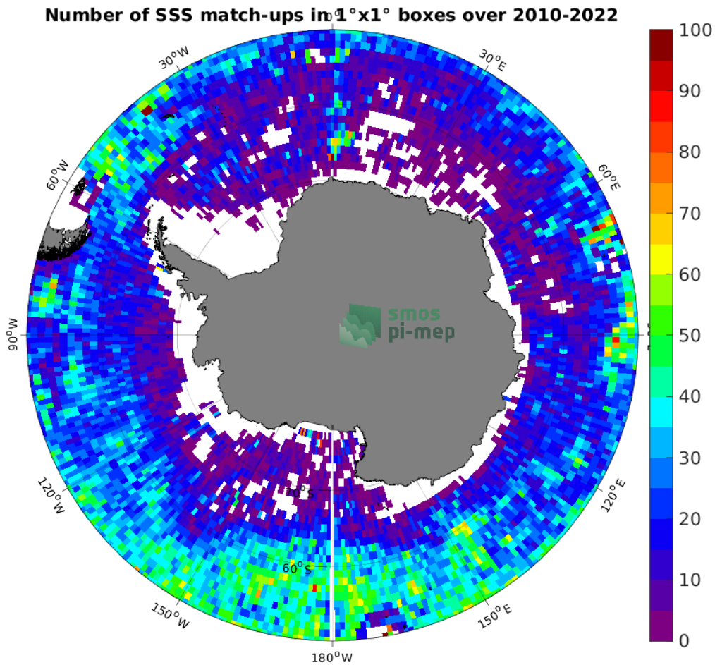
Figure 4: Number of SSS match-ups between Argo SSS and the SMOS SSS L4 v1 - Monthly (CMEMS-CNR) SSS product for the Southern Ocean Pi-MEP region over 1^\circ \times 1^\circ boxes and for the full satellite product period.
