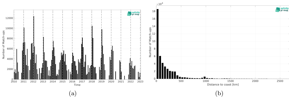
Figure 2: Number of match-ups between TSG (SAMOS) and SMOS SSS L4 v1 - Daily (CMEMS-CNR) SSS as a function of time (a) and as function of the distance to coast (b) over the Southern Ocean Pi-MEP region and for the full satellite product period.
