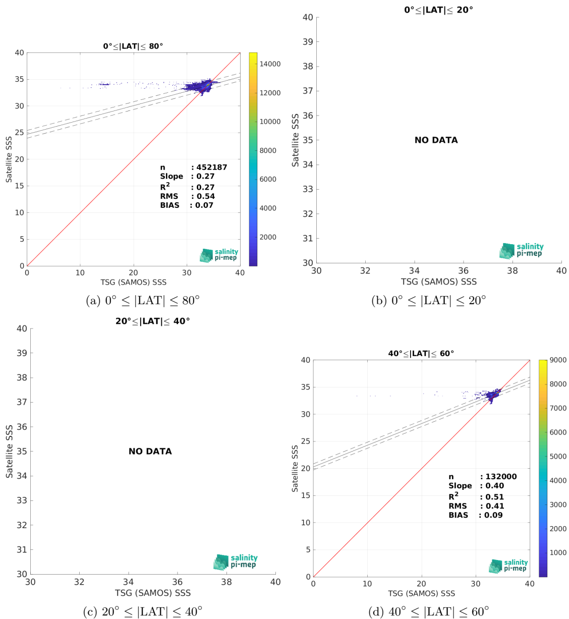
Figure 10: Contour maps of the concentration of SMOS SSS L4 v1 - Daily (CMEMS-CNR) SSS (y-axis) versus TSG (SAMOS) SSS (x-axis) at match-up pairs for different latitude bands. For each plot, the red line shows x=y . The black thin and dashed lines indicate a linear fit through the data cloud and the \pm 95\% confidence levels, respectively. The number match-up pairs n , the slope and R^2 coefficient of the linear fit, the root mean square (RMS) and the mean bias between satellite and in situ data are indicated for each latitude band in each plots.
