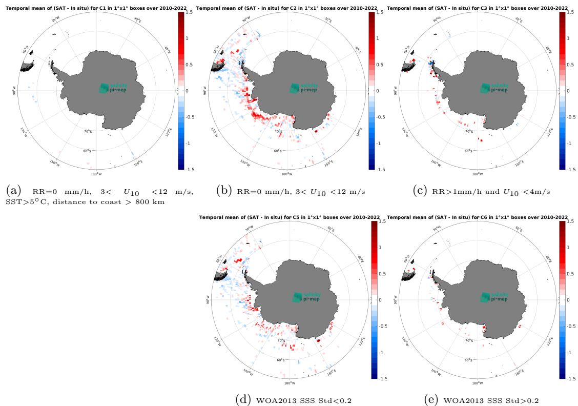
Figure 14: Temporal mean gridded over spatial boxes of size 1^\circ \times 1^\circ of \Delta SSS (SMOS SSS L4 v1 - Daily (CMEMS-CNR) - TSG (SAMOS)) for 5 different subdatasets corresponding to:RR=0 mm/h, 3 < U_{10} < 12 m/s, SST >5^\circ\text{C} , distance to coast > 800 km (a), RR=0 mm/h, 3 < U_{10} < 12 m/s (b), RR >1 mm/h and U_{10} < 4 m/s (c), WOA2013 SSS Std <0.2 (d), WOA2013 SSS Std >0.2 (e).
