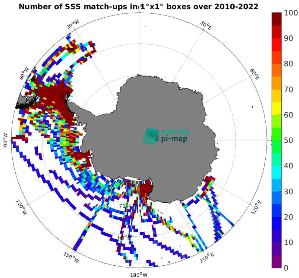
Figure 5: Number of SSS match-ups between TSG (SAMOS) SSS and the SMOS SSS L4 v1 - Daily (CMEMS-CNR) SSS product for the Southern Ocean Pi-MEP region over 1^{\circ} \times 1^{\circ} boxes and for the full satellite product period.
