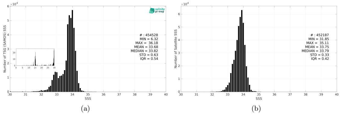
Figure 3: Histograms of SSS from TSG (SAMOS) (a) and SMOS SSS L4 v1 - Daily (CMEMS-CNR) (b) considering all match-up pairs per bins of 0.1 over the Southern Ocean Pi-MEP region and for the full satellite product period.
