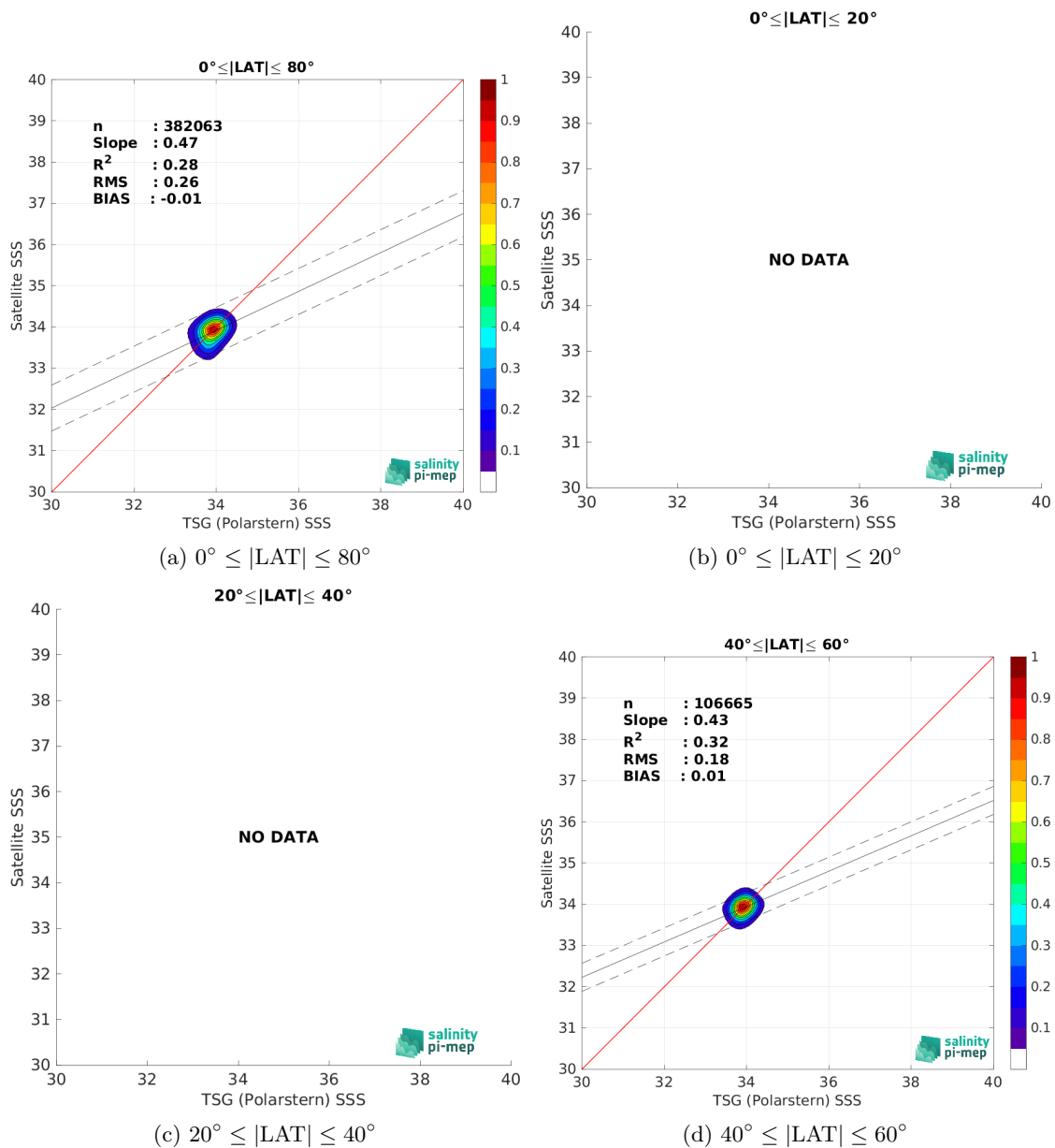
Figure 10: Contour maps of the concentration of SMOS SSS L4 v1 - Daily (CMEMS-CNR) SSS (y-axis) versus TSG (Polarstern) SSS (x-axis) at match-up pairs for different latitude bands. For each plot, the red line shows x=y . The black thin and dashed lines indicate a linear fit through the data cloud and the \pm 95\% confidence levels, respectively. The number match-up pairs n , the slope and R^2 coefficient of the linear fit, the root mean square (RMS) and the mean bias between satellite and in situ data are indicated for each latitude band in each plots.
