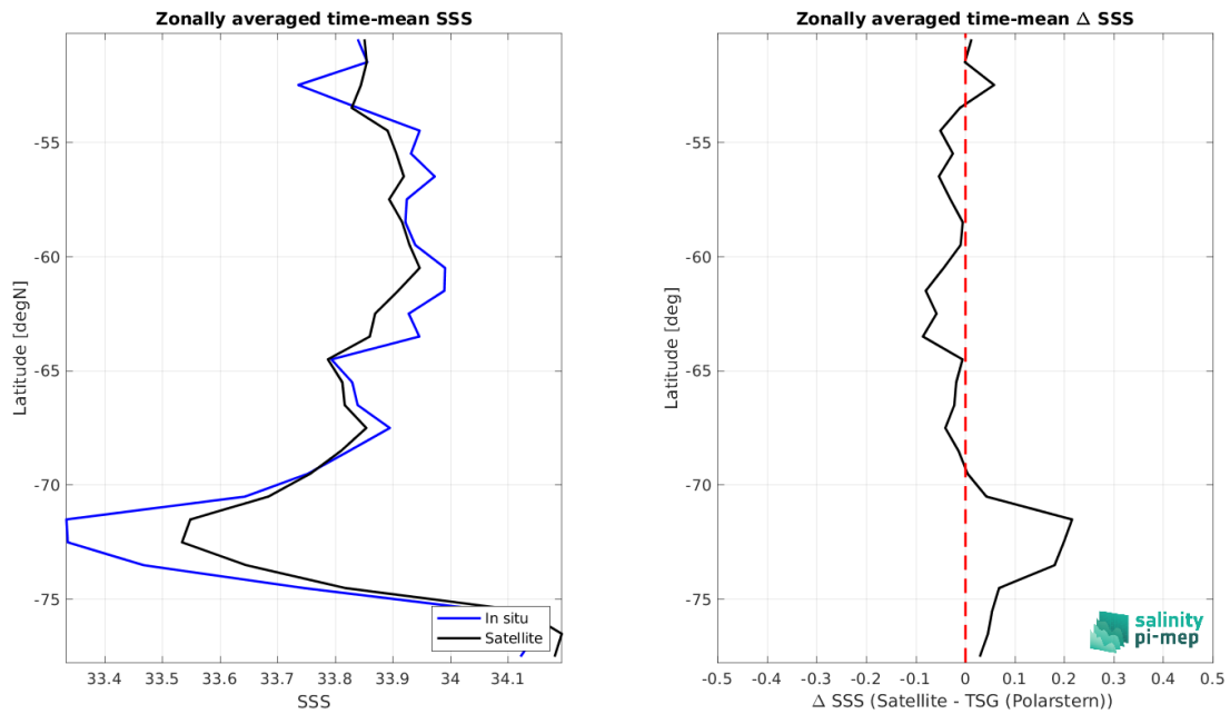
Figure 9: Left panel: Zonal mean SSS from SMOS SSS L4 v1 - Daily (CMEMS-CNR) satellite product (black) and from TSG (Polarstern) (blue). Right panel: Zonal mean of \Delta SSS (Satellite - TSG (Polarstern)) for all the collected Pi-MEP match-up pairs estimated over the full satellite product period.
