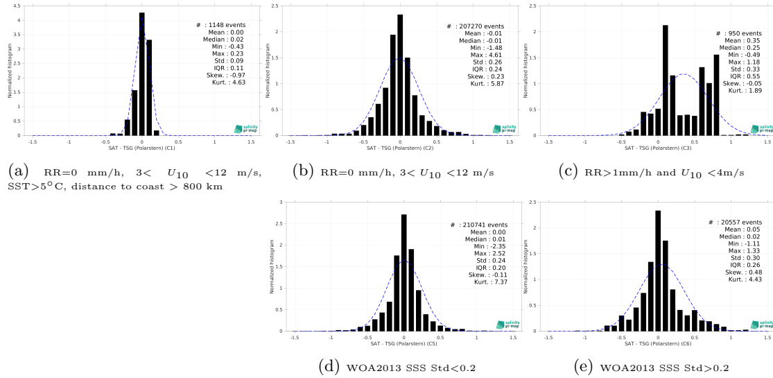
Figure 15: Normalized histogram of \Delta SSS (SMOS SSS L4 v1 - Daily (CMEMS-CNR) - TSG (Polarstern)) for 5 different subdatasets corresponding to: RR=0 mm/h, 3 < U_{10} < 12 m/s, SST>5°C, distance to coast > 800 km (a), RR=0 mm/h, 3 < U_{10} < 12 m/s (b), RR>1mm/h and U_{10} < 4 m/s (c), WOA2013 SSS Std<0.2 (d), WOA2013 SSS Std>0.2 (e).
