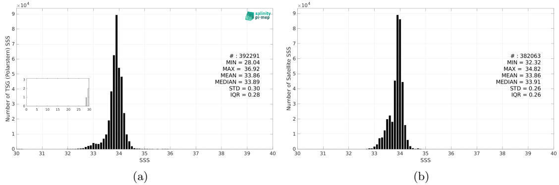
Figure 3: Histograms of SSS from TSG (Polarstern) (a) and SMOS SSS L4 v1 - Daily (CMEMS-CNR) (b) considering all match-up pairs per bins of 0.1 over the Southern Ocean Pi-MEP region and for the full satellite product period.
