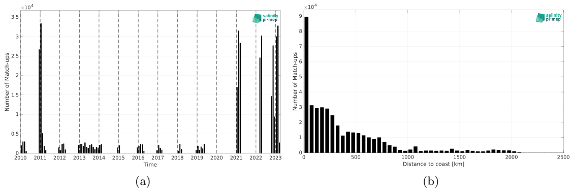
Figure 2: Number of match-ups between TSG (Polarstern) and SMOS SSS L4 v1 - Daily (CMEMS-CNR) SSS as a function of time (a) and as function of the distance to coast (b) over the Southern Ocean Pi-MEP region and for the full satellite product period.
