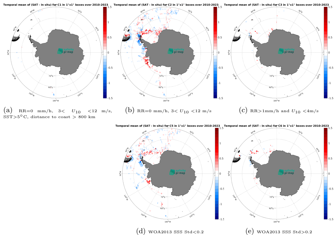
Figure 14: Temporal mean gridded over spatial boxes of size 1^\circ \times 1^\circ of \Delta SSS (SMOS SSS L4 v1 - Daily (CMEMS-CNR) - TSG (Polarstern)) for 5 different subdatasets corresponding to:RR=0 mm/h, 3 < U_{10} < 12 m/s, SST > 5^\circ\text{C} , distance to coast > 800 km (a), RR=0 mm/h, 3 < U_{10} < 12 m/s (b), RR > 1 mm/h and U_{10} < 4 m/s (c), WOA2013 SSS Std < 0.2 (d), WOA2013 SSS Std > 0.2 (e).
