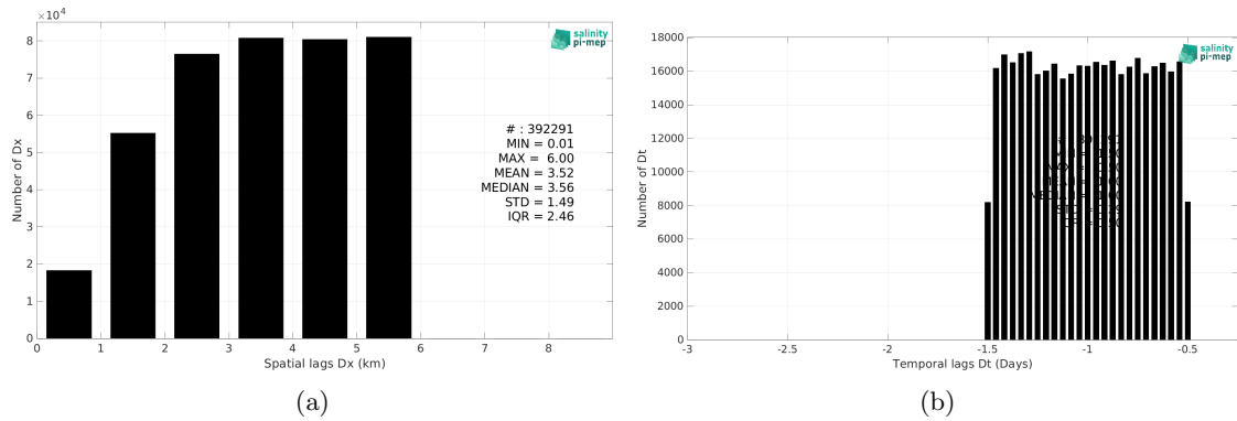
Figure 6: Histograms of the spatial (a) and temporal (b) lags between the location/time of the TSG (Polarstern) measurement and the date of the corresponding SMOS SSS L4 v1 - Daily (CMEMS-CNR) SSS pixel.
