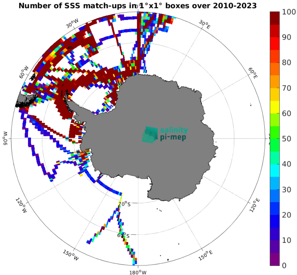
Figure 5: Number of SSS match-ups between TSG (Polarstern) SSS and the SMOS SSS L4 v1 - Daily (CMEMS-CNR) SSS product for the Southern Ocean Pi-MEP region over 1^\circ \times 1^\circ boxes and for the full satellite product period.
