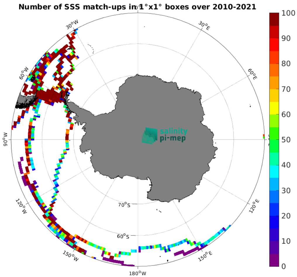
Figure 5: Number of SSS match-ups between TSG (GOSUD-Sailing-ship) SSS and the SMOS SSS L4 v1 - Daily (CMEMS-CNR) SSS product for the Southern Ocean Pi-MEP region over 1^\circ \times 1^\circ boxes and for the full satellite product period.
