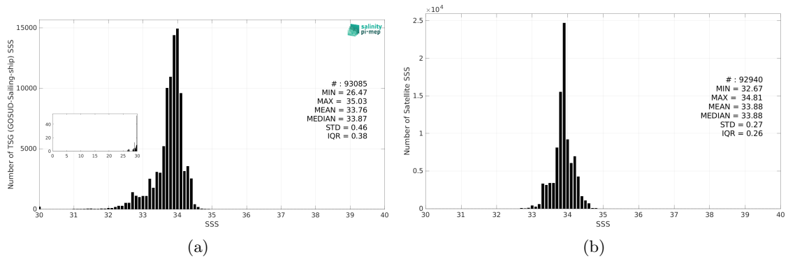
Figure 3: Histograms of SSS from TSG (GOSUD-Sailing-ship) (a) and SMOS SSS L4 v1 - Daily (CMEMS-CNR) (b) considering all match-up pairs per bins of 0.1 over the Southern Ocean Pi-MEP region and for the full satellite product period.
