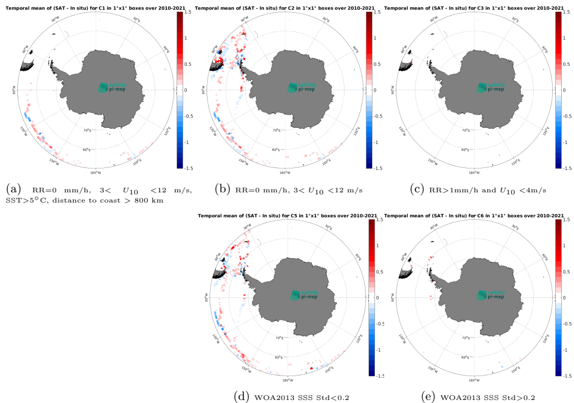
Figure 14: Temporal mean gridded over spatial boxes of size 1^\circ \times 1^\circ of \Delta\text{SSS} (SMOS SSS L4 v1 - Daily (CMEMS-CNR) - TSG (GOSUD-Sailing-ship)) for 5 different subdatasets corresponding to:RR=0 mm/h, 3 < U_{10} < 12 m/s, SST >5^\circ\text{C} , distance to coast > 800 km (a), RR=0 mm/h, 3 < U_{10} < 12 m/s (b), RR >1 mm/h and U_{10} < 4 m/s (c), WOA2013 SSS Std <0.2 (d), WOA2013 SSS Std >0.2 (e).
