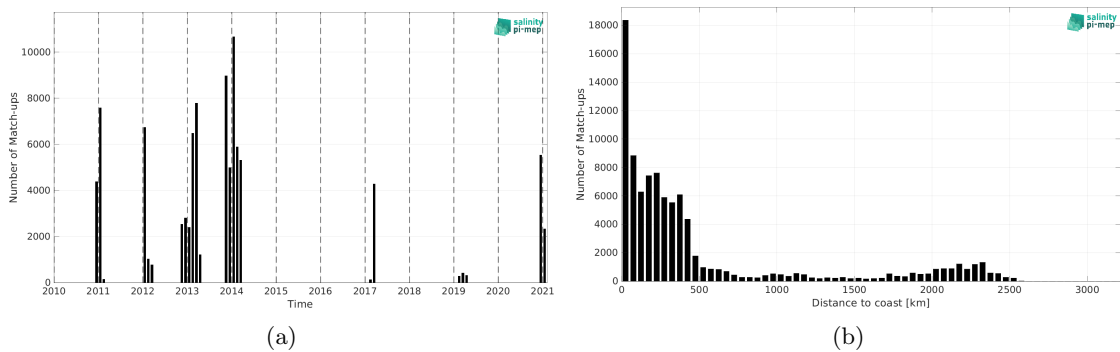
Figure 2: Number of match-ups between TSG (GOSUD-Sailing-ship) and SMOS SSS L4 v1 - Daily (CMEMS-CNR) SSS as a function of time (a) and as function of the distance to coast (b) over the Southern Ocean Pi-MEP region and for the full satellite product period.
