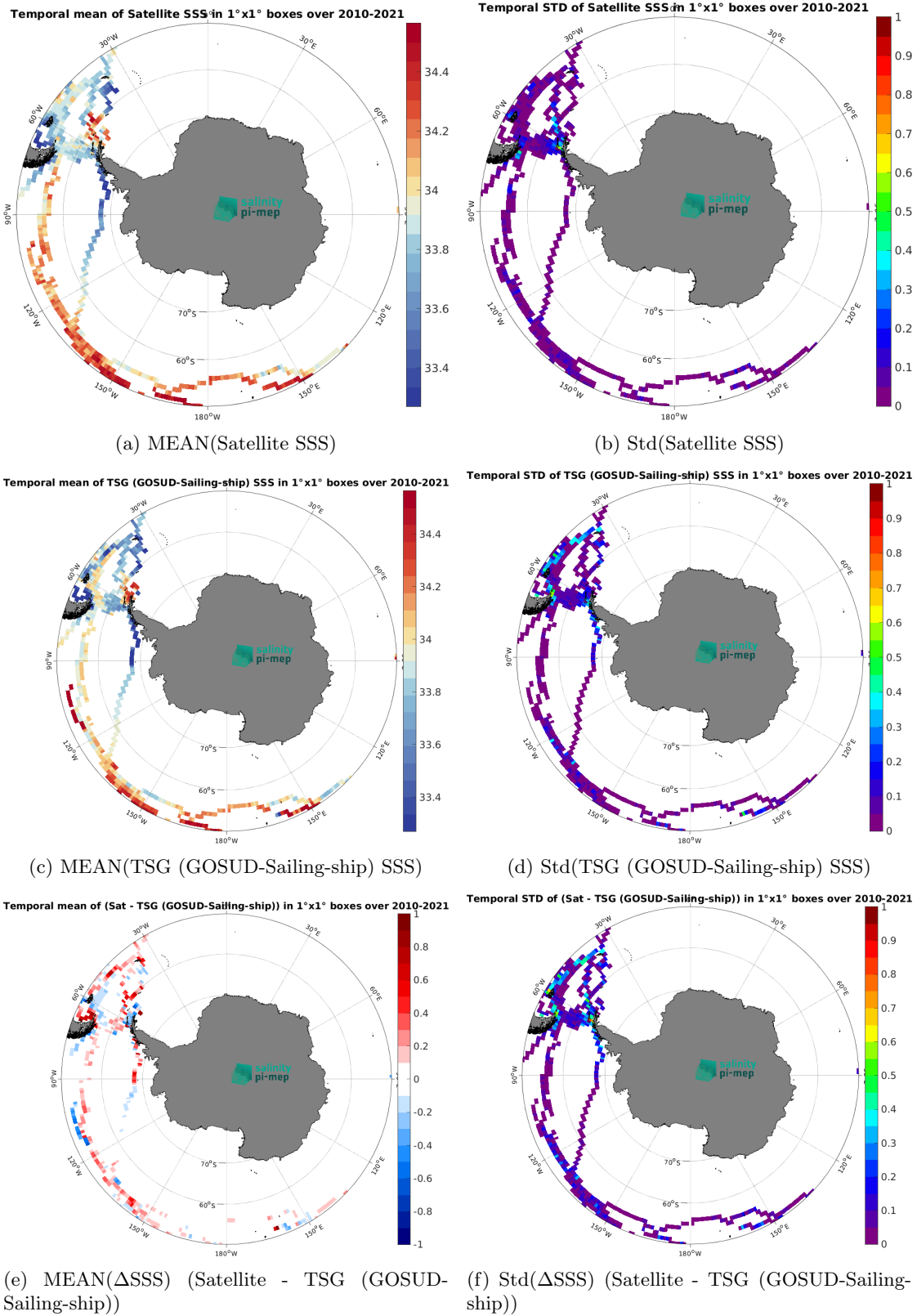
Figure 7: Temporal mean (left) and Std (right) of SSS from SMOS SSS L4 v1 - Daily (CMEMS-CNR) (top), TSG (GOSUD-Sailing-ship) (middle), and of \Delta SSS (Satellite - TSG (GOSUD-Sailing-ship)). Only match-up pairs are used to generate these maps.
