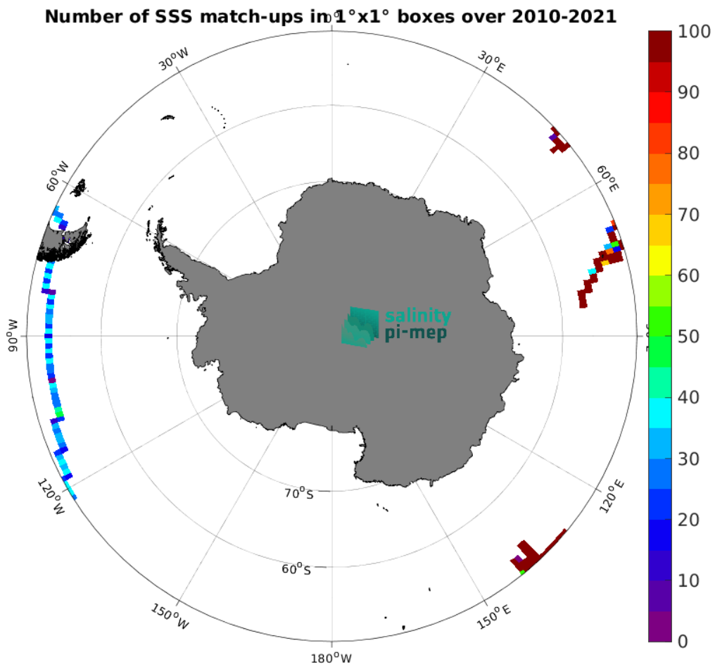
Figure 5: Number of SSS match-ups between TSG (GOSUD-Research-vessel) SSS and the SMOS SSS L4 v1 - Daily (CMEMS-CNR) SSS product for the Southern Ocean Pi-MEP region over 1^\circ \times 1^\circ boxes and for the full satellite product period.
