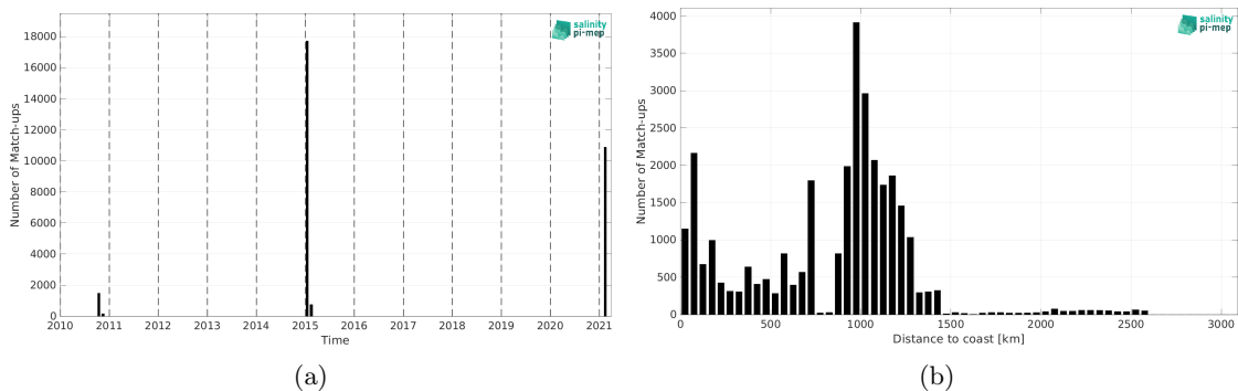
Figure 2: Number of match-ups between TSG (GOSUD-Research-vessel) and SMOS SSS L4 v1 - Daily (CMEMS-CNR) SSS as a function of time (a) and as function of the distance to coast (b) over the Southern Ocean Pi-MEP region and for the full satellite product period.
