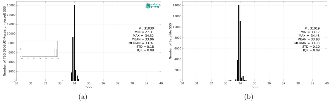
Figure 3: Histograms of SSS from TSG (GOSUD-Research-vessel) (a) and SMOS SSS L4 v1 - Daily (CMEMS-CNR) (b) considering all match-up pairs per bins of 0.1 over the Southern Ocean Pi-MEP region and for the full satellite product period.
