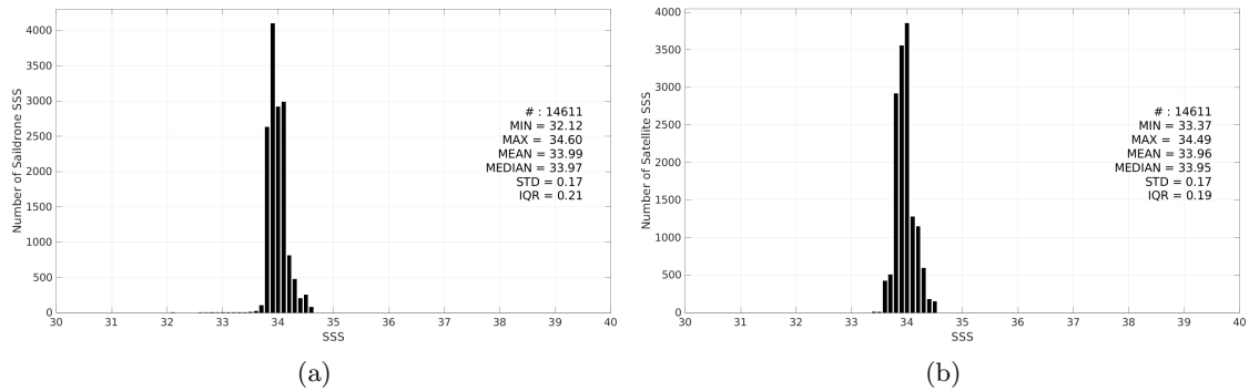
Figure 3: Histograms of SSS from Saildrone (a) and SMOS SSS L4 v1 - Daily (CMEMS-CNR) (b) considering all match-up pairs per bins of 0.1 over the Southern Ocean Pi-MEP region and for the full satellite product period.
