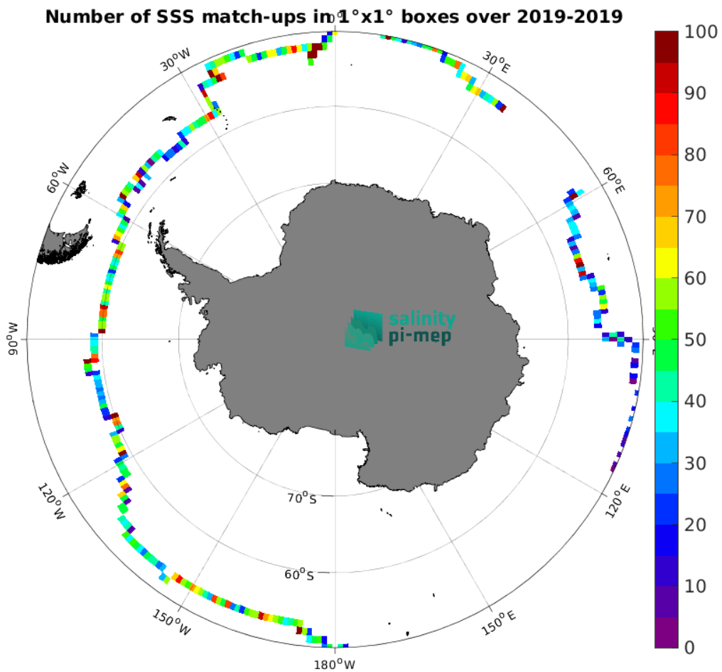
Figure 5: Number of SSS match-ups between Saildrone SSS and the SMOS SSS L4 v1 - Daily (CMEMS-CNR) SSS product for the Southern Ocean Pi-MEP region over 1^{\circ} \times 1^{\circ} boxes and for the full satellite product period.
