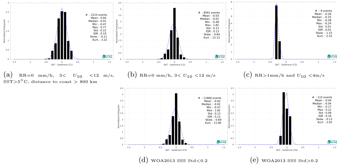
Figure 15: Normalized histogram of \Delta SSS (SMOS SSS L4 v1 - Daily (CMEMS-CNR) - Saldrone) for 5 different subdatasets corresponding to: RR=0 mm/h, 3 < U_{10} < 12 m/s, SST > 5°C, distance to coast > 800 km (a), RR=0 mm/h, 3 < U_{10} < 12 m/s (b), RR > 1mm/h and U_{10} < 4 m/s (c), WOA2013 SSS Std < 0.2 (d), WOA2013 SSS Std > 0.2 (e).
