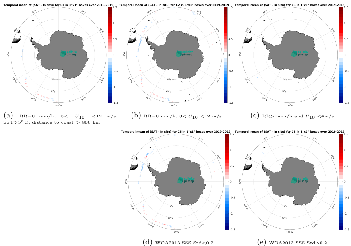
Figure 14: Temporal mean gridded over spatial boxes of size 1^\circ \times 1^\circ of \Delta SSS (SMOS SSS L4 v1 - Daily (CMEMS-CNR) - Sairdrone) for 5 different subdatasets corresponding to:RR=0 mm/h, 3 < U_{10} < 12 m/s, SST >5^\circ\text{C} , distance to coast > 800 km (a), RR=0 mm/h, 3 < U_{10} < 12 m/s (b), RR >1 mm/h and U_{10} < 4 m/s (c), WOA2013 SSS Std <0.2 (d), WOA2013 SSS Std >0.2 (e).
