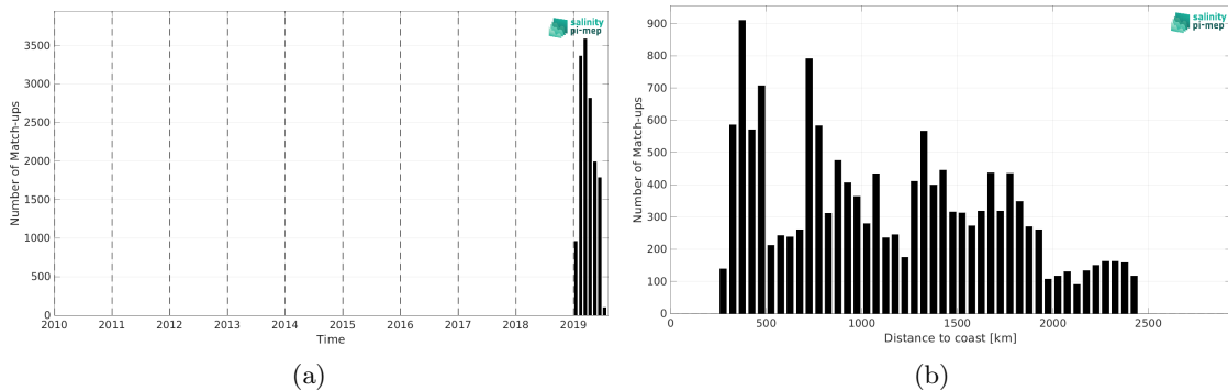
Figure 2: Number of match-ups between Saildrone and SMOS SSS L4 v1 - Daily (CMEMS-CNR) SSS as a function of time (a) and as function of the distance to coast (b) over the Southern Ocean Pi-MEP region and for the full satellite product period.
