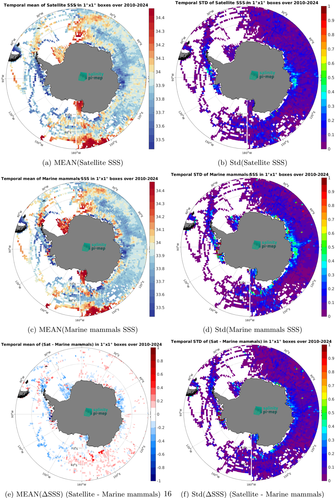
Figure 7: Temporal mean (left) and Std (right) of SSS from SMOS SSS L4 v1 - Daily (CMEMS-CNR) (top), Marine mammals (middle), and of \Delta SSS (Satellite - Marine mammals). Only match-up pairs are used to generate these maps.
