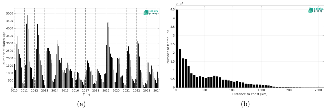
Figure 2: Number of match-ups between Marine mammals and SMOS SSS L4 v1 - Daily (CMEMS-CNR) SSS as a function of time (a) and as function of the distance to coast (b) over the Southern Ocean Pi-MEP region and for the full satellite product period.
