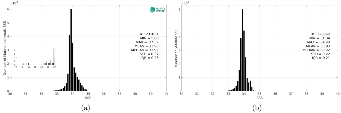
Figure 3: Histograms of SSS from Marine mammals (a) and SMOS SSS L4 v1 - Daily (CMEMS-CNR) (b) considering all match-up pairs per bins of 0.1 over the Southern Ocean Pi-MEP region and for the full satellite product period.
