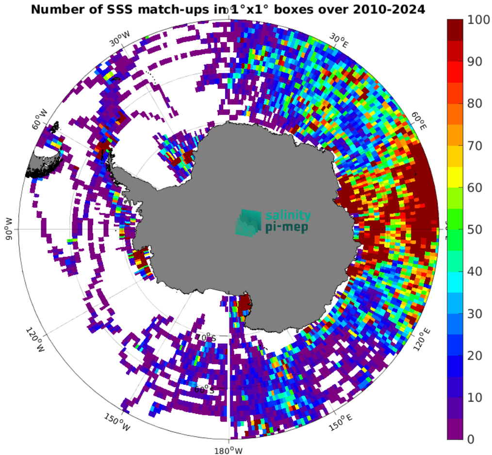
Figure 5: Number of SSS match-ups between Marine mammals SSS and the SMOS SSS L4 v1 - Daily (CMEMS-CNR) SSS product for the Southern Ocean Pi-MEP region over 1^\circ \times 1^\circ boxes and for the full satellite product period.
