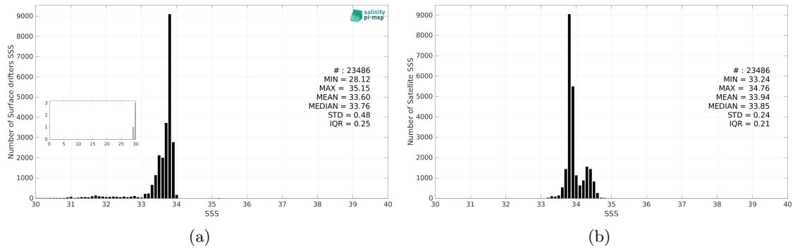
Figure 3: Histograms of SSS from Surface drifters (a) and SMOS SSS L4 v1 - Daily (CMEMS-CNR) (b) considering all match-up pairs per bins of 0.1 over the Southern Ocean Pi-MEP region and for the full satellite product period.
