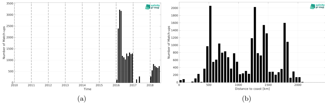
Figure 2: Number of match-ups between Surface drifters and SMOS SSS L4 v1 - Daily (CMEMS-CNR) SSS as a function of time (a) and as function of the distance to coast (b) over the Southern Ocean Pi-MEP region and for the full satellite product period.
