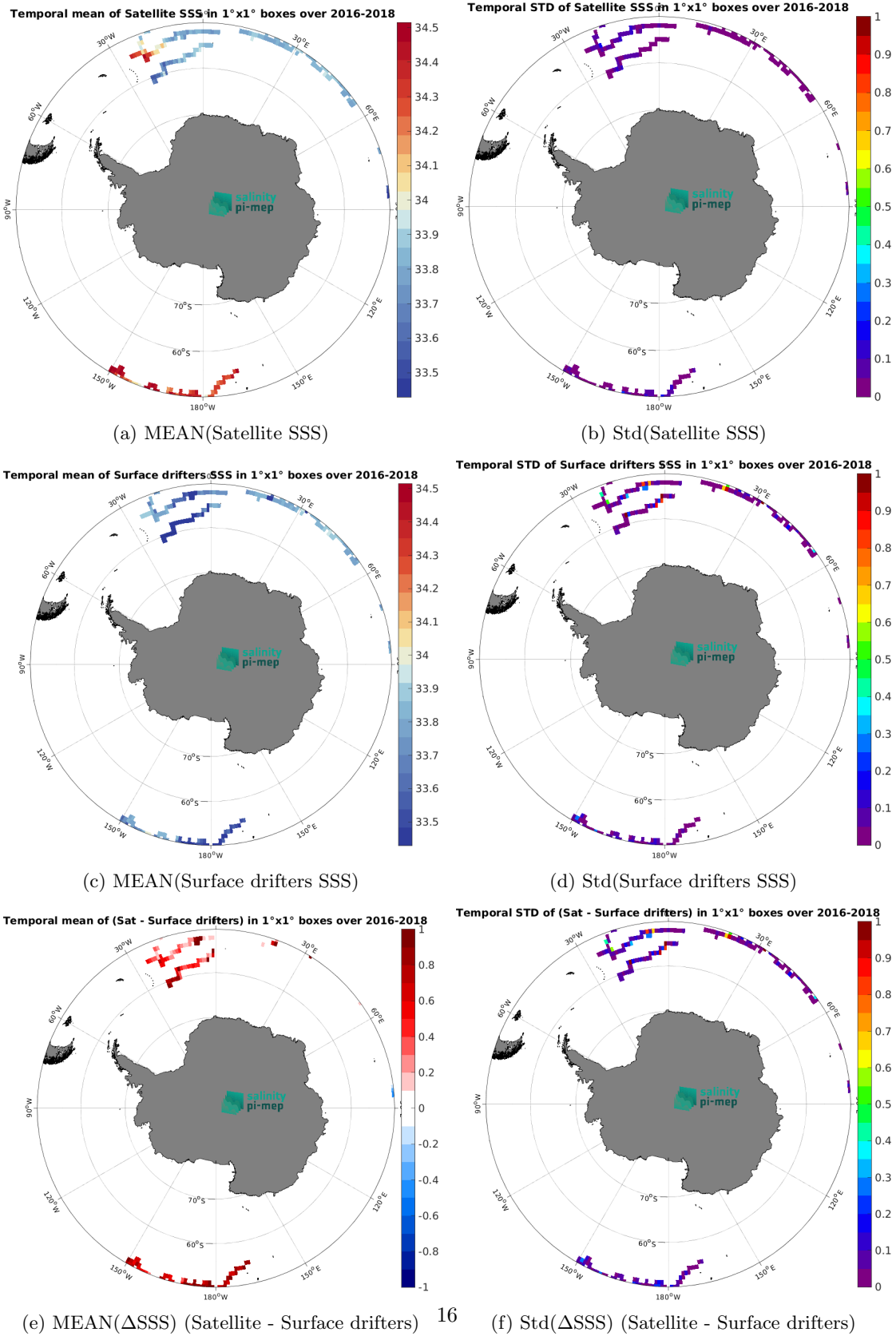
Figure 6: Temporal mean (left) and Std (right) of SSS from SMOS SSS L4 v1 - Daily (CMEMS-CNR) (top), Surface drifters (middle), and of \Delta SSS (Satellite - Surface drifters). Only match-up pairs are used to generate these maps.
