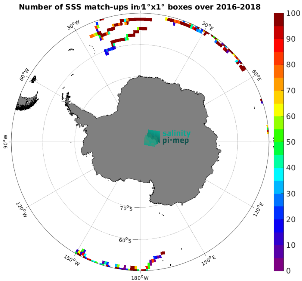
Figure 4: Number of SSS match-ups between Surface drifters SSS and the SMOS SSS L4 v1 - Daily (CMEMS-CNR) SSS product for the Southern Ocean Pi-MEP region over 1^\circ \times 1^\circ boxes and for the full satellite product period.
