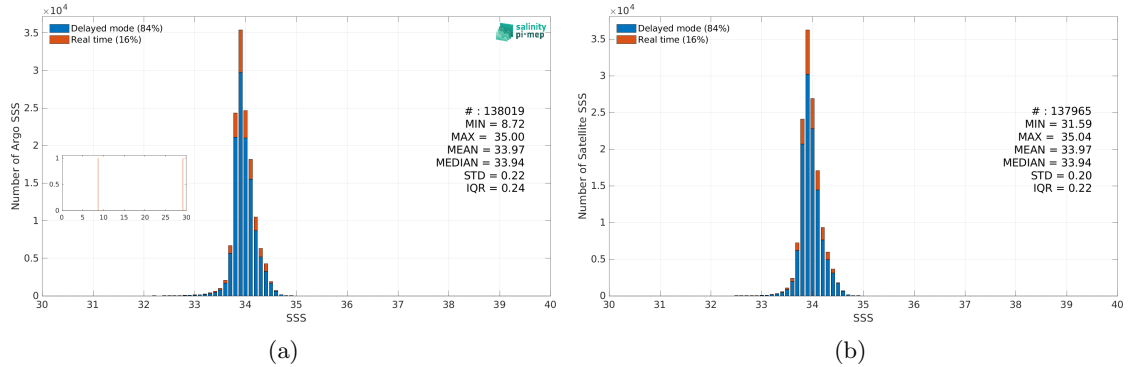
Figure 3: Histograms of SSS from Argo (a) and SMOS SSS L4 v1 - Daily (CMEMS-CNR) (b) considering all match-up pairs per bins of 0.1 over the Southern Ocean Pi-MEP region and for the full satellite product period.
