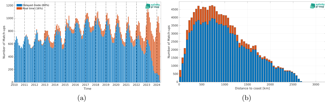
Figure 2: Number of match-ups between Argo and SMOS SSS L4 v1 - Daily (CMEMS-CNR) SSS as a function of time (a) and as function of the distance to coast (b) over the Southern Ocean Pi-MEP region and for the full satellite product period.
