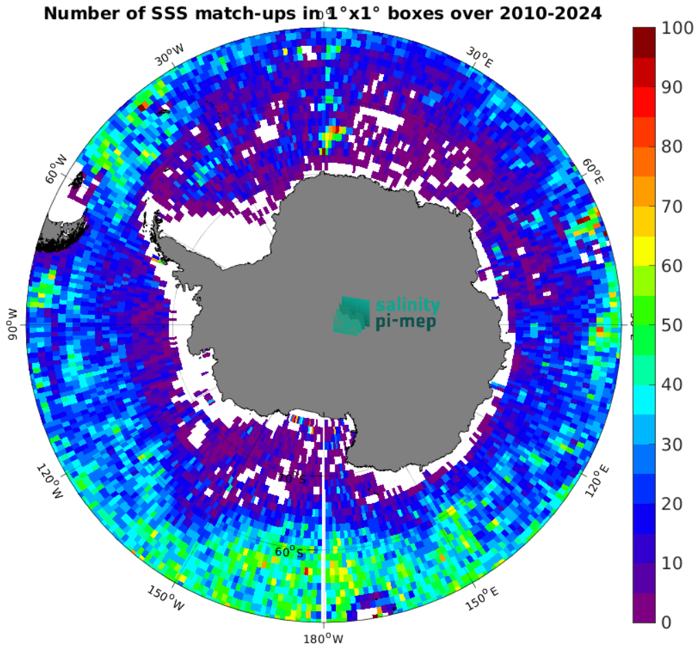
Figure 5: Number of SSS match-ups between Argo SSS and the SMOS SSS L4 v1 - Daily (CMEMS-CNR) SSS product for the Southern Ocean Pi-MEP region over 1^\circ \times 1^\circ boxes and for the full satellite product period.
