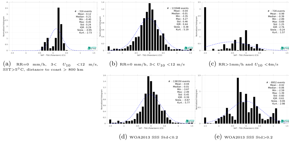
Figure 15: Normalized histogram of \Delta SSS (SMOS SSS L4 OI v346 - Weekly (CMEMS-CATDS-LOPS) - TSG (Polarstern)) for 5 different subdatasets corresponding to: RR=0 mm/h, 3 < U_{10} < 12 m/s, SST>5°C, distance to coast > 800 km (a), RR=0 mm/h, 3 < U_{10} < 12 m/s (b), RR>1mm/h and U_{10} < 4 m/s (c), WOA2013 SSS Std<0.2 (d), WOA2013 SSS Std>0.2 (e).
