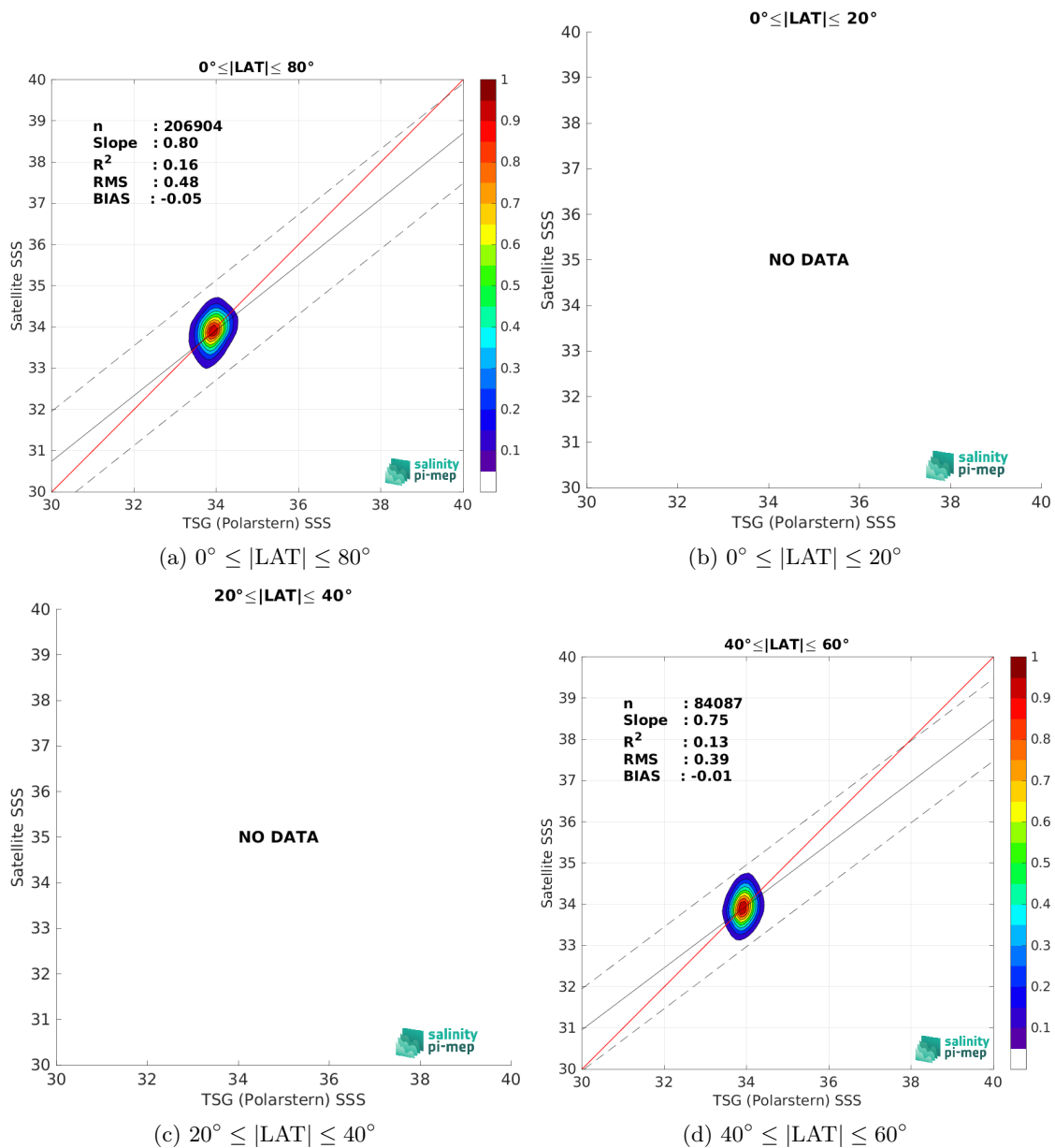
Figure 10: Contour maps of the concentration of SMOS SSS L4 OI v346 - Weekly (CMEMS-CATDS-LOPS) SSS (y-axis) versus TSG (Polarstern) SSS (x-axis) at match-up pairs for different latitude bands. For each plot, the red line shows x=y . The black thin and dashed lines indicate a linear fit through the data cloud and the \pm 95\% confidence levels, respectively. The number match-up pairs n , the slope and R^2 coefficient of the linear fit, the root mean square (RMS) and the mean bias between satellite and in situ data are indicated for each latitude band in each plots.
