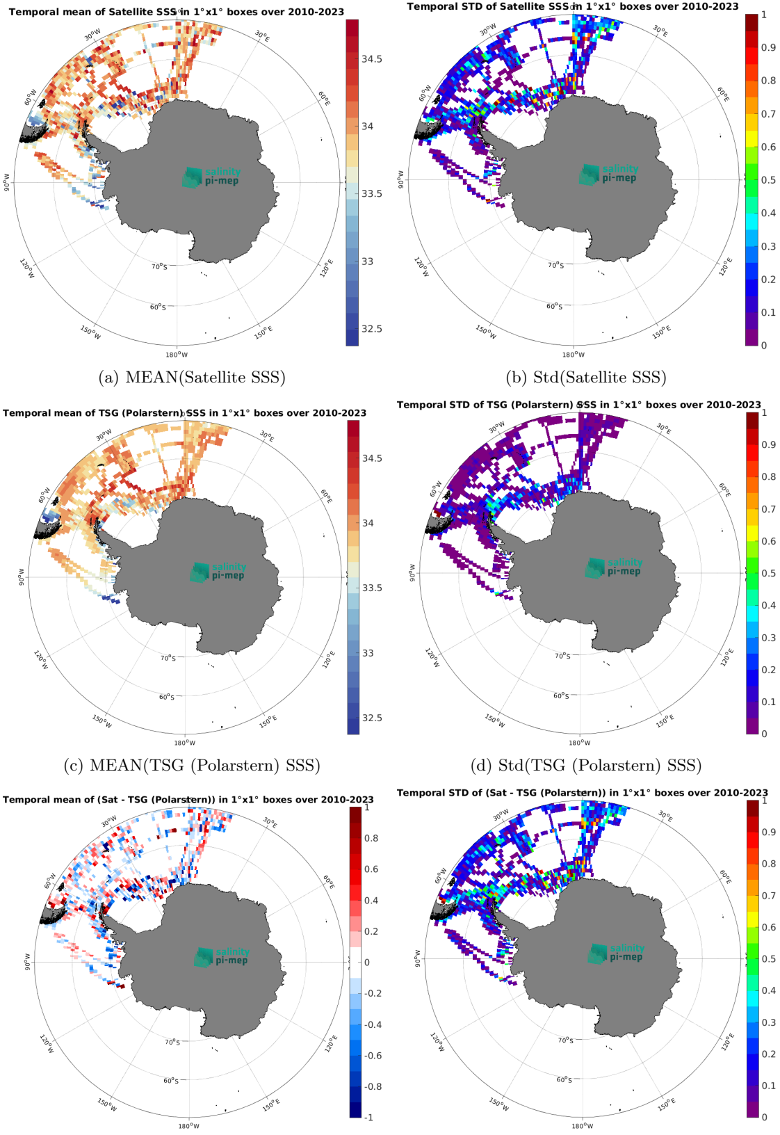
Figure 7: Temporal mean (left) and Std (right) of SSS from SMOS SSS L4 OI v346 - Weekly (CMEMS-CATDS-LOPS) (top), TSG (Polarstern) (middle), and of \Delta SSS (Satellite - TSG (Polarstern)). Only match-up pairs are used to generate these maps.
