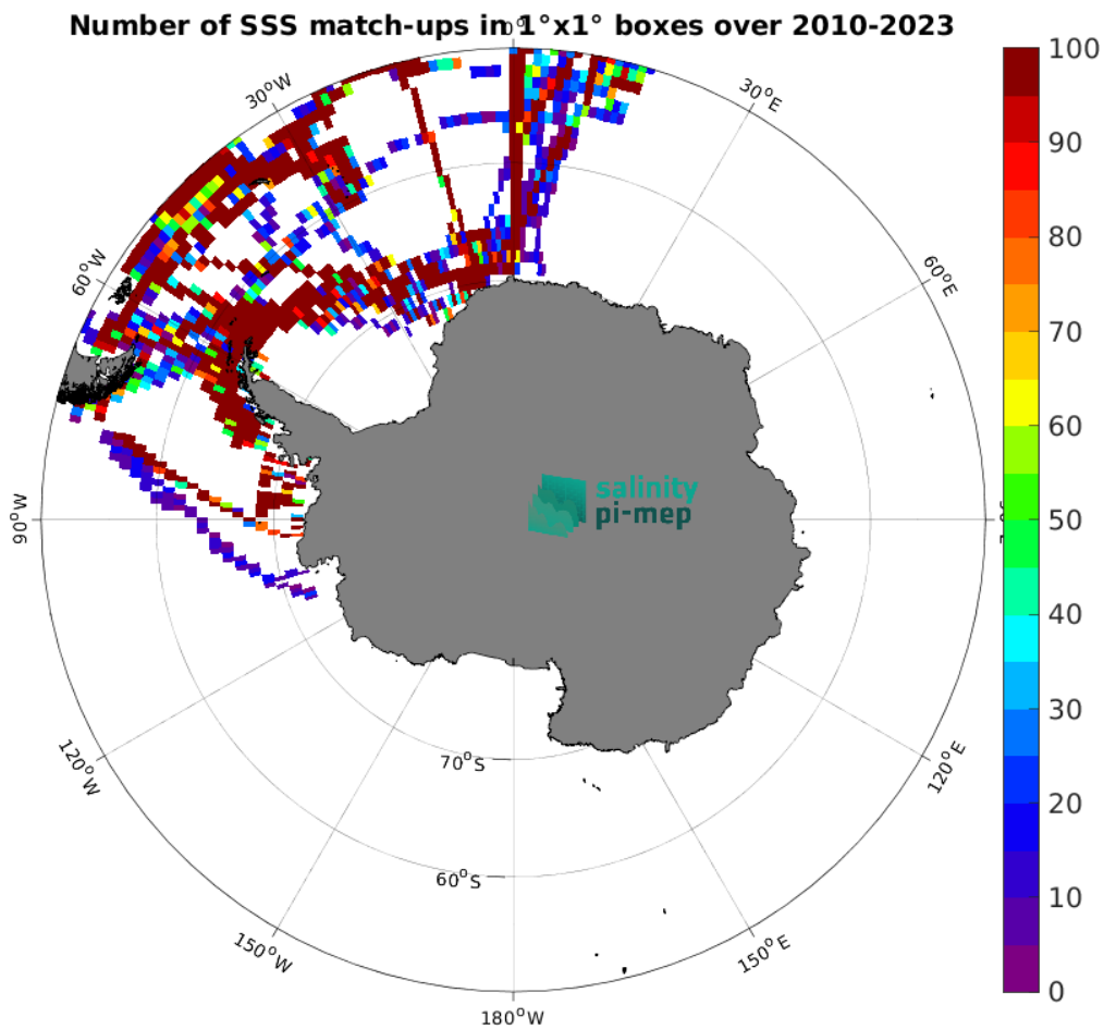
Figure 5: Number of SSS match-ups between TSG (Polarstern) SSS and the SMOS SSS L4 OI v346 - Weekly (CMEMS-CATDS-LOPS) SSS product for the Southern Ocean Pi-MEP region over 1^\circ \times 1^\circ boxes and for the full satellite product period.
