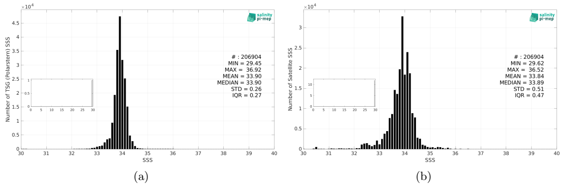
Figure 3: Histograms of SSS from TSG (Polarstern) (a) and SMOS SSS L4 OI v346 - Weekly (CMEMS-CATDS-LOPS) (b) considering all match-up pairs per bins of 0.1 over the Southern Ocean Pi-MEP region and for the full satellite product period.
