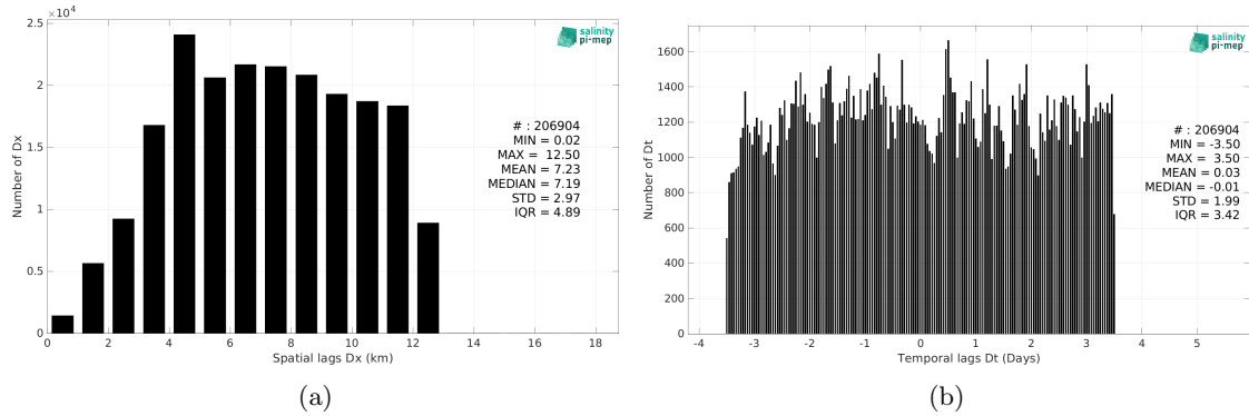
Figure 6: Histograms of the spatial (a) and temporal (b) lags between the location/time of the TSG (Polarstern) measurement and the date of the corresponding SMOS SSS L4 OI v346 - Weekly (CMEMS-CATDS-LOPS) SSS pixel.
