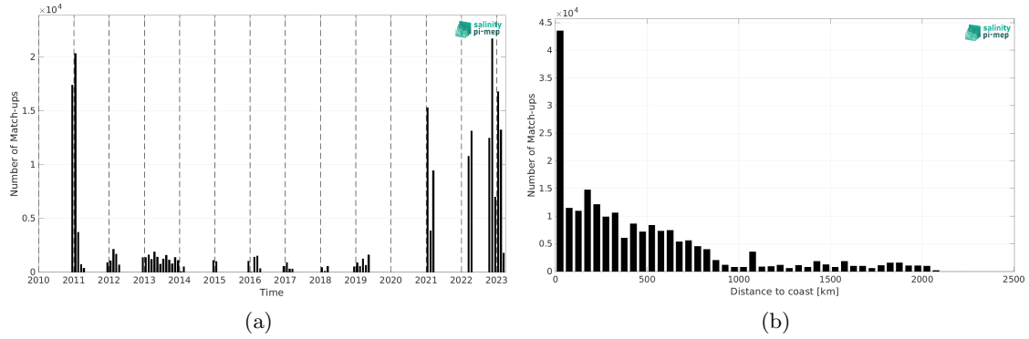
Figure 2: Number of match-ups between TSG (Polarstern) and SMOS SSS L4 OI v346 - Weekly (CMEMS-CATDS-LOPS) SSS as a function of time (a) and as function of the distance to coast (b) over the Southern Ocean Pi-MEP region and for the full satellite product period.
