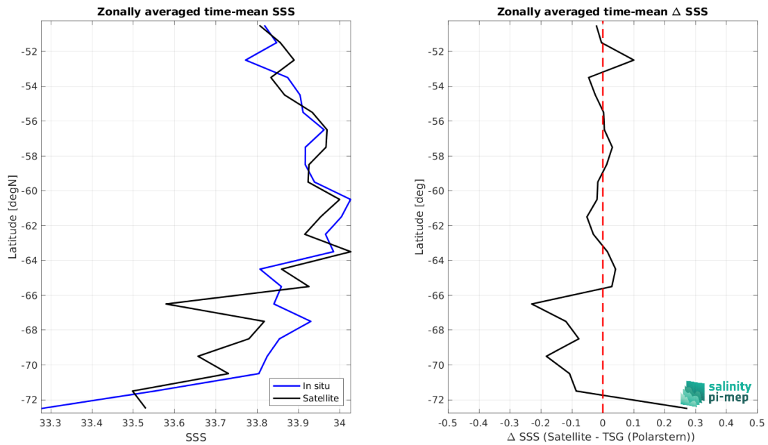
Figure 9: Left panel: Zonal mean SSS from SMOS SSS L4 OI v346 - Weekly (CMEMS-CATDS-LOPS) satellite product (black) and from TSG (Polarstern) (blue). Right panel: Zonal mean of \Delta SSS (Satellite - TSG (Polarstern)) for all the collected Pi-MEP match-up pairs estimated over the full satellite product period.
