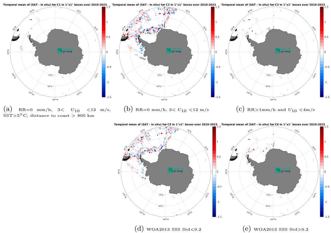
Figure 14: Temporal mean gridded over spatial boxes of size 1^\circ \times 1^\circ of \Delta SSS (SMOS SSS L4 OI v346 - Weekly (CMEMS-CATDS-LOPS) - TSG (Polarstern)) for 5 different subdatasets corresponding to:RR=0 mm/h, 3 < U_{10} < 12 m/s, SST>5°C, distance to coast > 800 km (a), RR=0 mm/h, 3 < U_{10} < 12 m/s (b), RR>1mm/h and U_{10} < 4 m/s (c), WOA2013 SSS Std<0.2 (d), WOA2013 SSS Std>0.2 (e).
