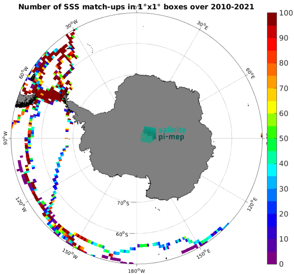
Figure 5: Number of SSS match-ups between TSG (GOSUD-Sailing-ship) SSS and the SMOS SSS L4 OI v346 - Weekly (CMEMS-CATDS-LOPS) SSS product for the Southern Ocean Pi-MEP region over 1^{\circ} \times 1^{\circ} boxes and for the full satellite product period.
