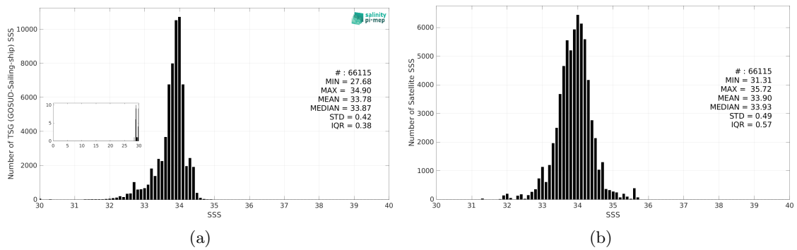
Figure 3: Histograms of SSS from TSG (GOSUD-Sailing-ship) (a) and SMOS SSS L4 OI v346 - Weekly (CMEMS-CATDS-LOPS) (b) considering all match-up pairs per bins of 0.1 over the Southern Ocean Pi-MEP region and for the full satellite product period.
