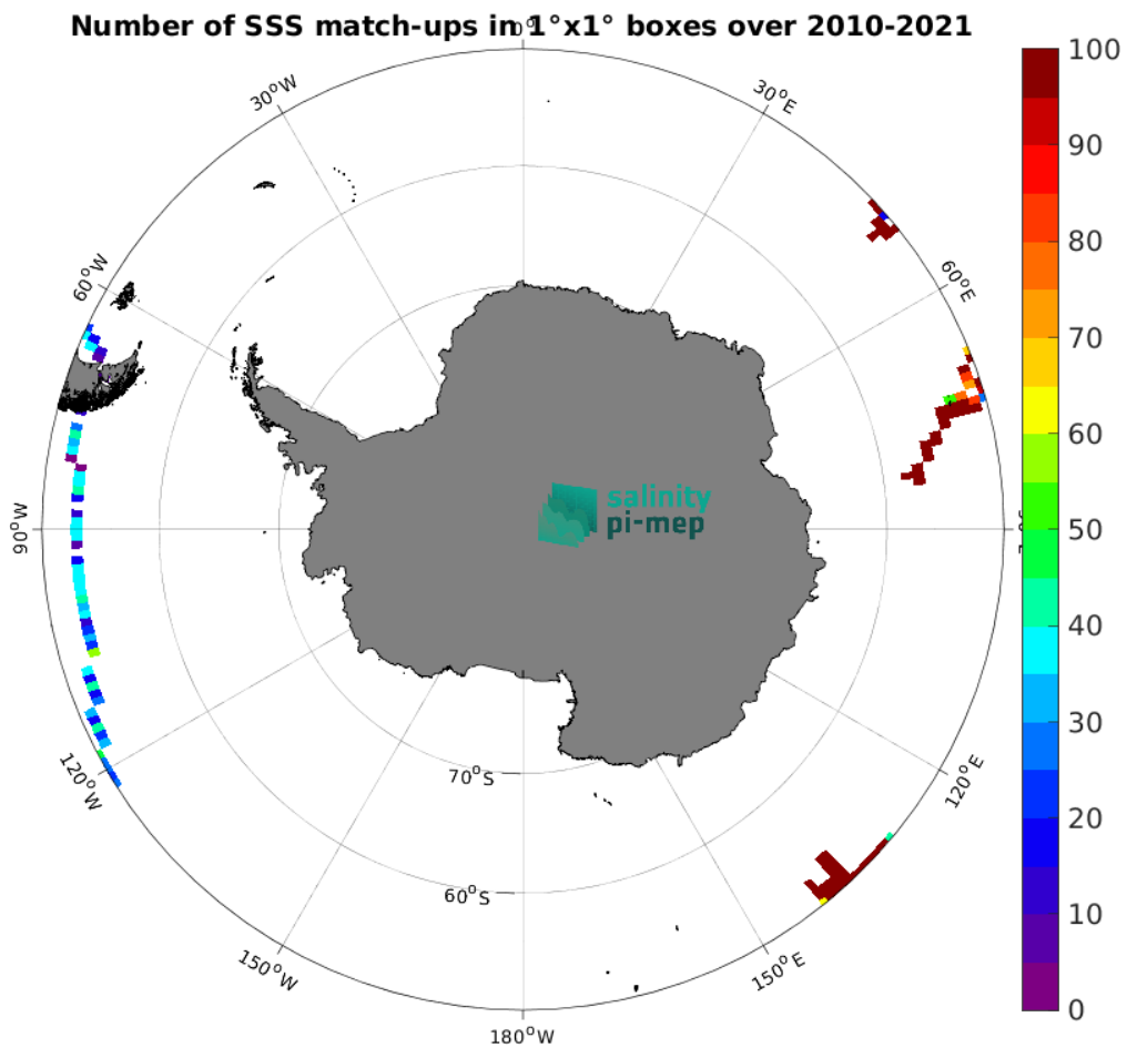
Figure 5: Number of SSS match-ups between TSG (GOSUD-Research-vessel) SSS and the SMOS SSS L4 OI v346 - Weekly (CMEMS-CATDS-LOPS) SSS product for the Southern Ocean Pi-MEP region over 1^\circ \times 1^\circ boxes and for the full satellite product period.
