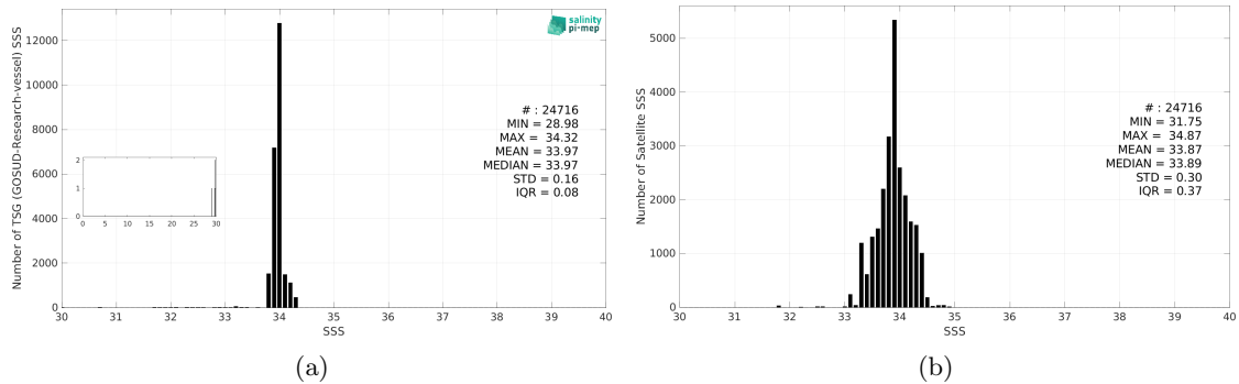
Figure 3: Histograms of SSS from TSG (GOSUD-Research-vessel) (a) and SMOS SSS L4 OI v346 - Weekly (CMEMS-CATDS-LOPS) (b) considering all match-up pairs per bins of 0.1 over the Southern Ocean Pi-MEP region and for the full satellite product period.
