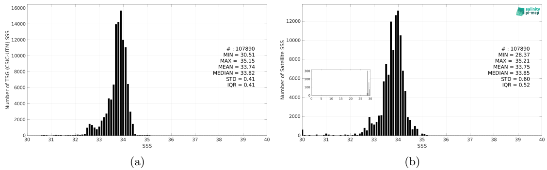
Figure 3: Histograms of SSS from TSG (CSIC-UTM) (a) and SMOS SSS L4 OI v346 - Weekly (CMEMS-CATDS-LOPS) (b) considering all match-up pairs per bins of 0.1 over the Southern Ocean Pi-MEP region and for the full satellite product period.
