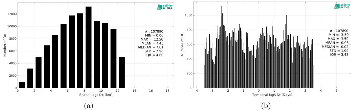
Figure 6: Histograms of the spatial (a) and temporal (b) lags between the location/time of the TSG (CSIC-UTM) measurement and the date of the corresponding SMOS SSS L4 OI v346 - Weekly (CMEMS-CATDS-LOPS) SSS pixel.
