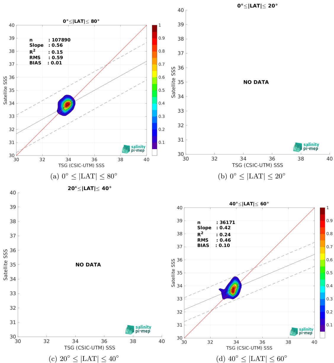
Figure 10: Contour maps of the concentration of SMOS SSS L4 OI v346 - Weekly (CMEMS-CATDS-LOPS) SSS (y-axis) versus TSG (CSIC-UTM) SSS (x-axis) at match-up pairs for different latitude bands. For each plot, the red line shows x=y . The black thin and dashed lines indicate a linear fit through the data cloud and the \pm 95\% confidence levels, respectively. The number match-up pairs n , the slope and R^2 coefficient of the linear fit, the root mean square (RMS) and the mean bias between satellite and in situ data are indicated for each latitude band in each plots.
