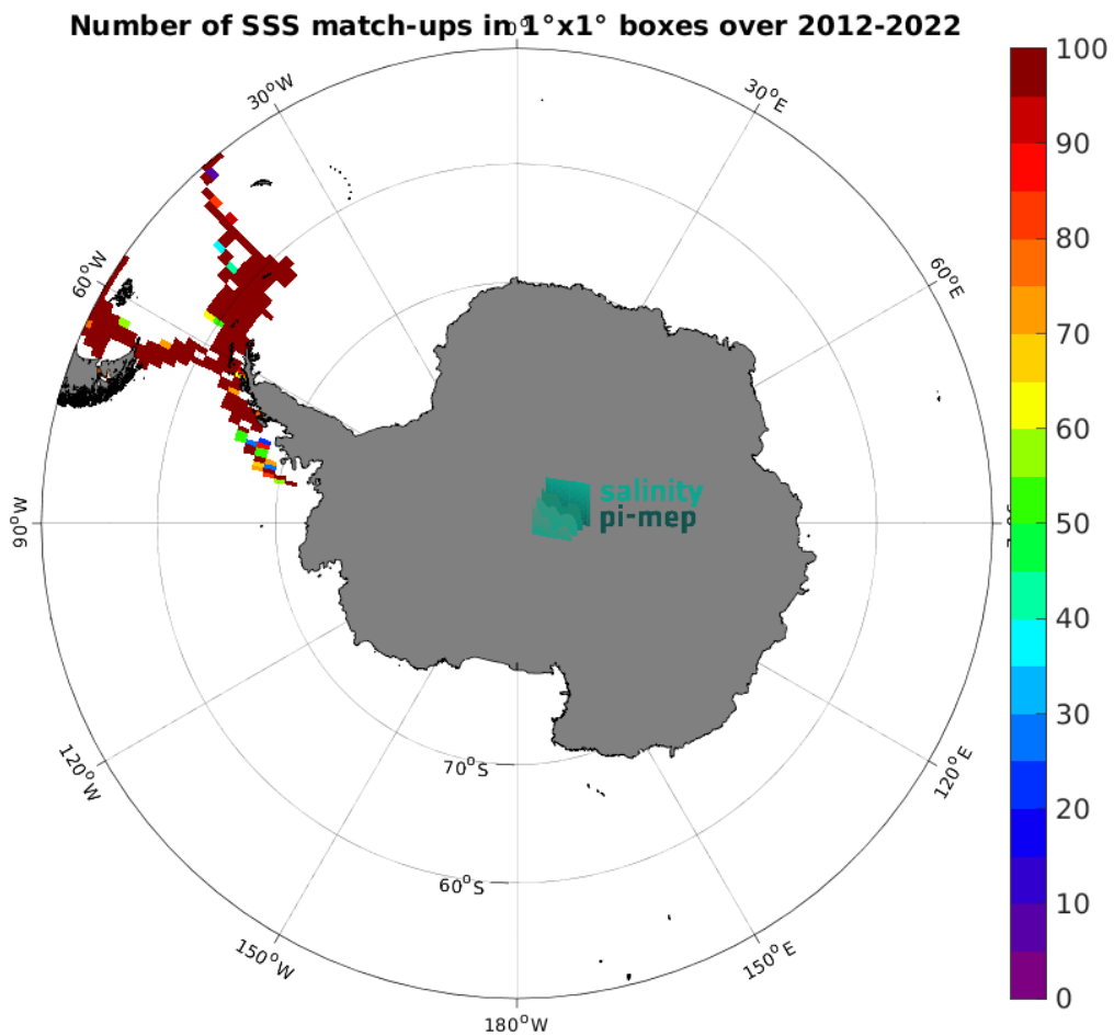
Figure 5: Number of SSS match-ups between TSG (CSIC-UTM) SSS and the SMOS SSS L4 OI v346 - Weekly (CMEMS-CATDS-LOPS) SSS product for the Southern Ocean Pi-MEP region over 1^\circ \times 1^\circ boxes and for the full satellite product period.
