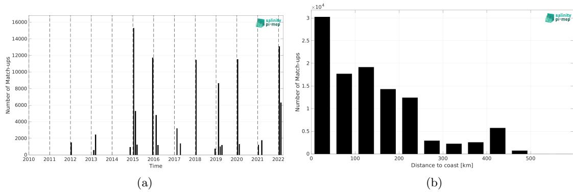
Figure 2: Number of match-ups between TSG (CSIC-UTM) and SMOS SSS L4 OI v346 - Weekly (CMEMS-CATDS-LOPS) SSS as a function of time (a) and as function of the distance to coast (b) over the Southern Ocean Pi-MEP region and for the full satellite product period.
