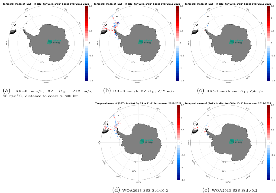
Figure 14: Temporal mean gridded over spatial boxes of size 1^\circ \times 1^\circ of \Delta SSS (SMOS SSS L4 OI v346 - Weekly (CMEMS-CATDS-LOPS) - TSG (CSIC-UTM)) for 5 different subdatasets corresponding to:RR=0 mm/h, 3 < U_{10} < 12 m/s, SST >5^\circ\text{C} , distance to coast > 800 km (a), RR=0 mm/h, 3 < U_{10} < 12 m/s (b), RR >1 mm/h and U_{10} < 4 m/s (c), WOA2013 SSS Std <0.2 (d), WOA2013 SSS Std >0.2 (e).
