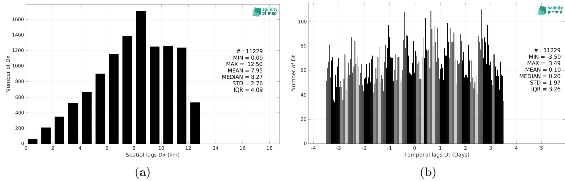
Figure 6: Histograms of the spatial (a) and temporal (b) lags between the location/time of the Saildrone measurement and the date of the corresponding SMOS SSS L4 OI v346 - Weekly (CMEMS-CATDS-LOPS) SSS pixel.
