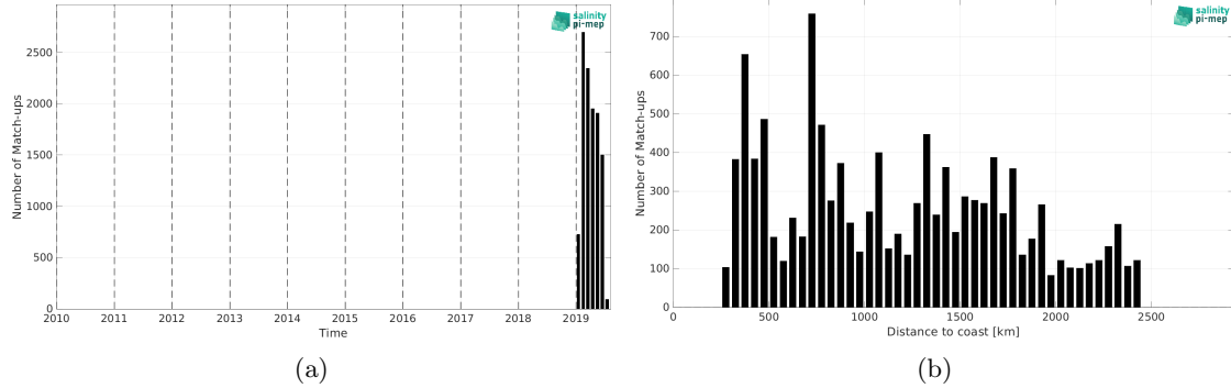
Figure 2: Number of match-ups between Saildrone and SMOS SSS L4 OI v346 - Weekly (CMEMS-CATDS-LOPS) SSS as a function of time (a) and as function of the distance to coast (b) over the Southern Ocean Pi-MEP region and for the full satellite product period.
