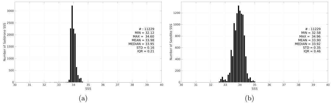
Figure 3: Histograms of SSS from Saildrone (a) and SMOS SSS L4 OI v346 - Weekly (CMEMS-CATDS-LOPS) (b) considering all match-up pairs per bins of 0.1 over the Southern Ocean Pi-MEP region and for the full satellite product period.
