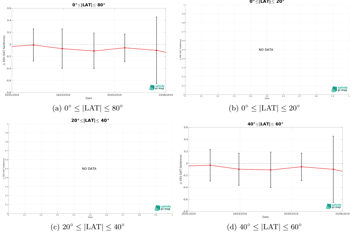
Figure 11: Monthly median (red curves) of \Delta SSS (Satellite - Sairdrone ) and \pm 1 Std (black vertical thick bars) as function of time for all the collected Pi-MEP match-up pairs estimated over the Southern Ocean Pi-MEP region and for the full satellite product period are shown for different latitude bands: (a) 80^\circ\text{S}-80^\circ\text{N} , (b) 20^\circ\text{S}-20^\circ\text{N} , (c) 40^\circ\text{S}-20^\circ\text{S} and 20^\circ\text{N}-40^\circ\text{N} and (d) 60^\circ\text{S}-40^\circ\text{S} and 40^\circ\text{N}-60^\circ\text{N} .
