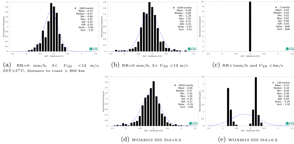
Figure 15: Normalized histogram of \Delta SSS (SMOS SSS L4 OI v346 - Weekly (CMEMS-CATDS-LOPS) - Saldrone) for 5 different subdatasets corresponding to: RR=0 mm/h, 3 < U_{10} < 12 m/s, SST > 5°C, distance to coast > 800 km (a), RR=0 mm/h, 3 < U_{10} < 12 m/s (b), RR > 1mm/h and U_{10} < 4 m/s (c), WOA2013 SSS Std < 0.2 (d), WOA2013 SSS Std > 0.2 (e).
