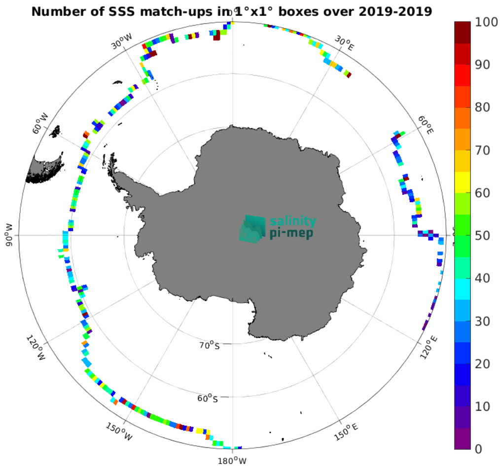
Figure 5: Number of SSS match-ups between Saildrone SSS and the SMOS SSS L4 OI v346 - Weekly (CMEMS-CATDS-LOPS) SSS product for the Southern Ocean Pi-MEP region over 1^\circ \times 1^\circ boxes and for the full satellite product period.
