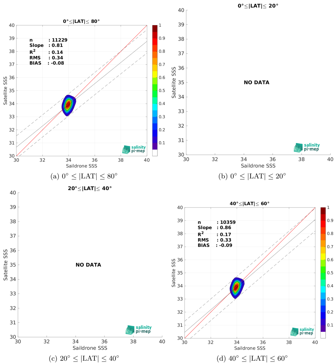
Figure 10: Contour maps of the concentration of SMOS SSS L4 OI v346 - Weekly (CMEMS-CATDS-LOPS) SSS (y-axis) versus Saildrone SSS (x-axis) at match-up pairs for different latitude bands. For each plot, the red line shows x=y . The black thin and dashed lines indicate a linear fit through the data cloud and the \pm 95\% confidence levels, respectively. The number match-up pairs n , the slope and R^2 coefficient of the linear fit, the root mean square (RMS) and the mean bias between satellite and in situ data are indicated for each latitude band in each plots.
