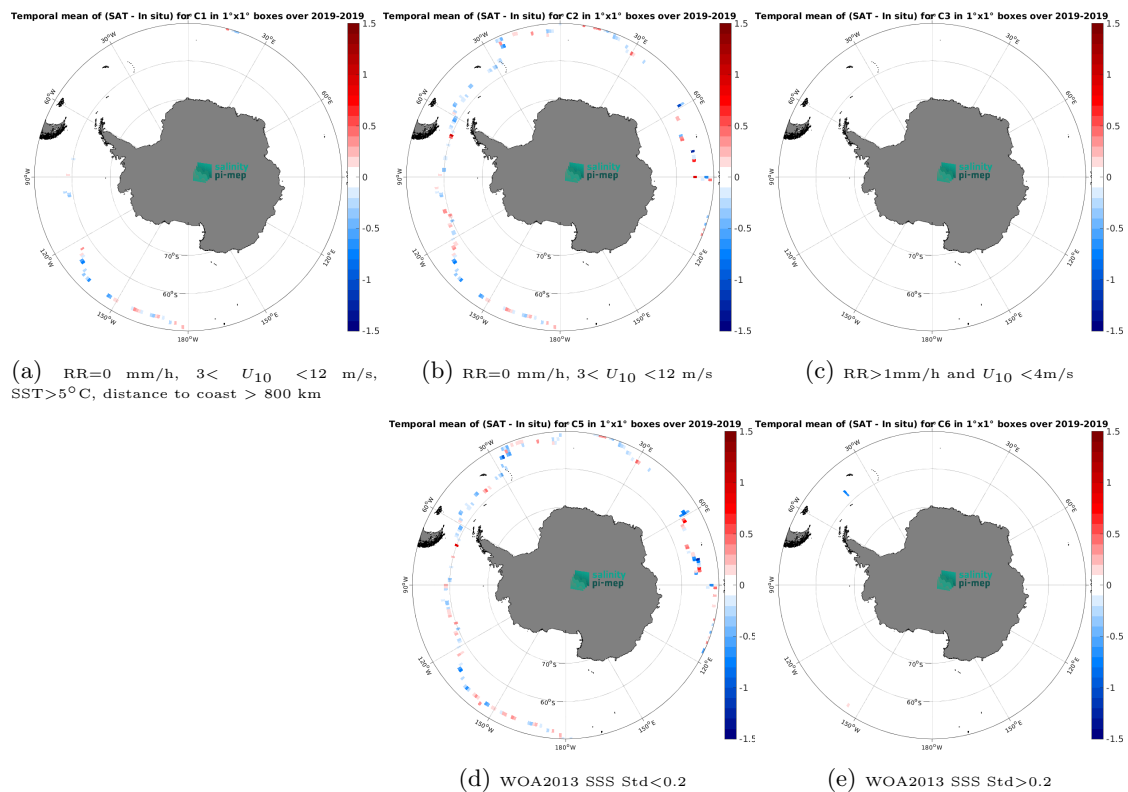
Figure 14: Temporal mean gridded over spatial boxes of size 1^\circ \times 1^\circ of \Delta\text{SSS} (SMOS SSS L4 OI v346 - Weekly (CMEMS-CATDS-LOPS) - Saildrone) for 5 different subdatasets corresponding to:RR=0 mm/h, 3 < U_{10} < 12 m/s, SST>5°C, distance to coast > 800 km (a), RR=0 mm/h, 3 < U_{10} < 12 m/s (b), RR>1mm/h and U_{10} < 4 m/s (c), WOA2013 SSS Std<0.2 (d), WOA2013 SSS Std>0.2 (e).
