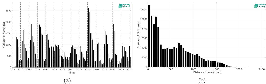
Figure 2: Number of match-ups between Marine mammals and SMOS SSS L4 OI v346 - Weekly (CMEMS-CATDS-LOPS) SSS as a function of time (a) and as function of the distance to coast (b) over the Southern Ocean Pi-MEP region and for the full satellite product period.
