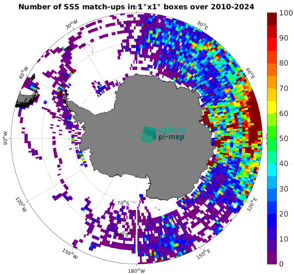
Figure 5: Number of SSS match-ups between Marine mammals SSS and the SMOS SSS L4 OI v346 - Weekly (CMEMS-CATDS-LOPS) SSS product for the Southern Ocean Pi-MEP region over 1^\circ \times 1^\circ boxes and for the full satellite product period.
