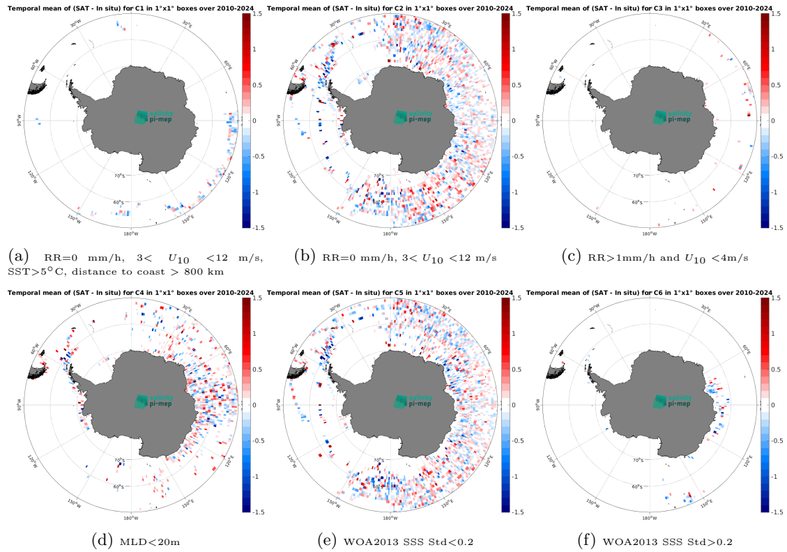
Figure 14: Temporal mean gridded over spatial boxes of size 1^\circ \times 1^\circ of \Delta SSS (SMOS SSS L4 OI v346 - Weekly (CMEMS-CATDS-LOPS) - Marine mammals) for 6 different subdatasets corresponding to:RR=0 mm/h, 3 < U_{10} < 12 m/s, SST>5°C, distance to coast > 800 km (a), RR=0 mm/h, 3 < U_{10} < 12 m/s (b), RR>1mm/h and U_{10} < 4 m/s (c),MLD<20m (d),WOA2013 SSS Std<0.2 (e),WOA2013 SSS Std>0.2 (f).
