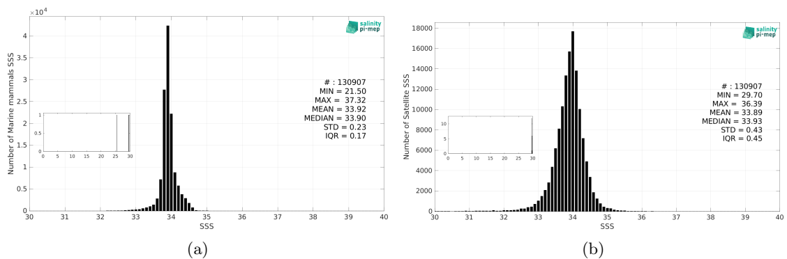
Figure 3: Histograms of SSS from Marine mammals (a) and SMOS SSS L4 OI v346 - Weekly (CMEMS-CATDS-LOPS) (b) considering all match-up pairs per bins of 0.1 over the Southern Ocean Pi-MEP region and for the full satellite product period.
