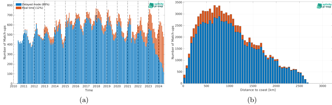
Figure 2: Number of match-ups between Argo and SMOS SSS L4 OI v346 - Weekly (CMEMS-CATDS-LOPS) SSS as a function of time (a) and as function of the distance to coast (b) over the Southern Ocean Pi-MEP region and for the full satellite product period.
