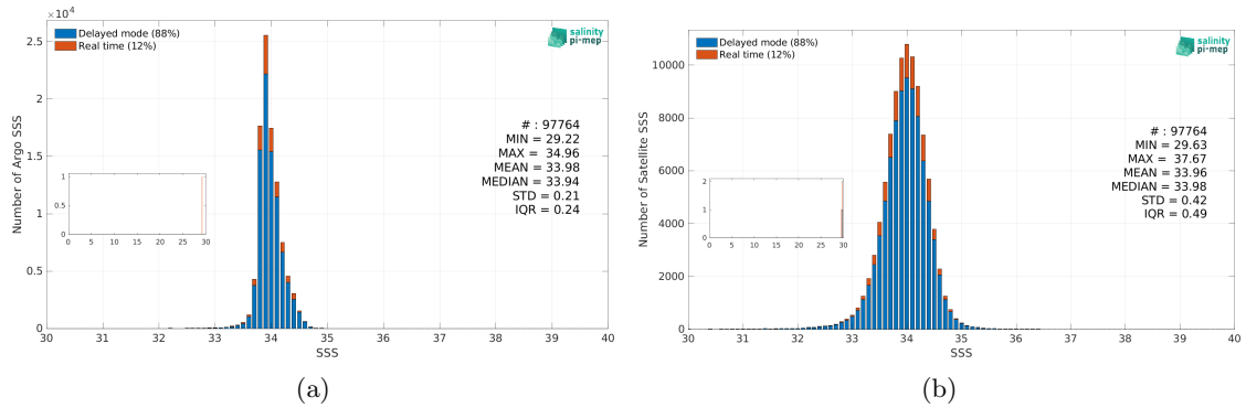
Figure 3: Histograms of SSS from Argo (a) and SMOS SSS L4 OI v346 - Weekly (CMEMS-CATDS-LOPS) (b) considering all match-up pairs per bins of 0.1 over the Southern Ocean Pi-MEP region and for the full satellite product period.
