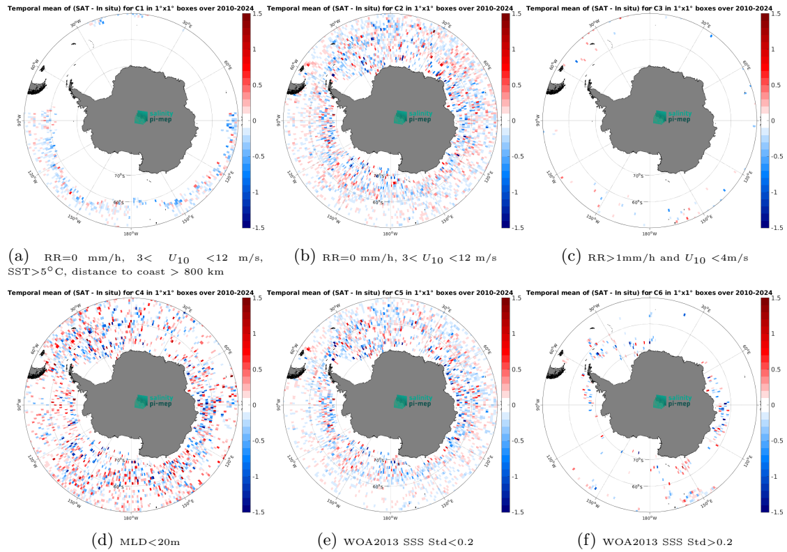
Figure 14: Temporal mean gridded over spatial boxes of size 1^\circ \times 1^\circ of \Delta SSS (SMOS SSS L4 OI v346 - Weekly (CMEMS-CATDS-LOPS) - Argo) for 6 different subdatasets corresponding to:RR=0 mm/h, 3 < U_{10} < 12 m/s, SST>5°C, distance to coast > 800 km (a), RR=0 mm/h, 3 < U_{10} < 12 m/s (b), RR>1mm/h and U_{10} < 4 m/s (c),MLD<20m (d),WOA2013 SSS Std<0.2 (e),WOA2013 SSS Std>0.2 (f).
