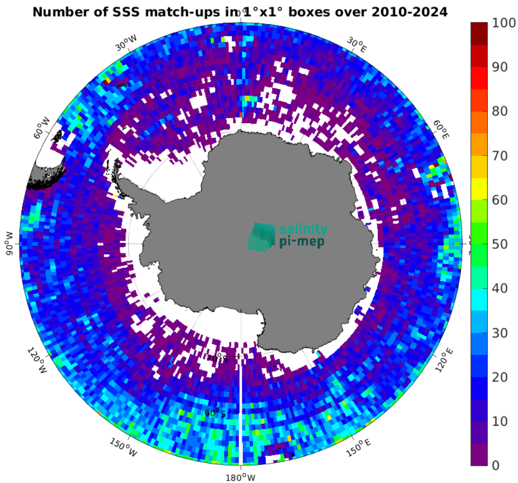
Figure 5: Number of SSS match-ups between Argo SSS and the SMOS SSS L4 OI v346 - Weekly (CMEMS-CATDS-LOPS) SSS product for the Southern Ocean Pi-MEP region over 1^{\circ} \times 1^{\circ} boxes and for the full satellite product period.
