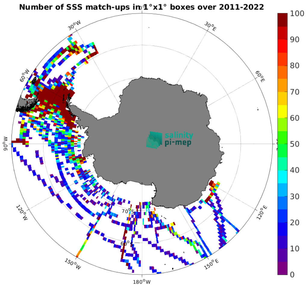
Figure 4: Number of SSS match-ups between TSG (SAMOS) SSS and the SMOS SSS L4 OI v342 - Weekly (CMEMS-CATDS-LOPS) SSS product for the Southern Ocean Pi-MEP region over 1^{\circ} \times 1^{\circ} boxes and for the full satellite product period.
