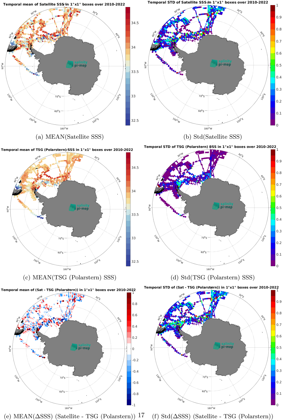
Figure 6: Temporal mean (left) and Std (right) of SSS from SMOS SSS L4 OI v342 - Weekly (CMEMS-CATDS-LOPS) (top), TSG (Polarstern) (middle), and of \Delta SSS (Satellite - TSG (Polarstern)). Only match-up pairs are used to generate these maps.
