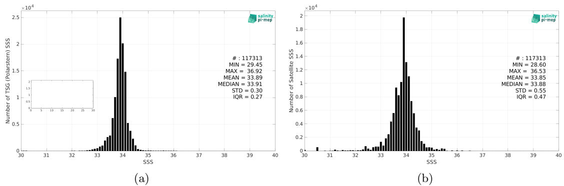
Figure 2: Histograms of SSS from TSG (Polarstern) (a) and SMOS SSS L4 OI v342 - Weekly (CMEMS-CATDS-LOPS) (b) considering all match-up pairs per bins of 0.1 over the Southern Ocean Pi-MEP region and for the full satellite product period.
