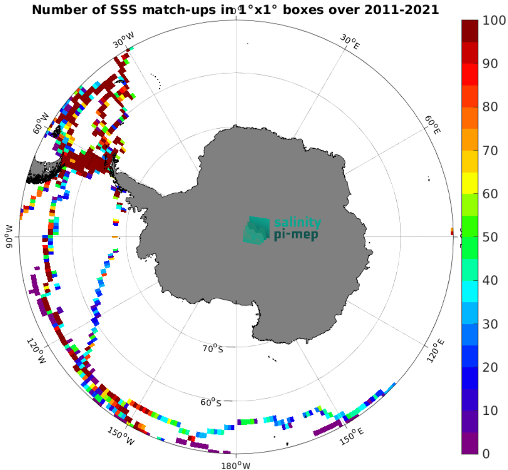
Figure 4: Number of SSS match-ups between TSG (GOSUD-Sailing-ship) SSS and the SMOS SSS L4 OI v342 - Weekly (CMEMS-CATDS-LOPS) SSS product for the Southern Ocean Pi-MEP region over 1^\circ \times 1^\circ boxes and for the full satellite product period.
