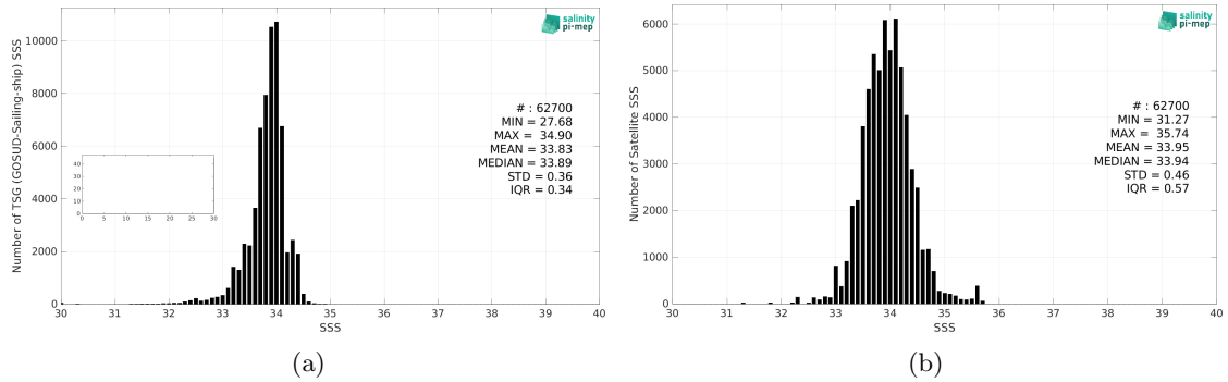
Figure 2: Histograms of SSS from TSG (GOSUD-Sailing-ship) (a) and SMOS SSS L4 OI v342 - Weekly (CMEMS-CATDS-LOPS) (b) considering all match-up pairs per bins of 0.1 over the Southern Ocean Pi-MEP region and for the full satellite product period.
