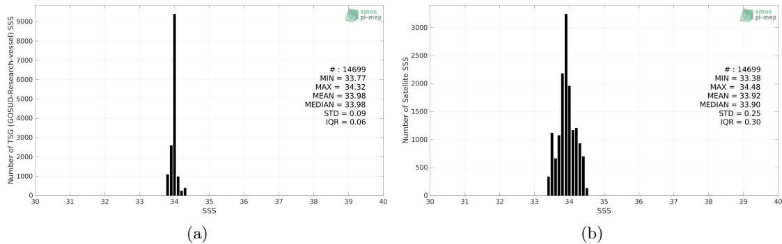
Figure 2: Histograms of SSS from TSG (GOSUD-Research-vessel) (a) and SMOS SSS L4 OI v342 - Weekly (CMEMS-CATDS-LOPS) (b) considering all match-up pairs per bins of 0.1 over the Southern Ocean Pi-MEP region and for the full satellite product period.
