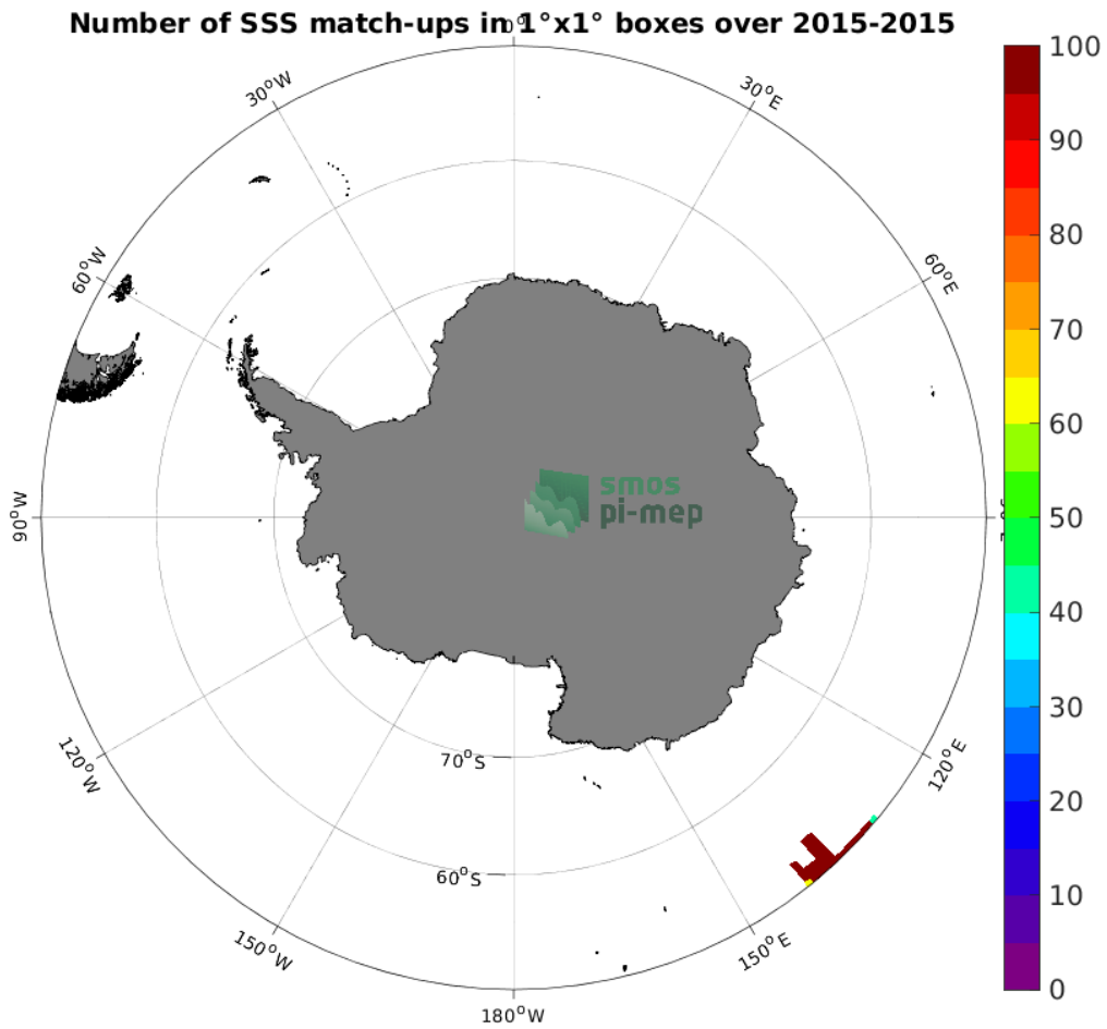
Figure 4: Number of SSS match-ups between TSG (GOSUD-Research-vessel) SSS and the SMOS SSS L4 OI v342 - Weekly (CMEMS-CATDS-LOPS) SSS product for the Southern Ocean Pi-MEP region over 1^\circ \times 1^\circ boxes and for the full satellite product period.
