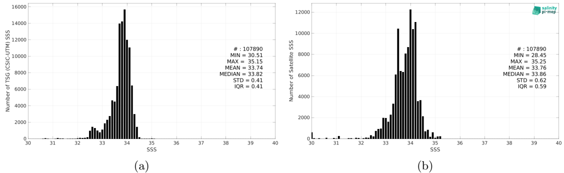
Figure 2: Histograms of SSS from TSG (CSIC-UTM) (a) and SMOS SSS L4 OI v342 - Weekly (CMEMS-CATDS-LOPS) (b) considering all match-up pairs per bins of 0.1 over the Southern Ocean Pi-MEP region and for the full satellite product period.
