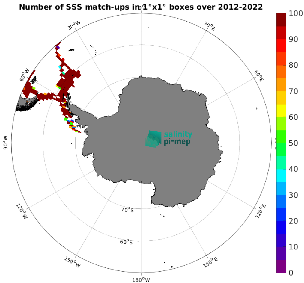
Figure 4: Number of SSS match-ups between TSG (CSIC-UTM) SSS and the SMOS SSS L4 OI v342 - Weekly (CMEMS-CATDS-LOPS) SSS product for the Southern Ocean Pi-MEP region over 1^{\circ} \times 1^{\circ} boxes and for the full satellite product period.
