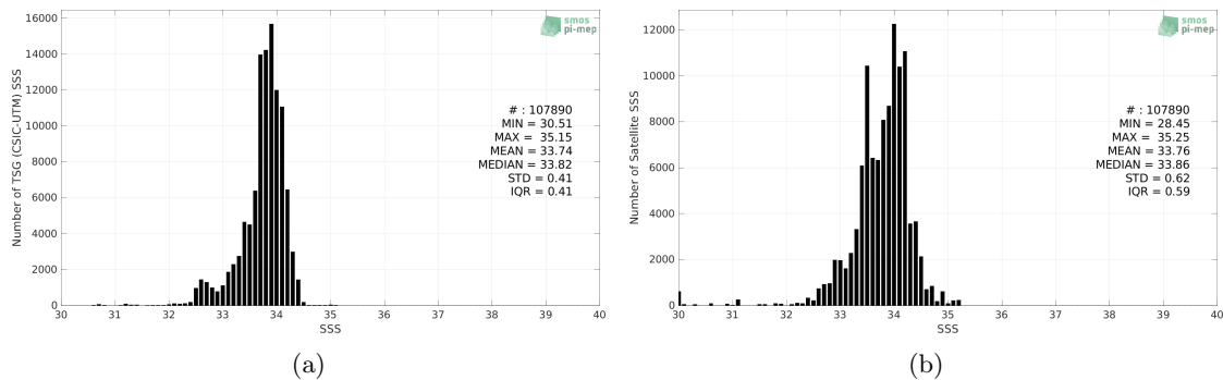
Figure 2: Histograms of SSS from TSG (CSIC-UTM) (a) and SMOS SSS L4 OI v342 - Weekly (CMEMS-CATDS-LOPS) (b) considering all match-up pairs per bins of 0.1 over the Southern Ocean Pi-MEP region and for the full satellite product period.
