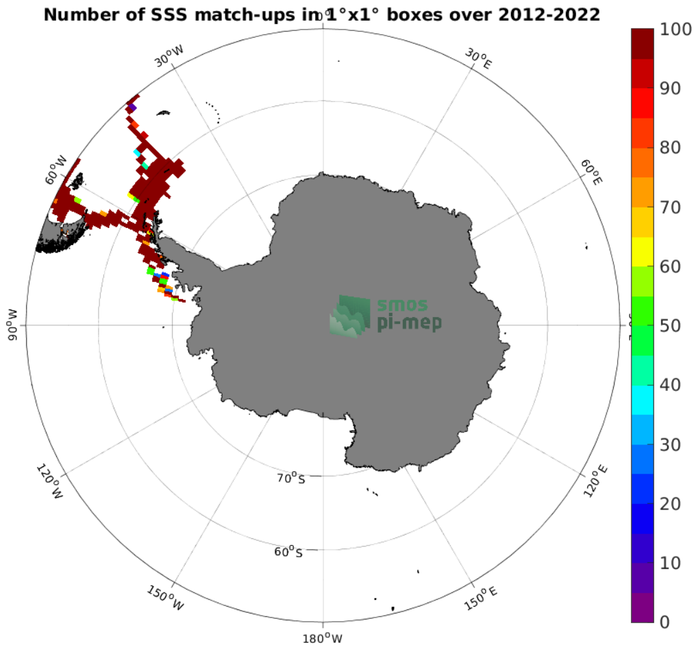
Figure 4: Number of SSS match-ups between TSG (CSIC-UTM) SSS and the SMOS SSS L4 OI v342 - Weekly (CMEMS-CATDS-LOPS) SSS product for the Southern Ocean Pi-MEP region over 1^\circ \times 1^\circ boxes and for the full satellite product period.
