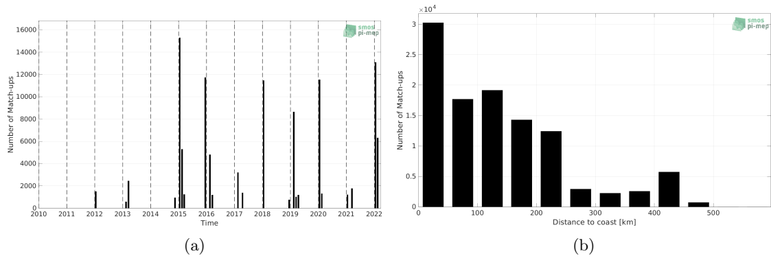
Figure 1: Number of match-ups between TSG (CSIC-UTM) and SMOS SSS L4 OI v342 - Weekly (CMEMS-CATDS-LOPS) SSS as a function of time (a) and as function of the distance to coast (b) over the Southern Ocean Pi-MEP region and for the full satellite product period.
