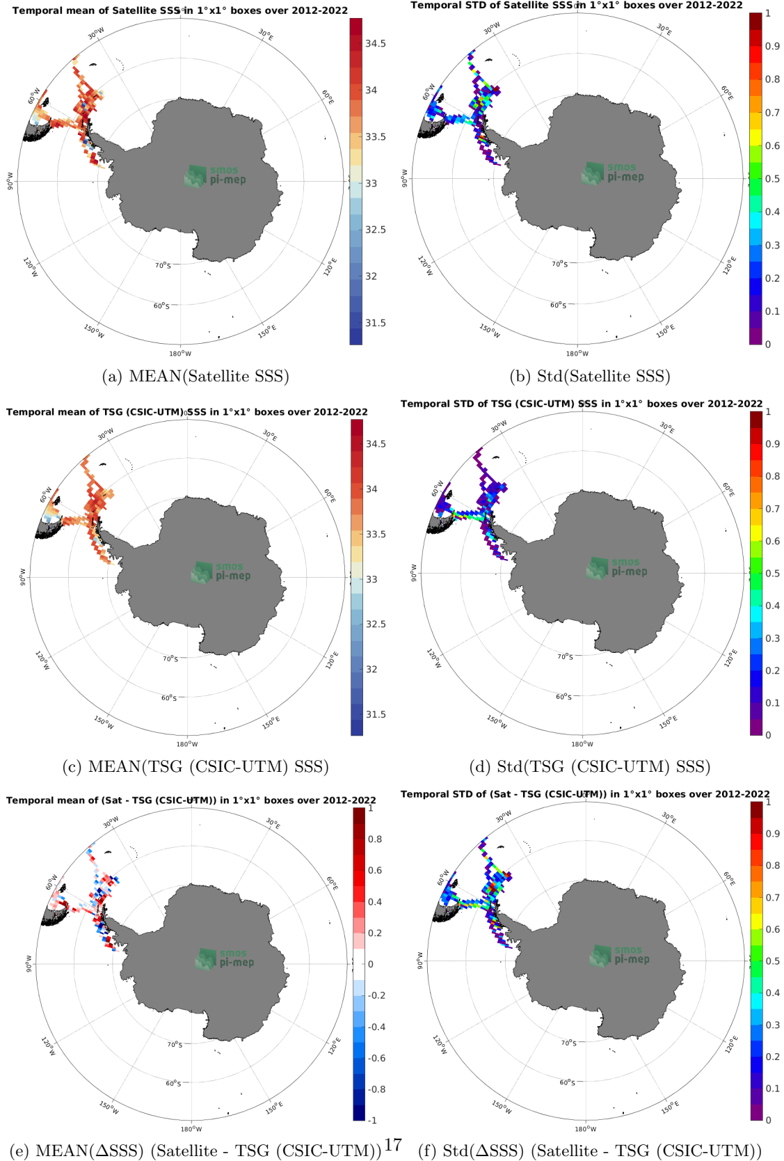
Figure 6: Temporal mean (left) and Std (right) of SSS from SMOS SSS L4 OI v342 - Weekly (CMEMS-CATDS-LOPS) (top), TSG (CSIC-UTM) (middle), and of \Delta SSS (Satellite - TSG (CSIC-UTM)). Only match-up pairs are used to generate these maps.
