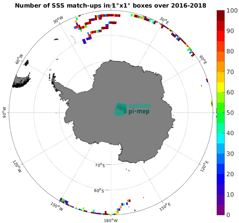
Figure 3: Number of SSS match-ups between Surface drifters SSS and the SMOS SSS L4 OI v342 - Weekly (CMEMS-CATDS-LOPS) SSS product for the Southern Ocean Pi-MEP region over 1^{\circ} \times 1^{\circ} boxes and for the full satellite product period.
