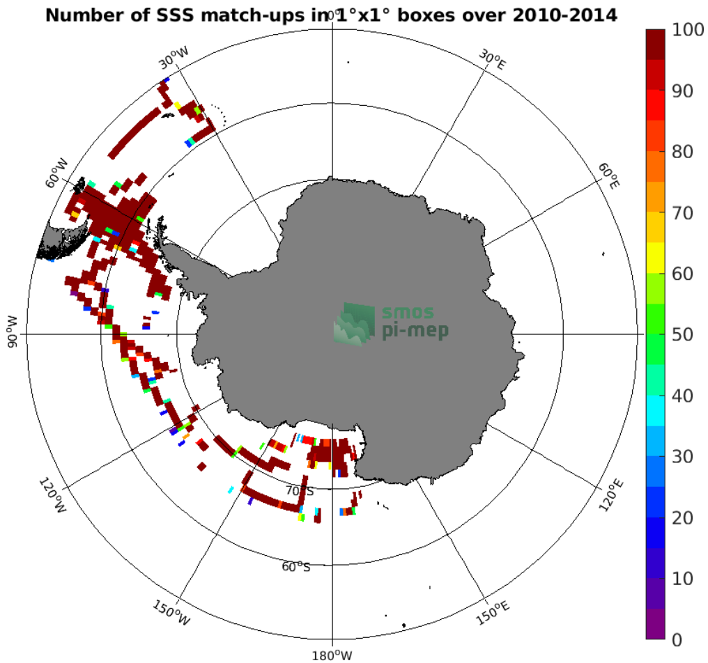
Figure 4: Number of SSS match-ups between TSG (SAMOS) SSS and the SMOS L4 v2 Weekly (CATDS-CECOS-IFREMER) SSS product for the Southern Ocean Pi-MEP region over 1^\circ \times 1^\circ boxes and for the full satellite product period.
