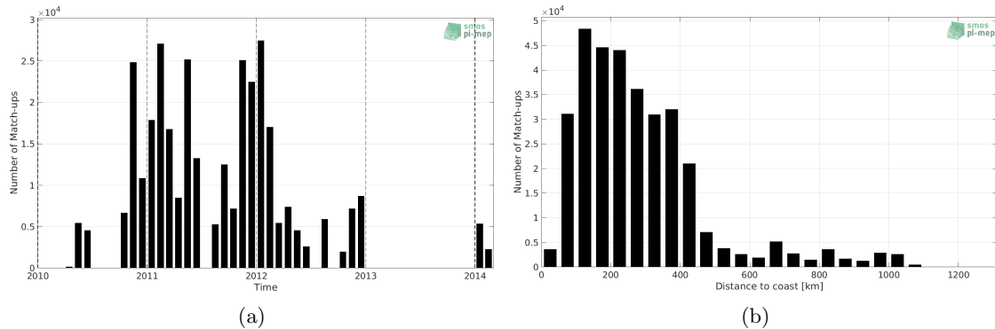
Figure 1: Number of match-ups between TSG (SAMOS) and SMOS L4 v2 Weekly (CATDS-CECOS-IFREMER) SSS as a function of time (a) and as function of the distance to coast (b) over the Southern Ocean Pi-MEP region and for the full satellite product period.
