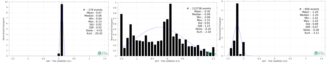
(a) RR=0 mm/h, 3 < U_{10} < 12 m/s, SST > 5^{\circ}\text{C} , distance to coast > 800 km (b) RR=0 mm/h, 3 < U_{10} < 12 m/s (c) RR > 1\text{mm/h} and U_{10} < 4\text{m/s}
