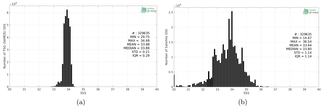
Figure 2: Histograms of SSS from TSG (SAMOS) (a) and SMOS L4 v2 Weekly (CATDS-CECOS-IFREMER) (b) considering all match-up pairs per bins of 0.1 over the Southern Ocean Pi-MEP region and for the full satellite product period.
