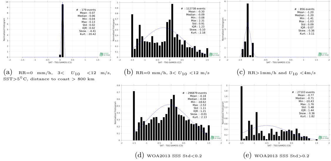
Figure 13: Normalized histogram of \Delta SSS (SMOS-L4-CATDS-CECOS-IFREMER-V2-WEEKLY-0.5DEG - TSG-SAMOS) for 5 different subdatasets corresponding to: RR=0 mm/h, 3 < U_{10} < 12 m/s, SST>5°C, distance to coast > 800 km (a), RR=0 mm/h, 3 < U_{10} < 12 m/s (b), RR>1mm/h and U_{10} < 4 m/s (c), WOA2013 SSS Std<0.2 (d), WOA2013 SSS Std>0.2 (e).
