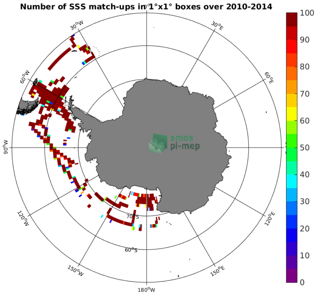
Figure 4: Number of SSS match-ups between TSG-SAMOS SSS and the SMOS-L4-CATDS-CECOS-IFREMER-V2-WEEKLY-0.5DEG SSS product for the Southern Ocean Pi-MEP region over 1°x1° boxes and for the full satellite product period.
