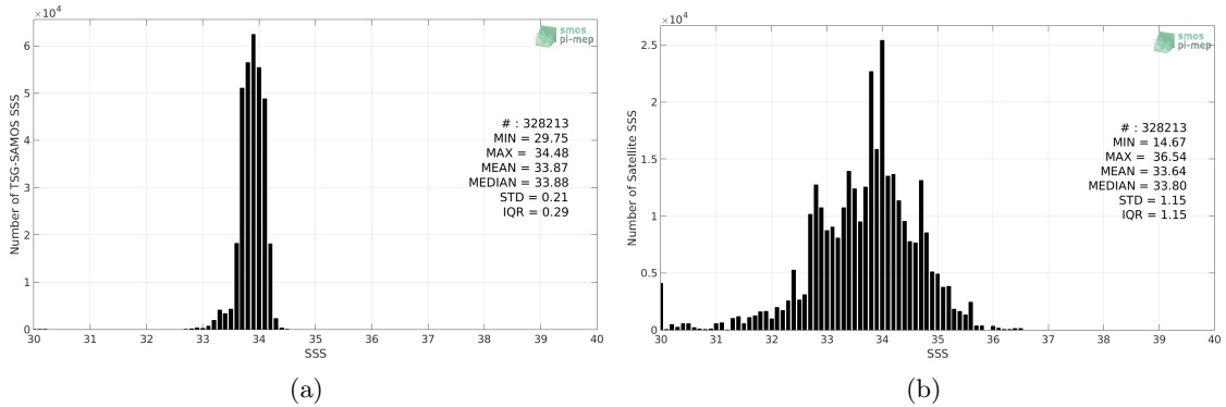
Figure 2: Histograms of SSS from TSG-SAMOS (a) and SMOS-L4-CATDS-CECOS-IFREMER-V2-WEEKLY-0.5DEG (b) considering all match-up pairs per bins of 0.1 over the Southern Ocean Pi-MEP region and for the full satellite product period.
