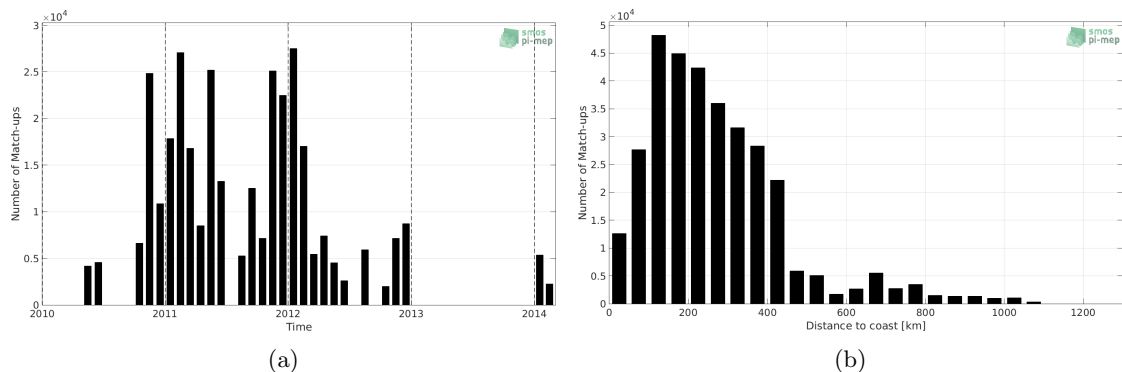
Figure 1: Number of match-ups between TSG-SAMOS and SMOS-L4-CATDS-CECOS-IFREMER-V2-WEEKLY-0.5DEG SSS as a function of time (a) and as function of the distance to coast (b) over the Southern Ocean Pi-MEP region and for the full satellite product period.
