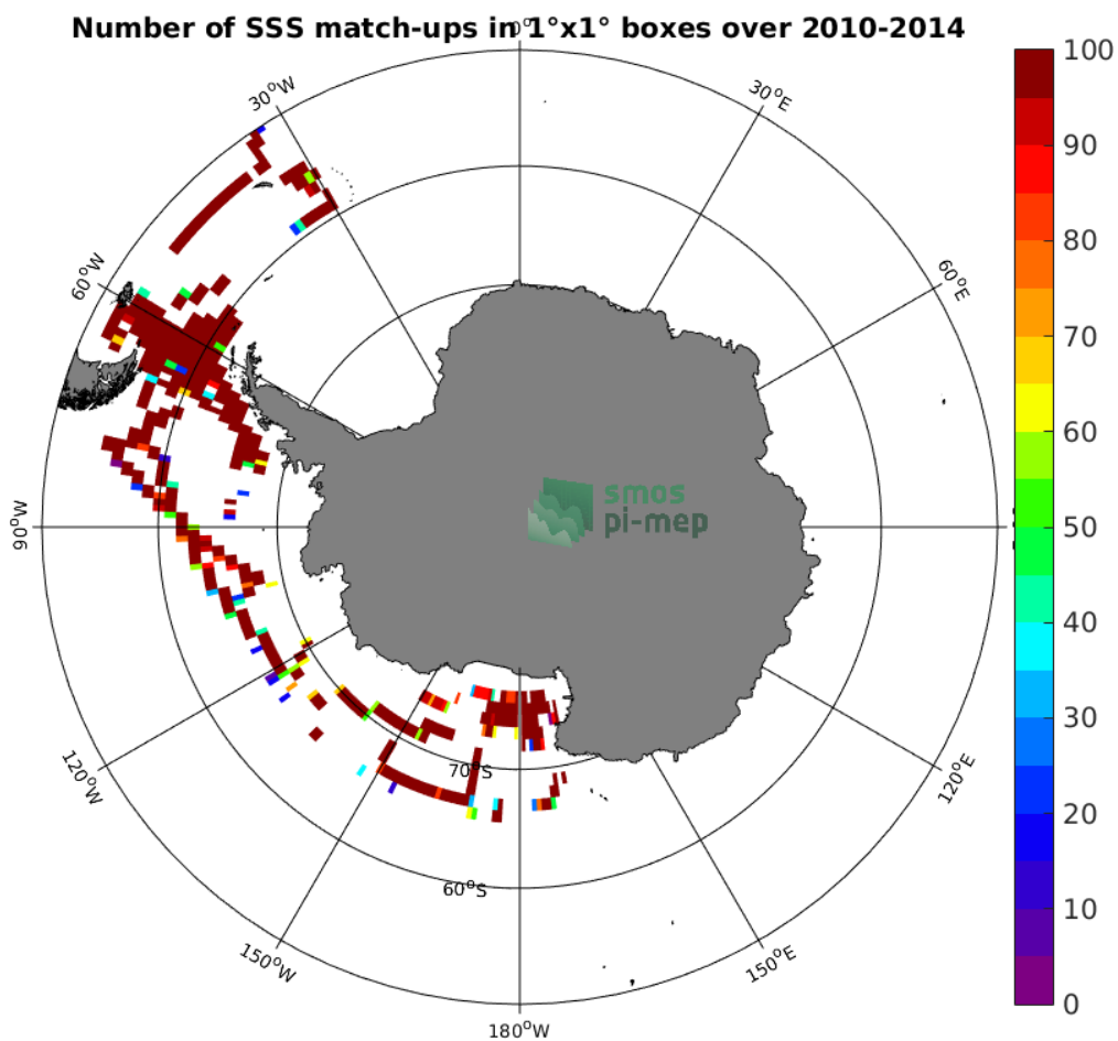
Figure 4: Number of SSS match-ups between TSG-SAMOS SSS and the SMOS-L4-CATDS-CECOS-IFREMER-V2-WEEKLY-0.5DEG SSS product for the Southern Ocean Pi-MEP region over 1^\circ \times 1^\circ boxes and for the full satellite product period.
