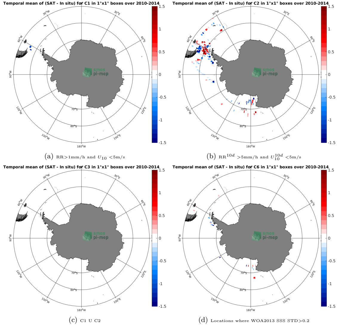
Figure 12: Temporal mean gridded over spatial boxes of size 1^\circ \times 1^\circ of \Delta SSS (SMOS-L4-CATDS-CECOS-IFREMER-V2-WEEKLY-0.5DEG - TSG-SAMOS) for 4 different subdatasets corresponding to: RR > 1\text{mm/h} and U_{10} < 5\text{m/s} (a), RR^{10d} > 5\text{mm/h} and U_{10}^{10d} < 5\text{m/s} (b), C1 U C2 (c), Locations where WOA2013 SSS STD > 0.2 (d).
