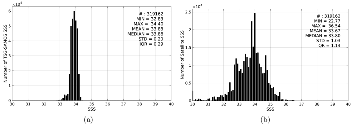
Figure 2: Histograms of SSS from TSG-SAMOS (a) and SMOS-L4-CATDS-CECOS-IFREMER-V2-WEEKLY-0.5DEG (b) considering all match-up pairs per bins of 0.1 over the Southern Ocean Pi-MEP region and for the full satellite product period.
