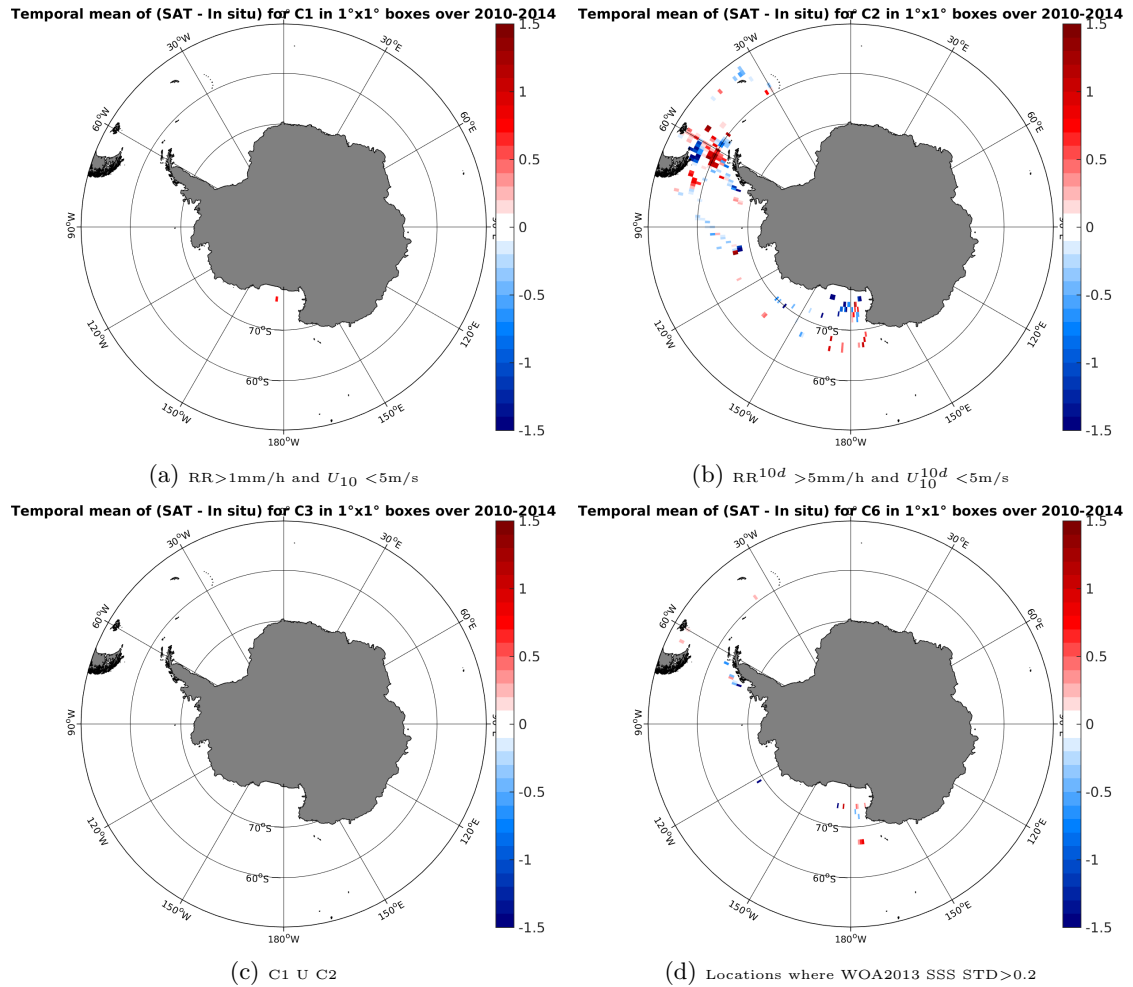
Figure 12: Temporal mean gridded over spatial boxes of size 1°x1° of \Delta SSS (SMOS-L4-CATDS-CECOS-IFREMER-V2-WEEKLY-0.5DEG - TSG-SAMOS) for 4 different subdatasets corresponding to: RR > 1\text{mm/h} and U_{10} < 5\text{m/s} (a), RR^{10d} > 5\text{mm/h} and U_{10}^{10d} < 5\text{m/s} (b), C1 U C2 (c), Locations where WOA2013 SSS STD > 0.2 (d).
