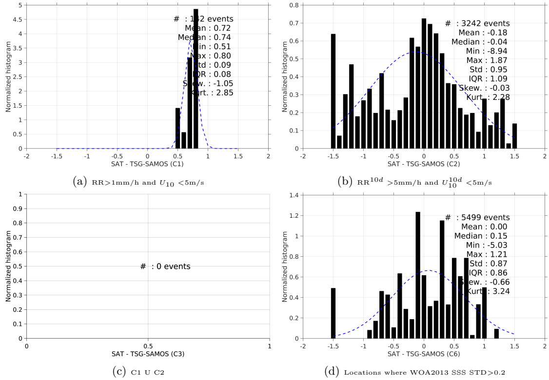
Figure 13: Normalized histogram of \Delta\text{SSS} (SMOS-L4-CATDS-CECOS-IFREMER-V2-WEEKLY-0.5DEG - TSG-SAMOS) for 6 different subdatasets corresponding to: RR>1mm/h and U_{10} < 5\text{m/s} (a), \text{RR}^{10d} > 5\text{mm/h} and U_{10}^{10d} < 5\text{m/s} (b), C1 U C2 (c), Locations where WOA2013 SSS STD>0.2 (d).
