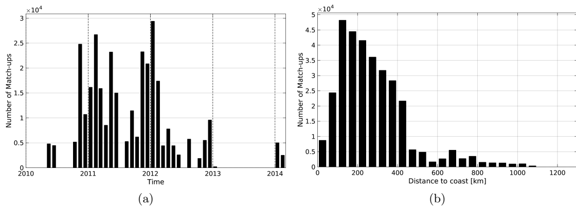
Figure 1: Number of match-ups between TSG-SAMOS and SMOS-L4-CATDS-CECOS-IFREMER-V2-WEEKLY-0.5DEG SSS as a function of time (a) and as function of the distance to coast (b) over the Southern Ocean Pi-MEP region and for the full satellite product period.
