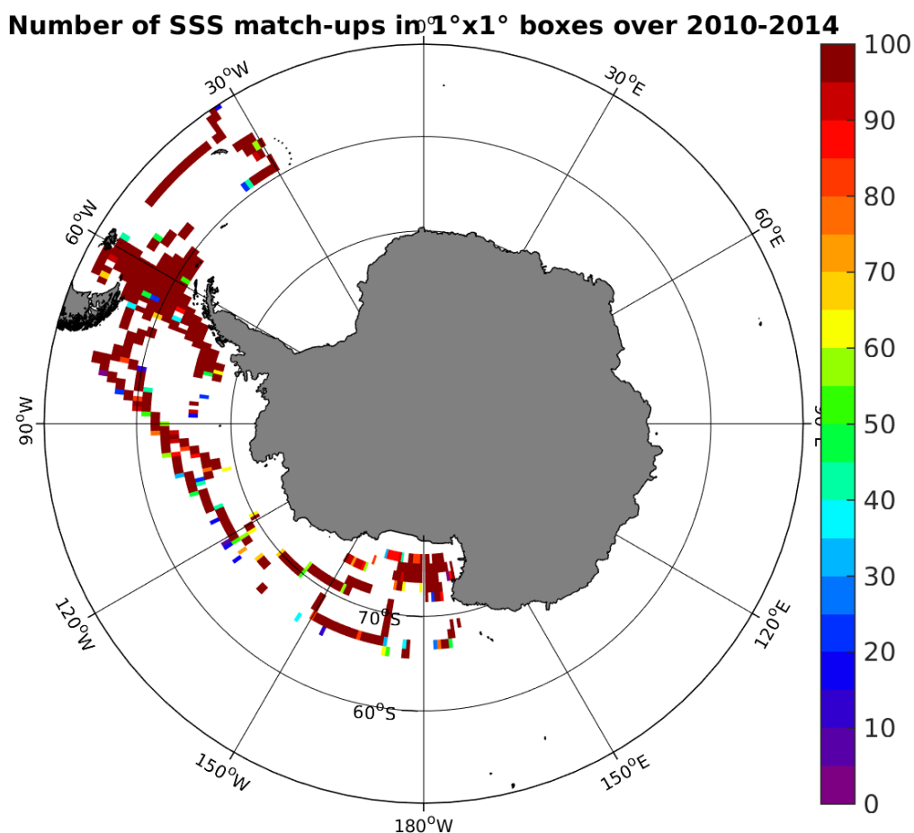
Figure 4: Number of SSS match-ups between TSG-SAMOS SSS and the SMOS-L4-CATDS-CECOS-IFREMER-V2-WEEKLY-0.5DEG SSS product for the Southern Ocean Pi-MEP region over 1°x1° boxes and for the full satellite product period.
