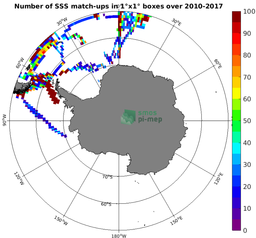
Figure 4: Number of SSS match-ups between TSG (Polarstern) SSS and the SMOS L4 v2 Weekly (CATDS-CECOS-IFREMER) SSS product for the Southern Ocean Pi-MEP region over 1°x1° boxes and for the full satellite product period.
