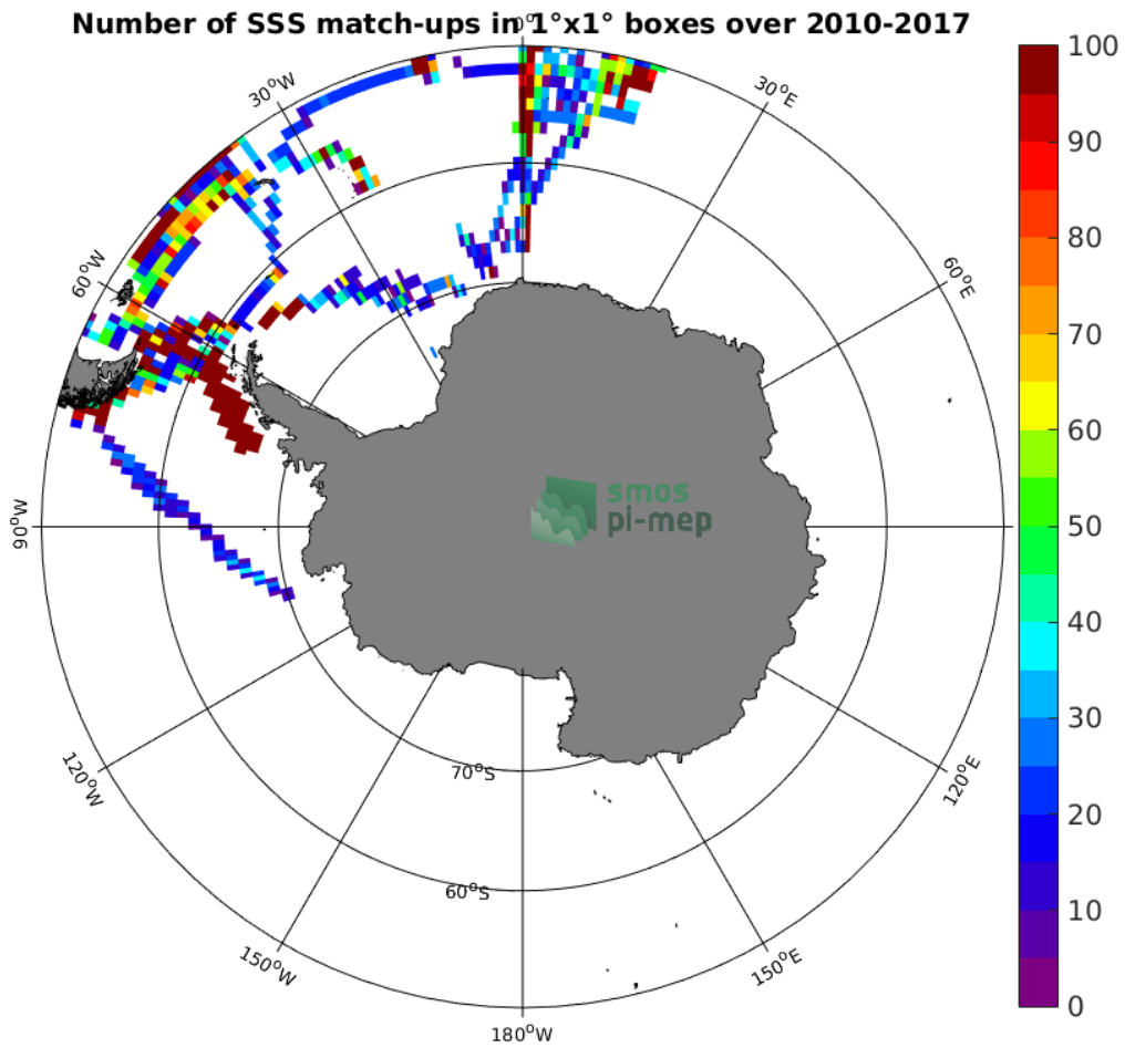
Figure 4: Number of SSS match-ups between TSG-POLARSTERN SSS and the SMOS-L4-CATDS-CECOS-IFREMER-V2-WEEKLY-0.5DEG SSS product for the Southern Ocean Pi-MEP region over 1°x1° boxes and for the full satellite product period.
