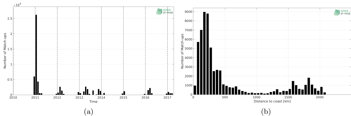
Figure 1: Number of match-ups between TSG-POLARSTERN and SMOS-L4-CATDS-CECOS-IFREMER-V2-WEEKLY-0.5DEG SSS as a function of time (a) and as function of the distance to coast (b) over the Southern Ocean Pi-MEP region and for the full satellite product period.
