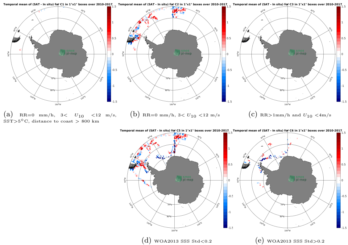
Figure 12: Temporal mean gridded over spatial boxes of size 1^{\circ}\times 1^{\circ} of \Delta\text{SSS} (SMOS-L4-CATDS-CECOS-IFREMER-V2-WEEKLY-0.5DEG - TSG-POLARSTERN) for 5 different subdatasets corresponding to:RR=0 mm/h, 3 < U_{10} < 12 m/s, SST > 5^{\circ}\text{C} , distance to coast > 800 km (a), RR=0 mm/h, 3 < U_{10} < 12 m/s (b), RR > 1 mm/h and U_{10} < 4 m/s (c), WOA2013 SSS Std < 0.2 (d), WOA2013 SSS Std > 0.2 (e).
