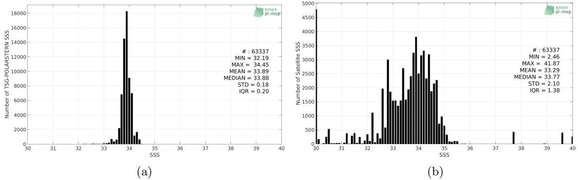
Figure 2: Histograms of SSS from TSG-POLARSTERN (a) and SMOS-L4-CATDS-CECOS-IFREMER-V2-WEEKLY-0.5DEG (b) considering all match-up pairs per bins of 0.1 over the Southern Ocean Pi-MEP region and for the full satellite product period.
