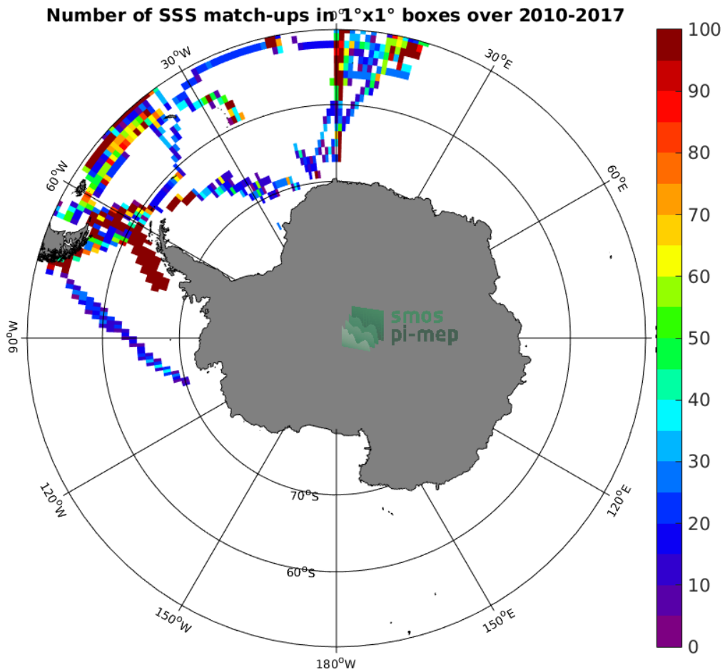
Figure 4: Number of SSS match-ups between TSG-POLARSTERN SSS and the SMOS-L4-CATDS-CECOS-IFREMER-V2-WEEKLY-0.5DEG SSS product for the Southern Ocean Pi-MEP region over 1^\circ \times 1^\circ boxes and for the full satellite product period.
