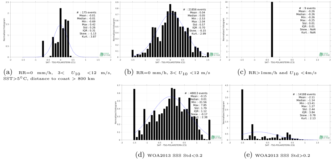
Figure 13: Normalized histogram of \Delta\text{SSS} (SMOS-L4-CATDS-CECOS-IFREMER-V2-WEEKLY-0.5DEG - TSG-POLARSTERN) for 5 different subdatasets corresponding to: RR=0 mm/h, 3 < U_{10} < 12 m/s, SST > 5^{\circ}\text{C} , distance to coast > 800 km (a), RR=0 mm/h, 3 < U_{10} < 12 m/s (b), RR > 1\text{mm/h} and U_{10} < 4\text{m/s} (c), WOA2013 SSS Std < 0.2 (d), WOA2013 SSS Std > 0.2 (e).
