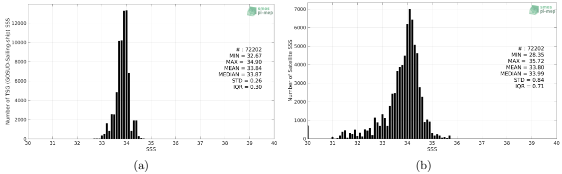
Figure 2: Histograms of SSS from TSG (GOSUD-Sailing-ship) (a) and SMOS L4 v2 Weekly (CATDS-CECOS-IFREMER) (b) considering all match-up pairs per bins of 0.1 over the Southern Ocean Pi-MEP region and for the full satellite product period.
