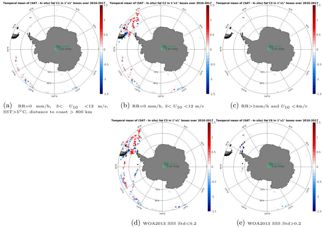
Figure 12: Temporal mean gridded over spatial boxes of size 1°x1° of \Delta SSS (SMOS L4 v2 Weekly (CATDS-CECOS-IFREMER) - TSG (GOSUD-Sailing-ship)) for 5 different subdatasets corresponding to:RR=0 mm/h, 3 < U_{10} < 12 m/s, SST>5°C, distance to coast > 800 km (a), RR=0 mm/h, 3 < U_{10} < 12 m/s (b), RR>1mm/h and U_{10} < 4 m/s (c), WOA2013 SSS Std<0.2 (d), WOA2013 SSS Std>0.2 (e).
