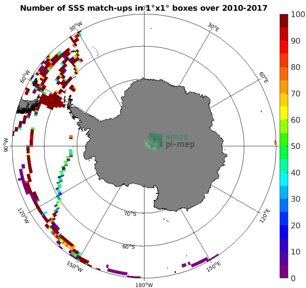
Figure 4: Number of SSS match-ups between TSG (GOSUD-Sailing-ship) SSS and the SMOS L4 v2 Weekly (CATDS-CECOS-IFREMER) SSS product for the Southern Ocean Pi-MEP region over 1^{\circ} \times 1^{\circ} boxes and for the full satellite product period.
