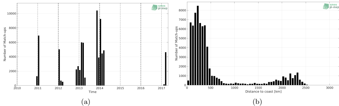
Figure 1: Number of match-ups between TSG (GOSUD-Sailing-ship) and SMOS L4 v2 Weekly (CATDS-CECOS-IFREMER) SSS as a function of time (a) and as function of the distance to coast (b) over the Southern Ocean Pi-MEP region and for the full satellite product period.
