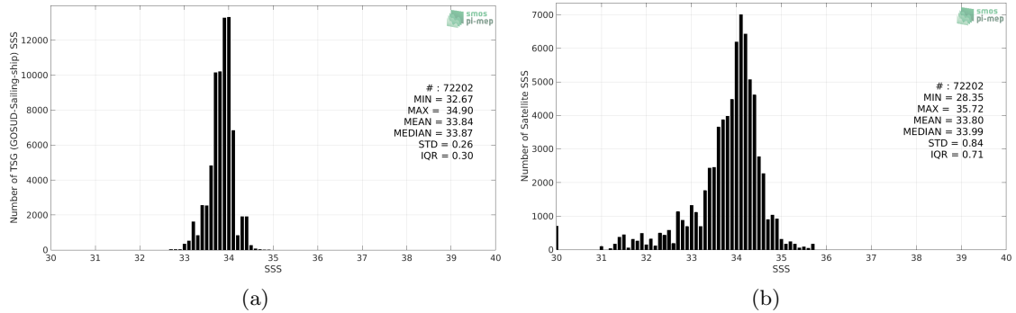
Figure 2: Histograms of SSS from TSG (GOSUD-Sailing-ship) (a) and SMOS L4 v2 Weekly (CATDS-CECOS-IFREMER) (b) considering all match-up pairs per bins of 0.1 over the Southern Ocean Pi-MEP region and for the full satellite product period.
