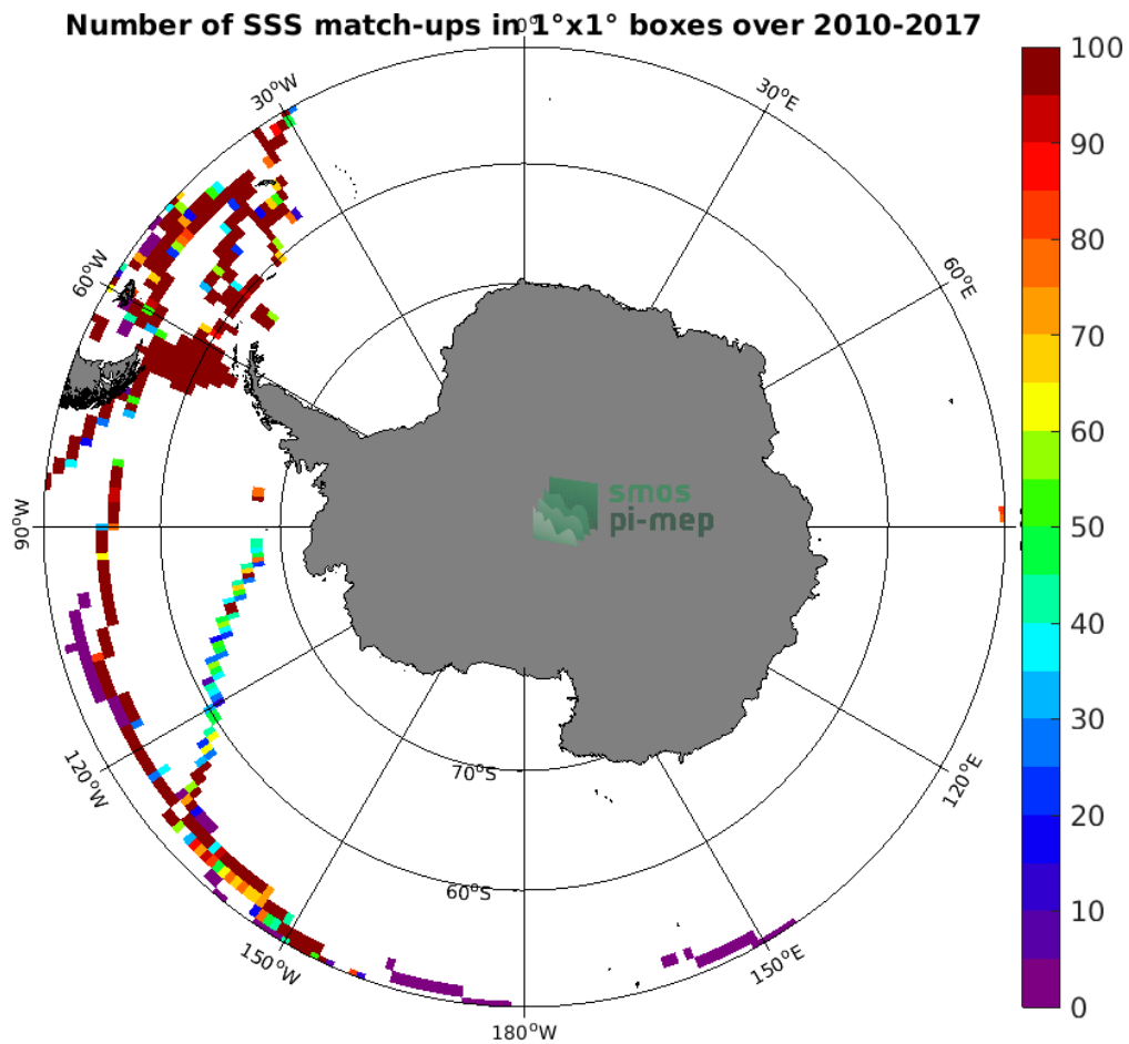
Figure 4: Number of SSS match-ups between TSG (GOSUD-Sailing-ship) SSS and the SMOS L4 v2 Weekly (CATDS-CECOS-IFREMER) SSS product for the Southern Ocean Pi-MEP region over 1°x1° boxes and for the full satellite product period.
