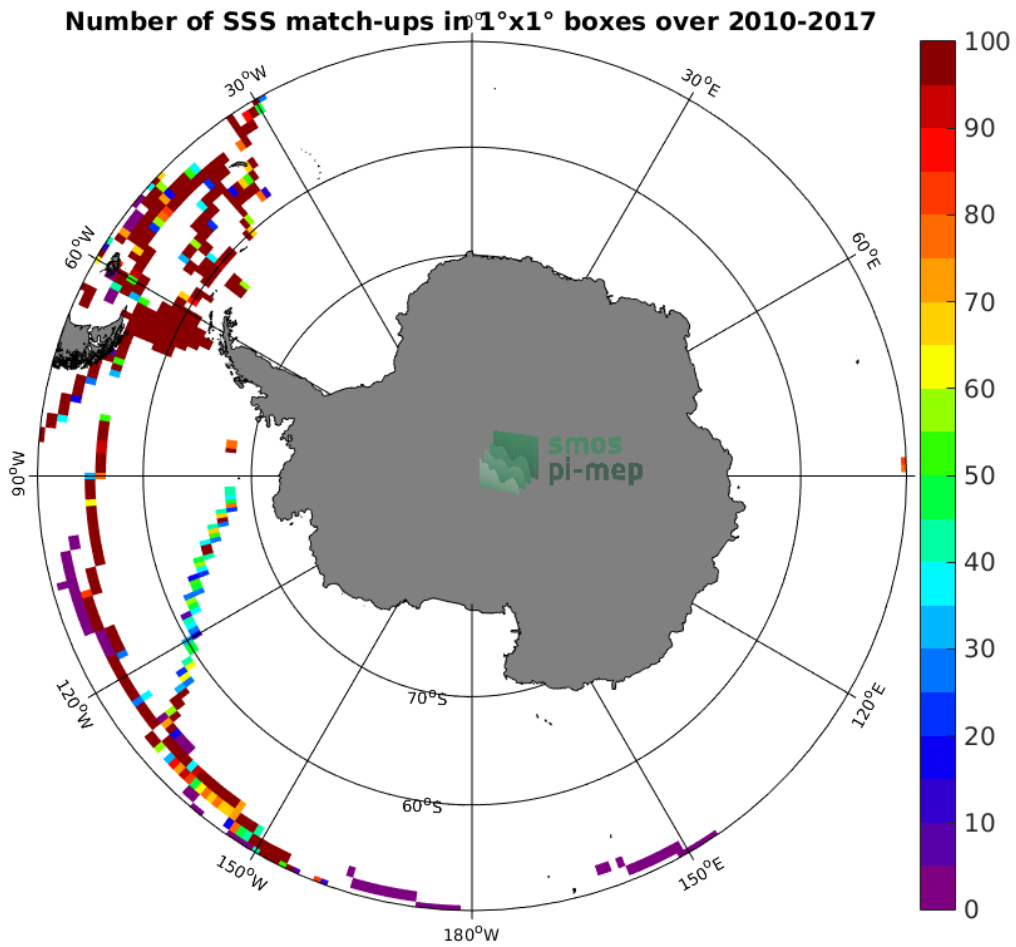
Figure 4: Number of SSS match-ups between TSG-GOSUD-Sailing-ship SSS and the SMOS-L4-CATDS-CECOS-IFREMER-V2-WEEKLY-0.5DEG SSS product for the Southern Ocean Pi-MEP region over 1°x1° boxes and for the full satellite product period.
