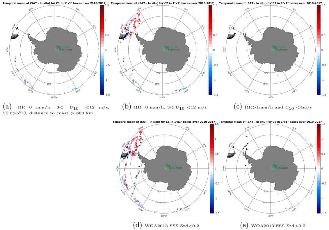
Figure 12: Temporal mean gridded over spatial boxes of size 1°x1° of \Delta SSS (SMOS-L4-CATDS-CECOS-IFREMER-V2-WEEKLY-0.5DEG - TSG-GOSUD-Sailing-ship) for 5 different subdatasets corresponding to:RR=0 mm/h, 3 < U_{10} < 12 m/s, SST>5°C, distance to coast > 800 km (a), RR=0 mm/h, 3 < U_{10} < 12 m/s (b), RR>1mm/h and U_{10} < 4 m/s (c), WOA2013 SSS Std<0.2 (d), WOA2013 SSS Std>0.2 (e).
