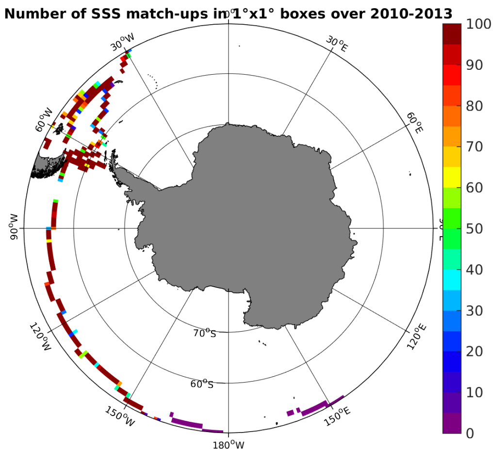
Figure 4: Number of SSS match-ups between TSG-GOSUD-Sailing-ship SSS and the SMOS-L4-CATDS-CECOS-IFREMER-V2-WEEKLY-0.5DEG SSS product for the Southern Ocean Pi-MEP region over 1°x1° boxes and for the full satellite product period.
