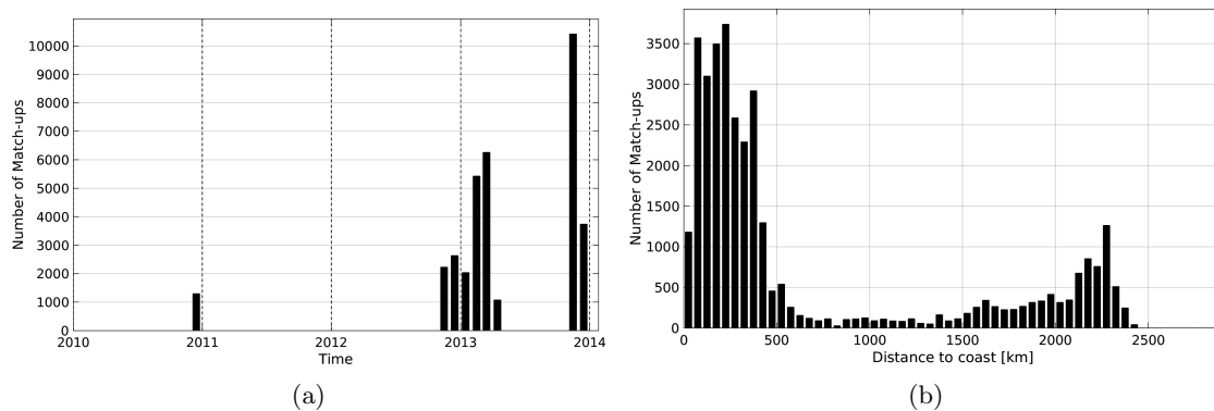
Figure 1: Number of match-ups between TSG-GOSUD-Sailing-ship and SMOS-L4-CATDS-CECOS-IFREMER-V2-WEEKLY-0.5DEG SSS as a function of time (a) and as function of the distance to coast (b) over the Southern Ocean Pi-MEP region and for the full satellite product period.
