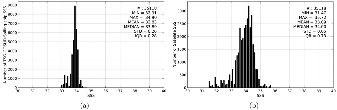
Figure 2: Histograms of SSS from TSG-GOSUD-Sailing-ship (a) and SMOS-L4-CATDS-CECOS-IFREMER-V2-WEEKLY-0.5DEG (b) considering all match-up pairs per bins of 0.1 over the Southern Ocean Pi-MEP region and for the full satellite product period.
